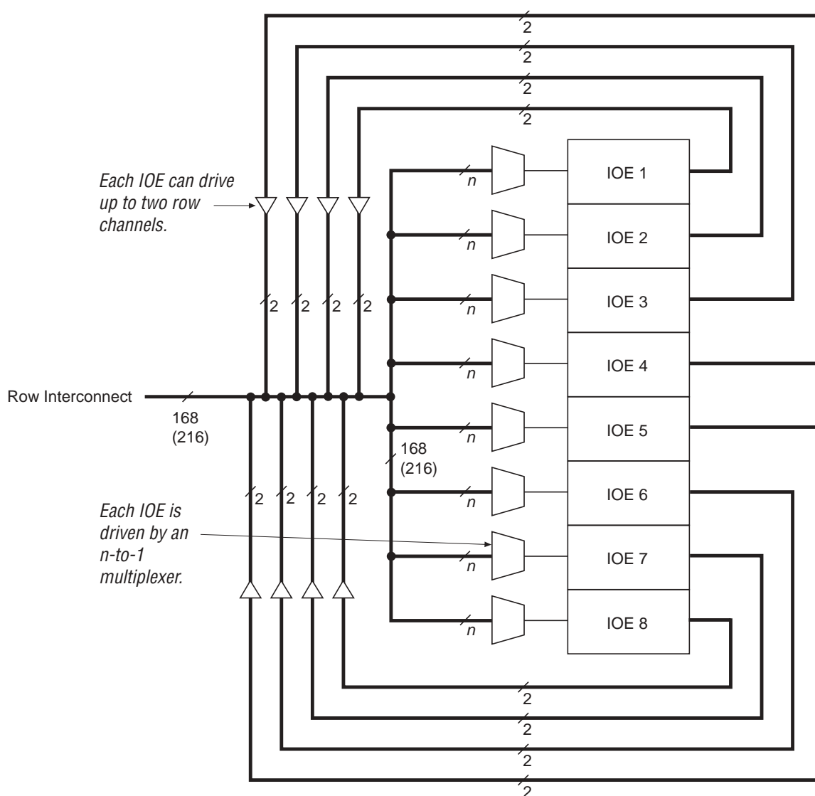
Figure 11. FLEX 8000 Row-to-IOE Connections
