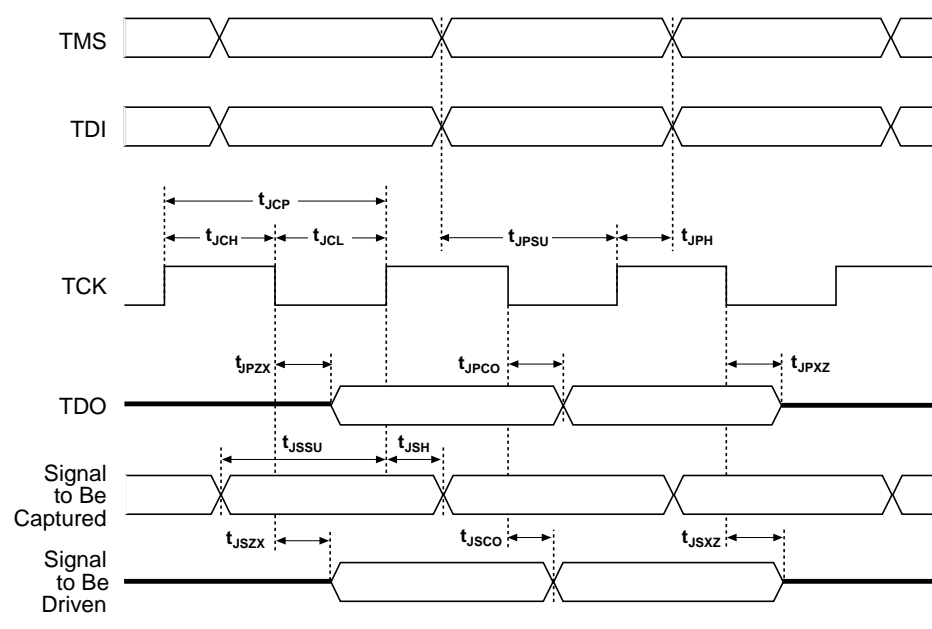
Figure 14. EPF8282A, EPF8282AV, EPF8636A, EPF8820A & EPF81500A JTAG Waveforms
