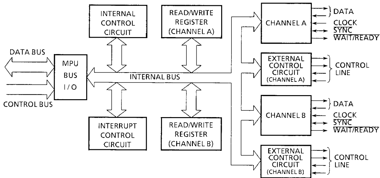
Figure 3.1 Block Diagram
