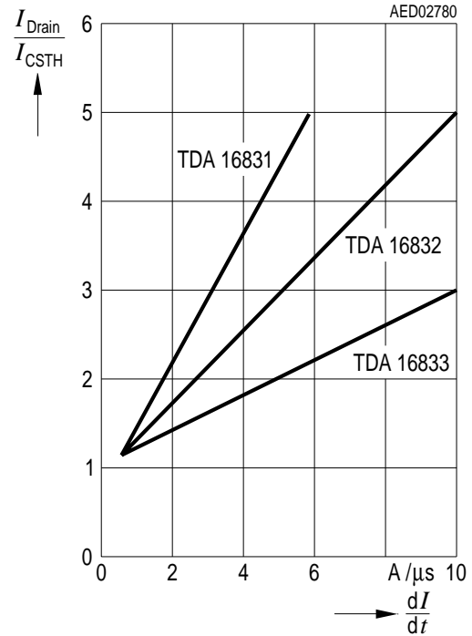
Normalized Overcurrent Shutdown versus Drain Current Slope
