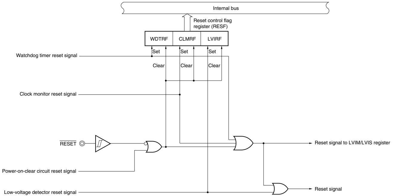
★Figure 20-1. Block Diagram of Reset Function
