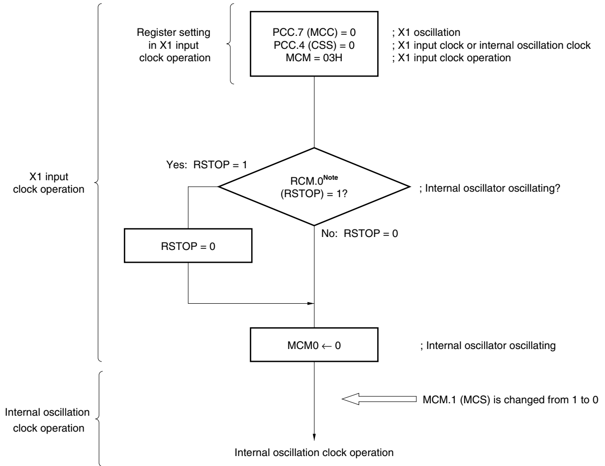
Figure 5-15. Switching from X1 Input Clock to Internal Oscillation Clock (Flowchart)
