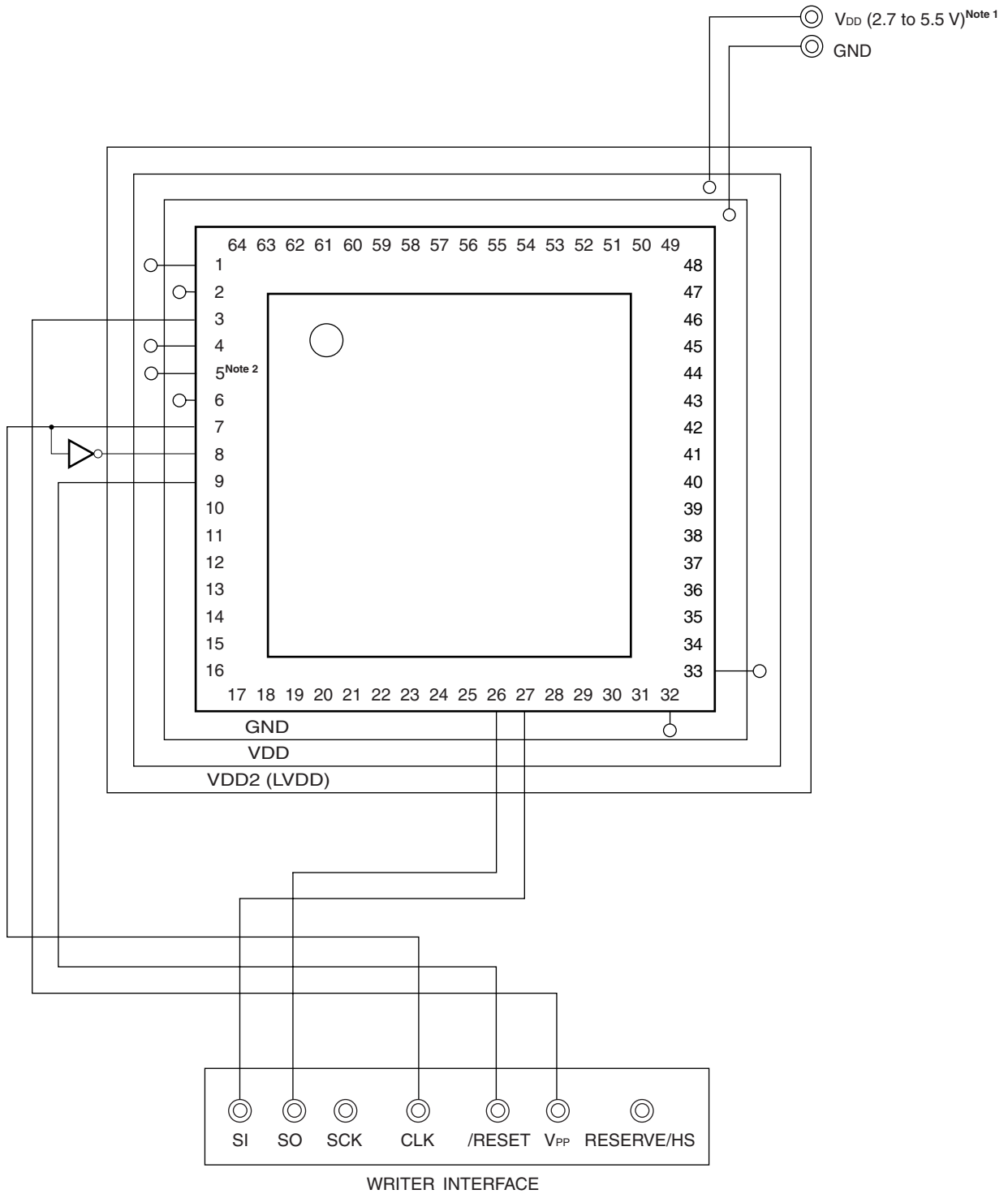
Figure 27-5. Example of Wiring Adapter for Flash Memory Writing in UART (UART0) Mode
