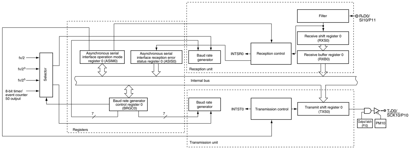
Figure 13-1. Block Diagram of Serial Interface UART0
