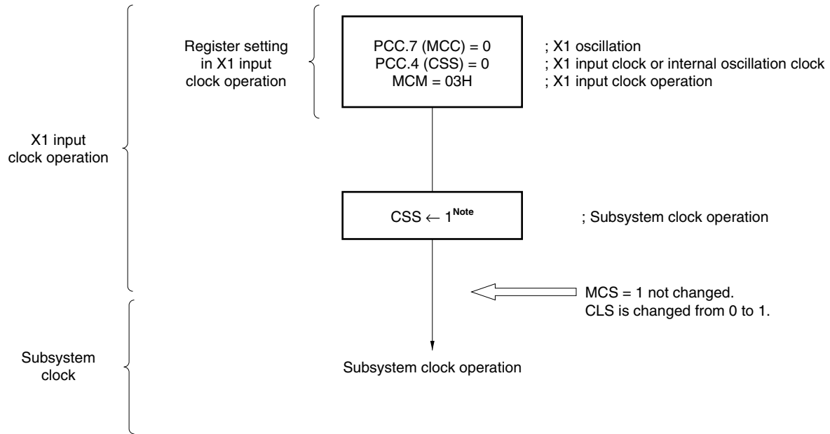
Figure 5-16. Switching from X1 Input Clock to Subsystem Clock (Flowchart)
