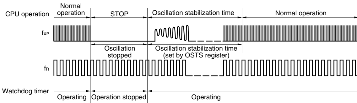
Figure 10-5. Operation in STOP Mode (CPU Clock: X1 Input Clock, WDT Operation Clock: Internal Oscillation Clock)
