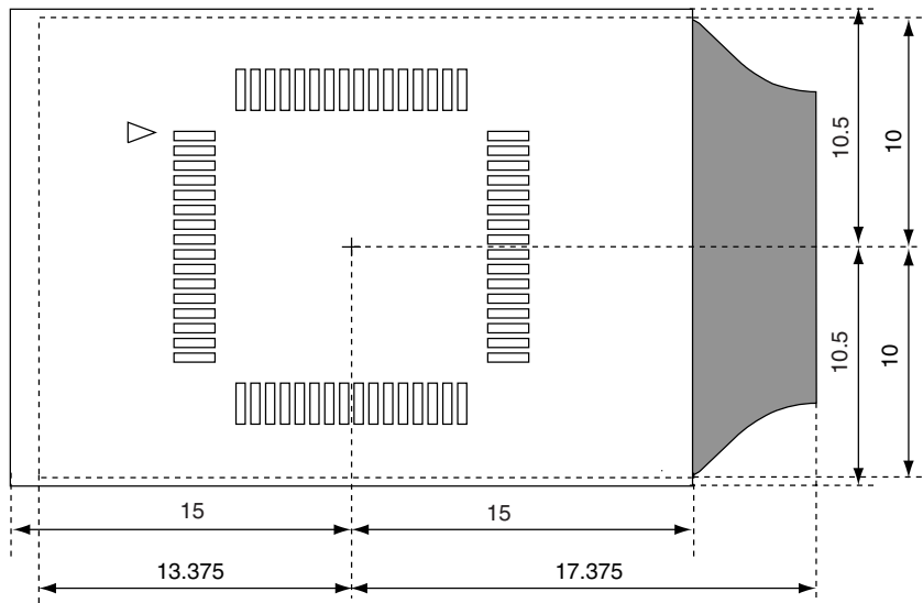
Figure B-9. Restricted Area on Target System (64-Pin GK Package)
