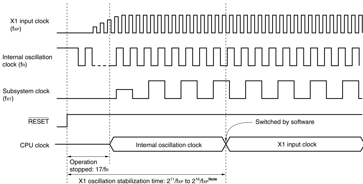
Figure 5-12. Timing Diagram of CPU Default Start Using Internal Oscillator
