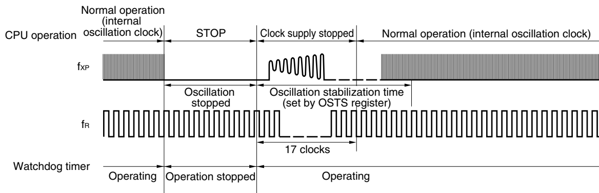
Figure 10-7. Operation in STOP Mode (CPU Clock and WDT Operation Clock: Internal Oscillation Clock)
