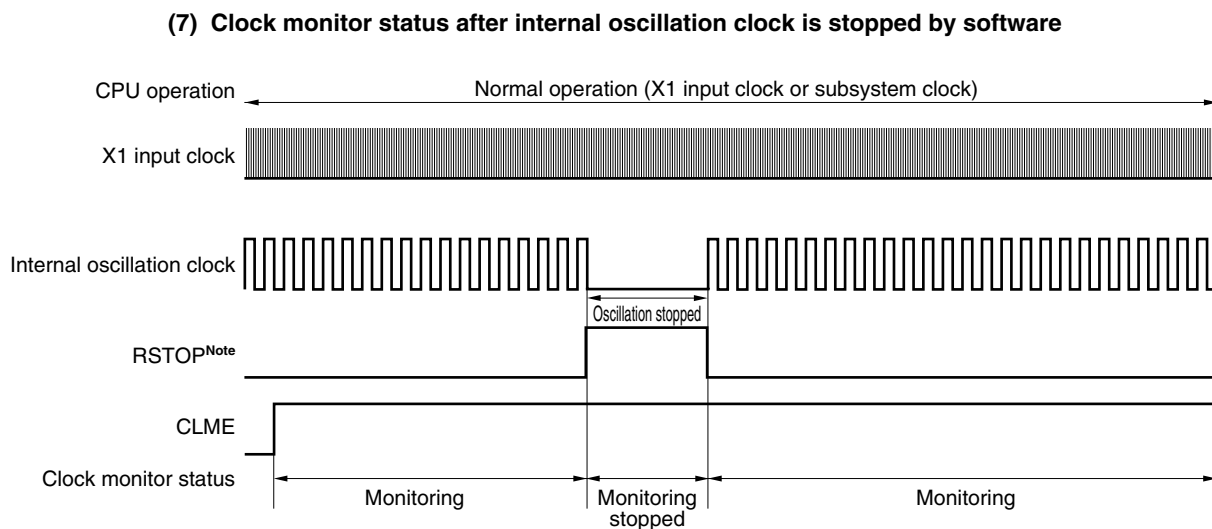
Figure 21-3. Timing of Clock Monitor (4/4)
