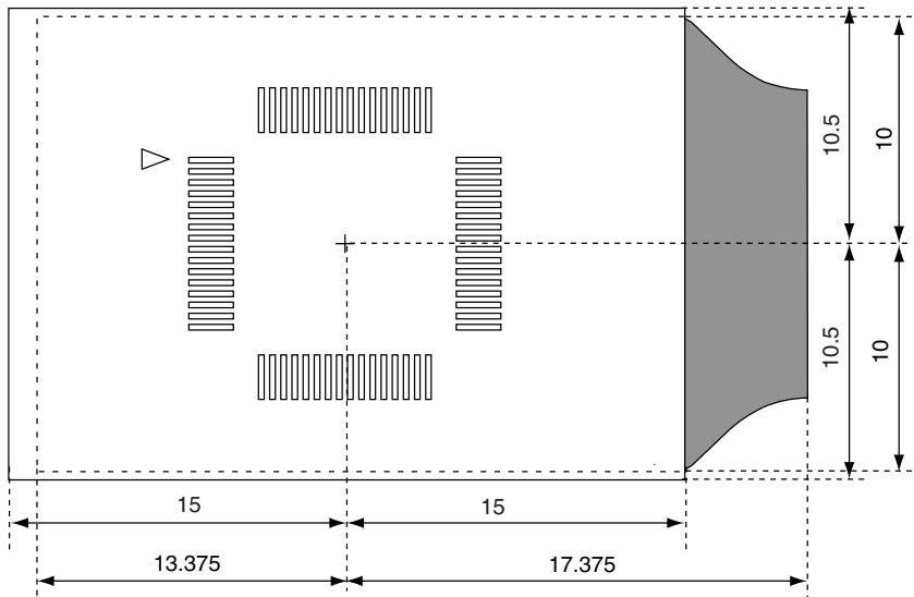
Figure B-8. Restricted Area on Target System (64-Pin GB Package)
