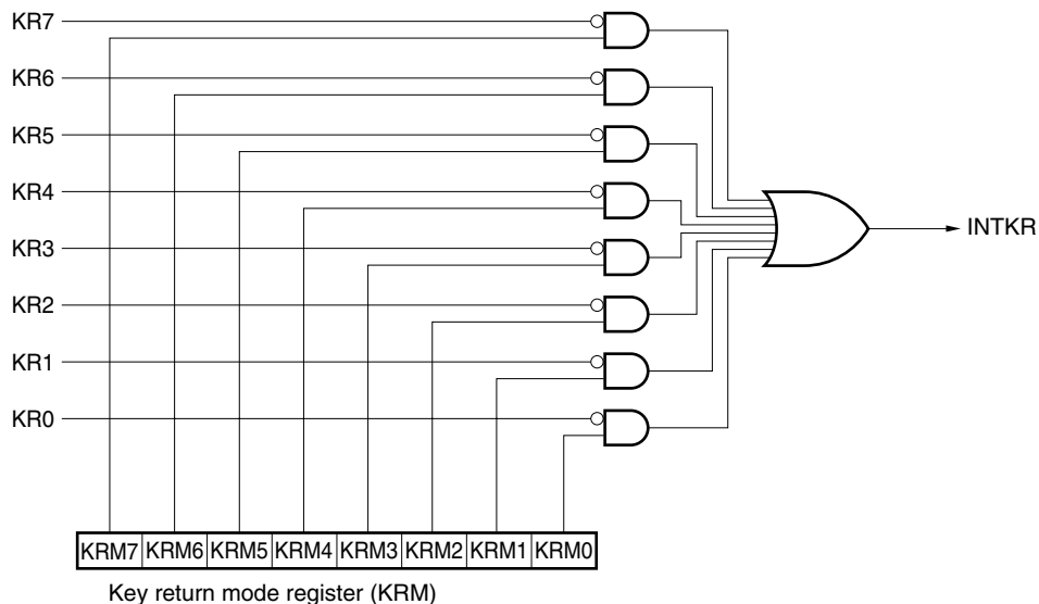
Figure 18-1. Block Diagram of Key Interrupt
