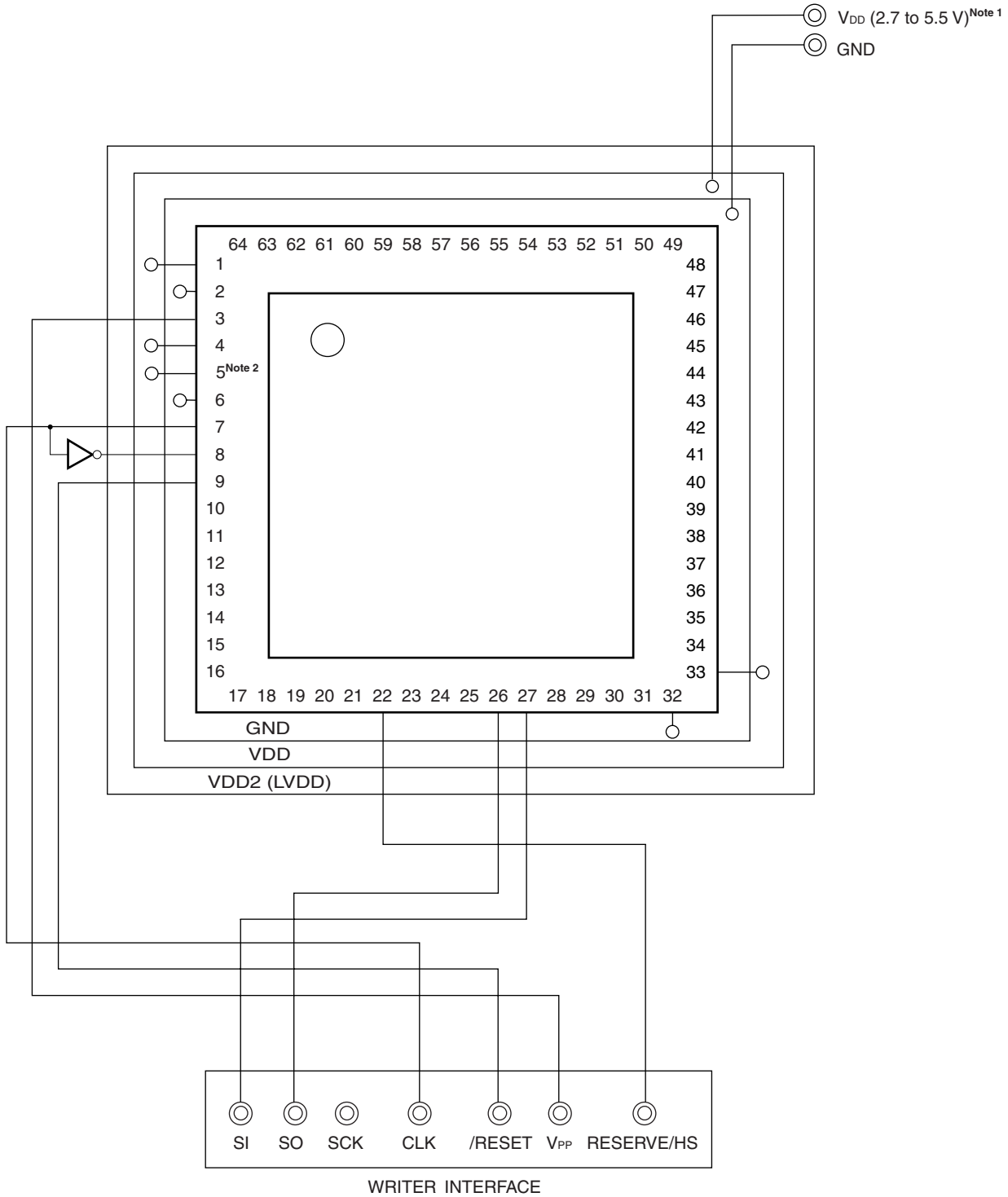
Figure 27-6. Example of Wiring Adapter for Flash Memory Writing in UART (UART0 + HS) Mode
