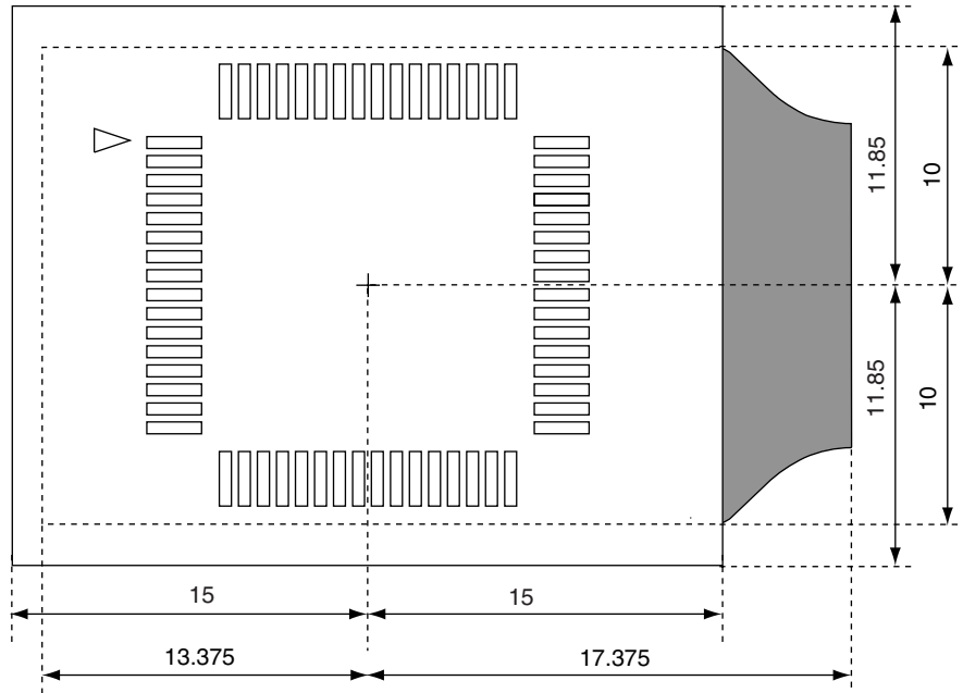
Figure B-10. Restricted Area on Target System (64-Pin GC Package)
