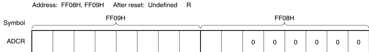
Figure 12-6. Format of A/D Conversion Result Register (ADCR)
