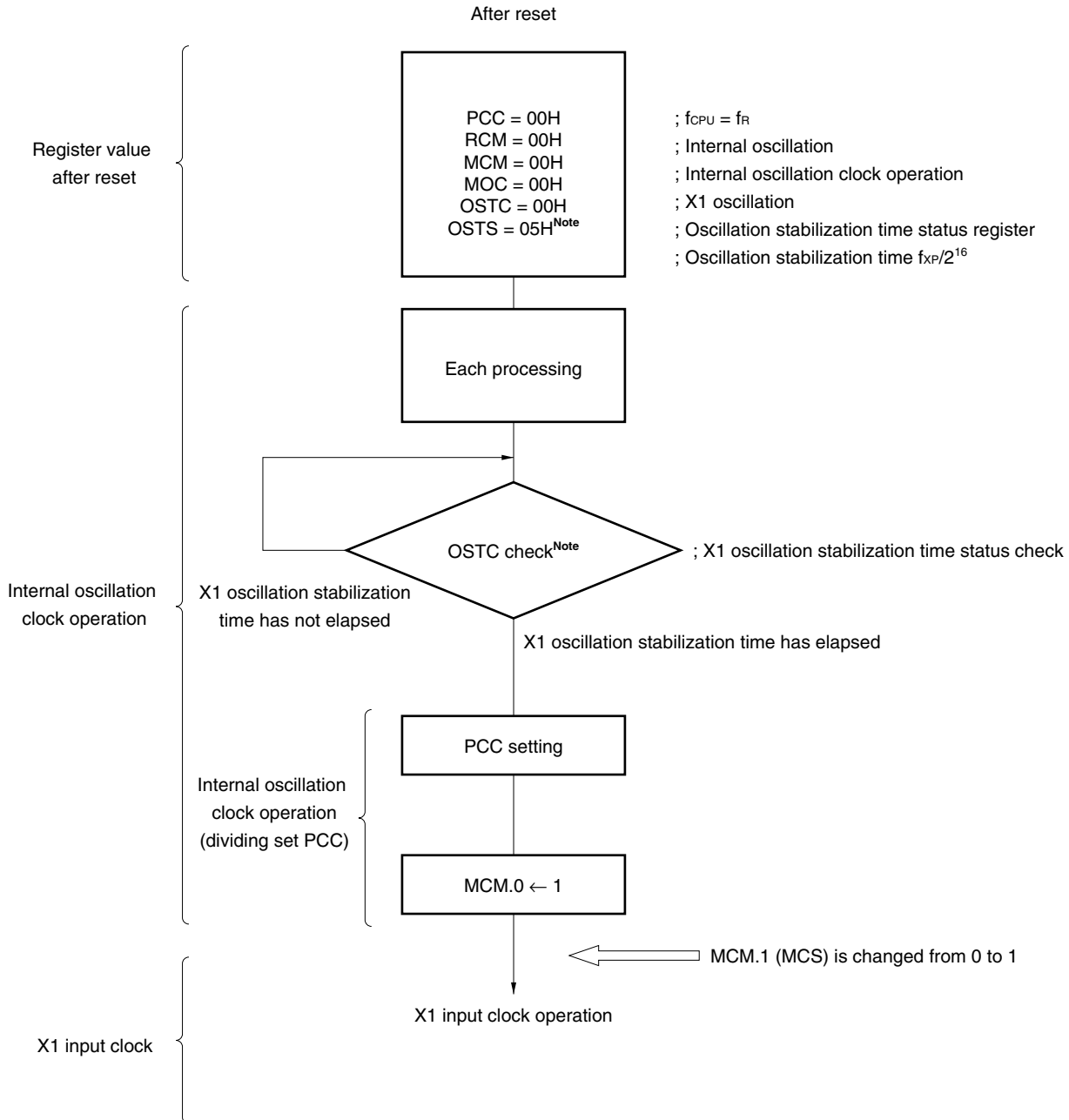
Figure 5-14. Switching from Internal Oscillation Clock to X1 Input Clock (Flowchart)
