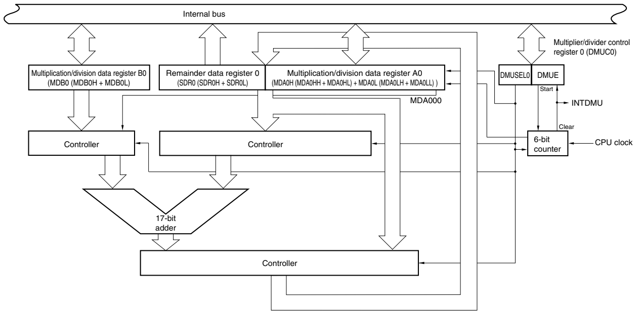
Figure 16-1. Block Diagram of Multiplier/Divider
