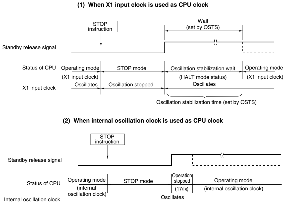
Figure 19-6. STOP Mode Release by Interrupt Request Generation
