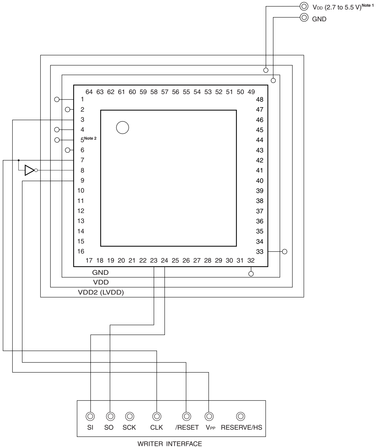
Figure 27-7. Example of Wiring Adapter for Flash Memory Writing in UART (UART6) Mode
