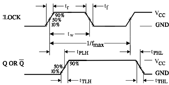
Figure 1. Switching Waveforms
