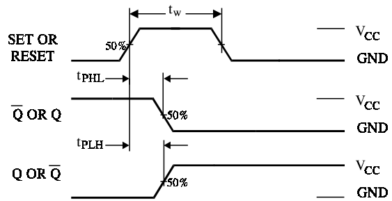
Figure 2. Switching Waveforms
