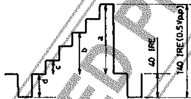
Note) : Linearity test waveform (2.4MHz) / (20kHz)
