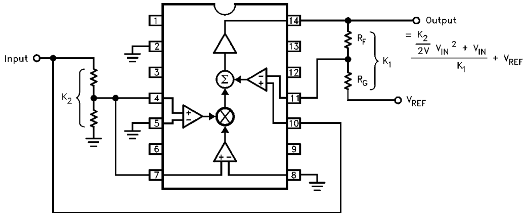
Figure 5. Polynomial Function Generator
