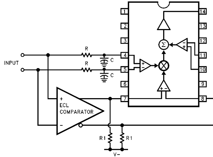
Figure 4. Absolute-Value Input Circuitry
