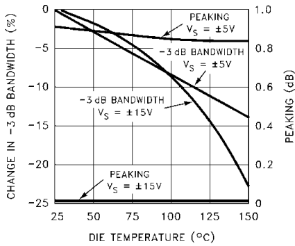
Change in Bandwidth and Peaking vs Temperature
