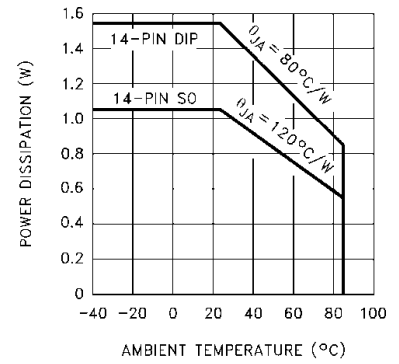
14-Pin Package Power Dissipation vs Ambient Temperature
