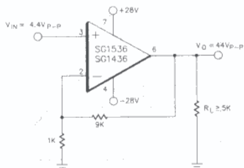
FIGURE 9 - TYPICAL NON-INVERTING X10 VOLTAGE AMPLIFIER
