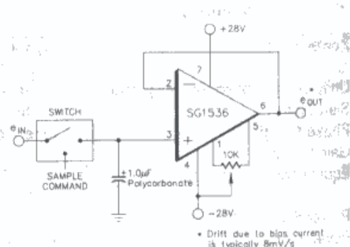
FIGURE 8 - LOW-DRIFT SAMPLE AND HOLD
