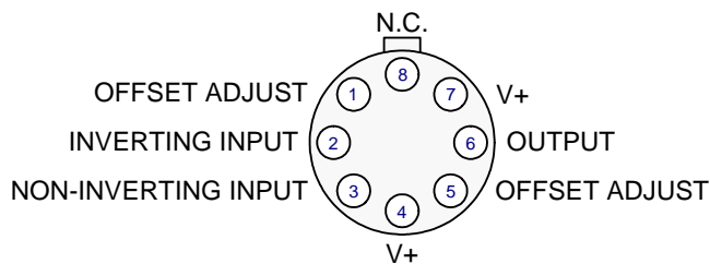
T PACKAGE
