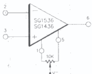
FIGURE 6 - VOLTAGE OFFSET NULL CIRCUIT
