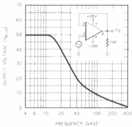
FIGURE 1. POWER BANDWIDTH
