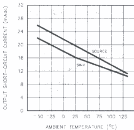
FIGURE 4. OUTPUT SHORT-CIRCUIT CURRENT VS. TEMPERATURE
