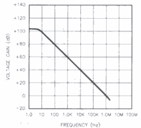
FIGURE 3. OPEN-LOOP FREQUENCY RESPONSE
