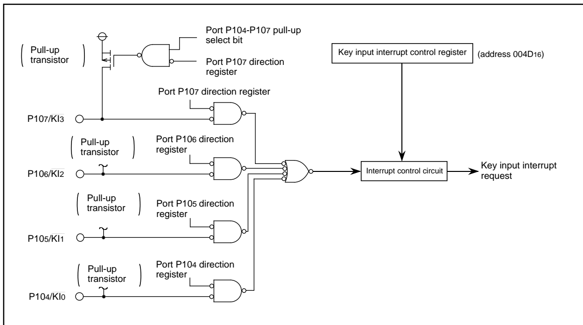
Figure 1.14.11. Block diagram of key input interrupt
