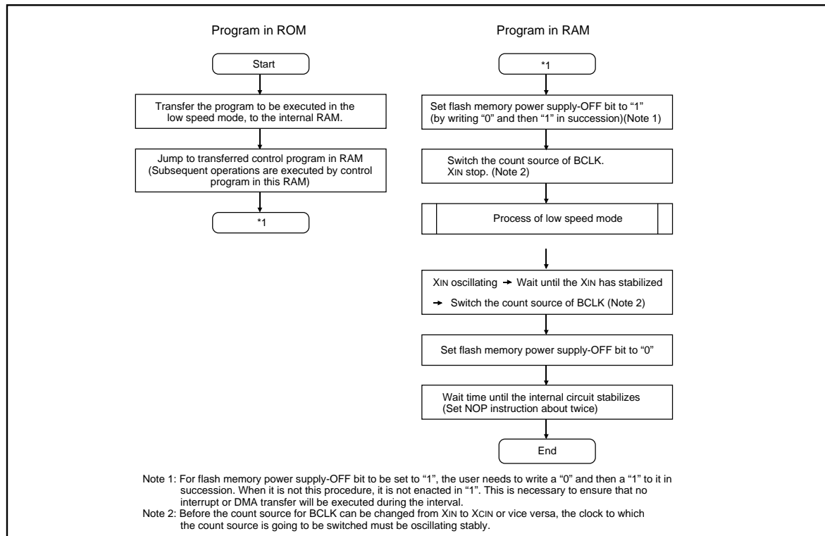
Figure 1.29.3. Shifting to The Low Speed Mode Flowchart
