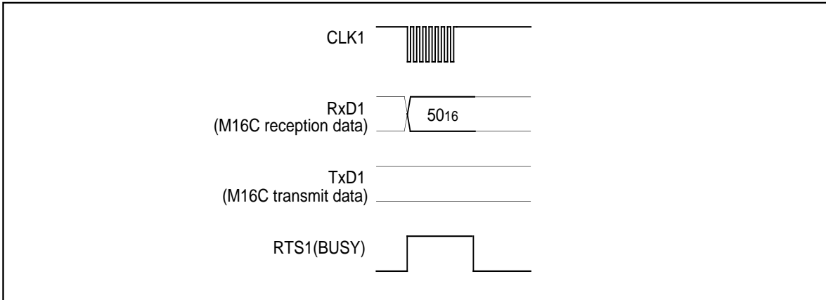
Figure 1.31.5. Timing for clearing the status register
