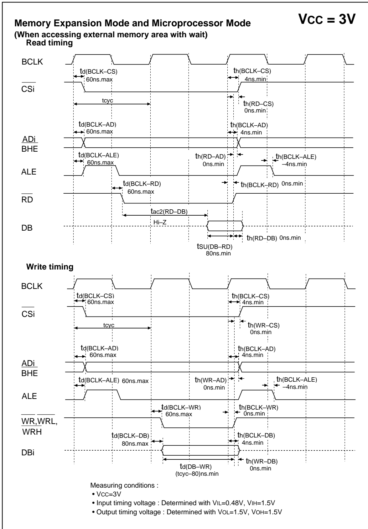
Figure 1.26.10. V_{CC}=3V timing diagram (4)
