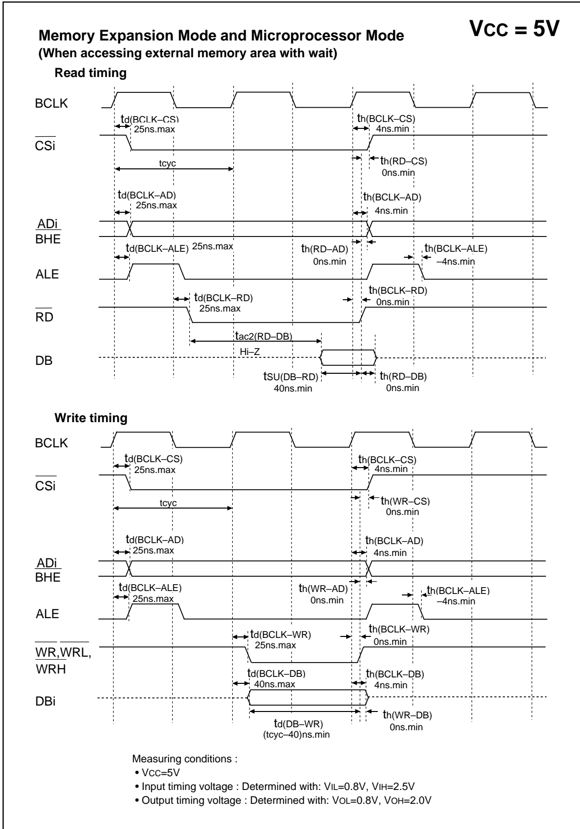
Figure 1.26.5. Vcc=5V timing diagram (4)
