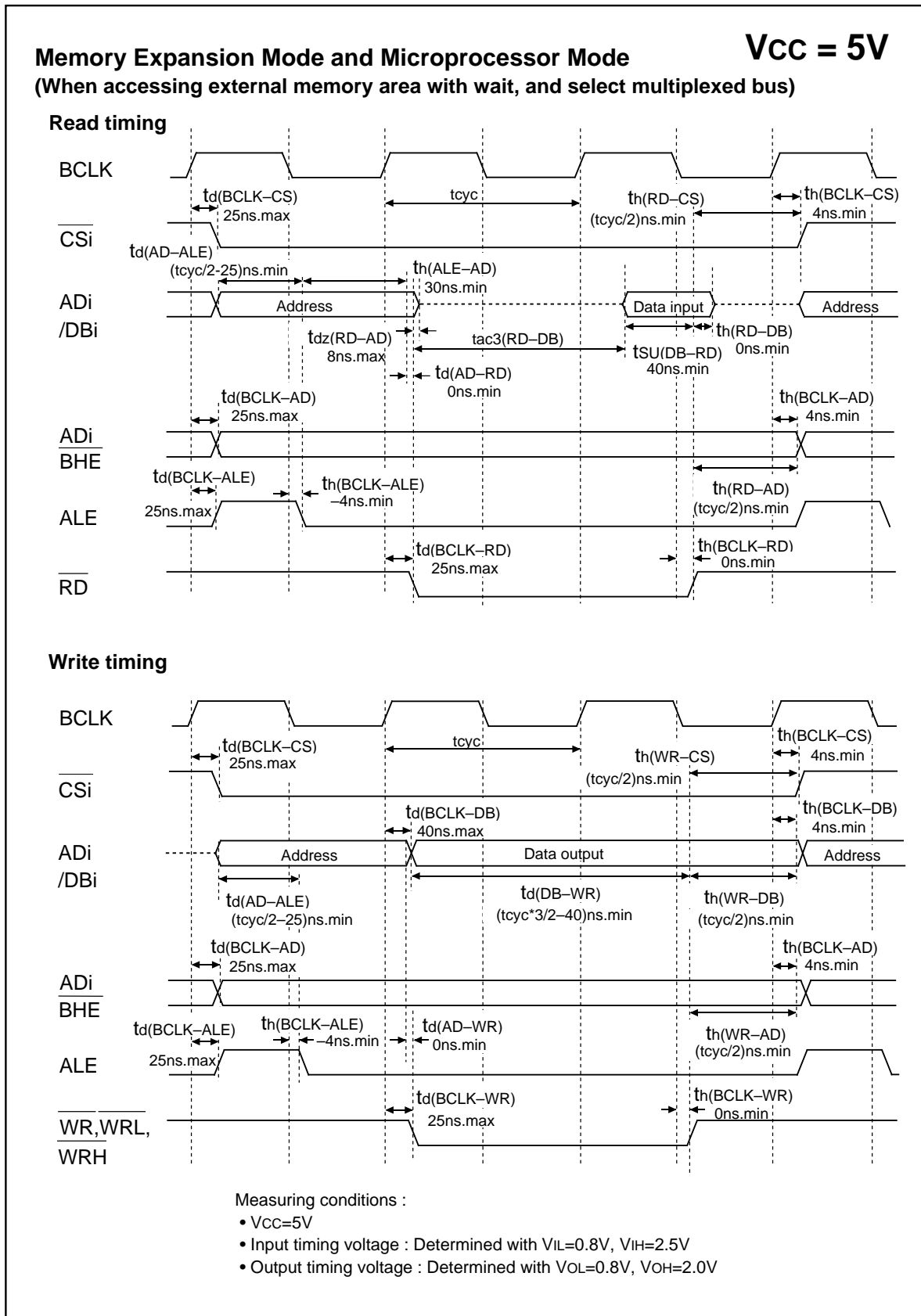
Figure 1.26.6. Vcc=5V timing diagram (5)
