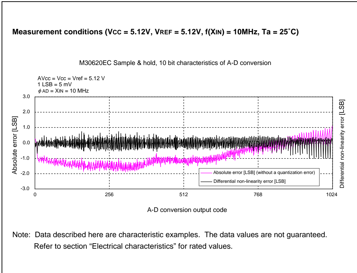
Figure 7.2.1. Standard characteristics of the A-D converter
