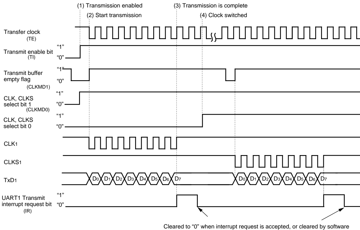
Figure 2.4.10. Operation timing of transmission in clock-synchronous serial I/O mode, transfer clock output from multiple pins function selected
