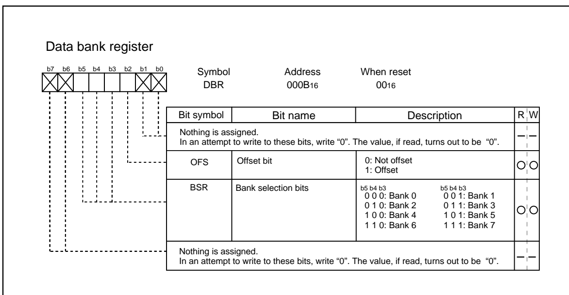
Figure 5.3.5. Data bank register
