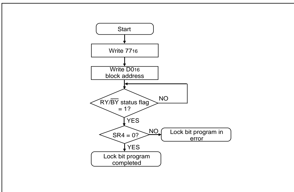
Figure 1.29.6. Lock bit program flowchart
