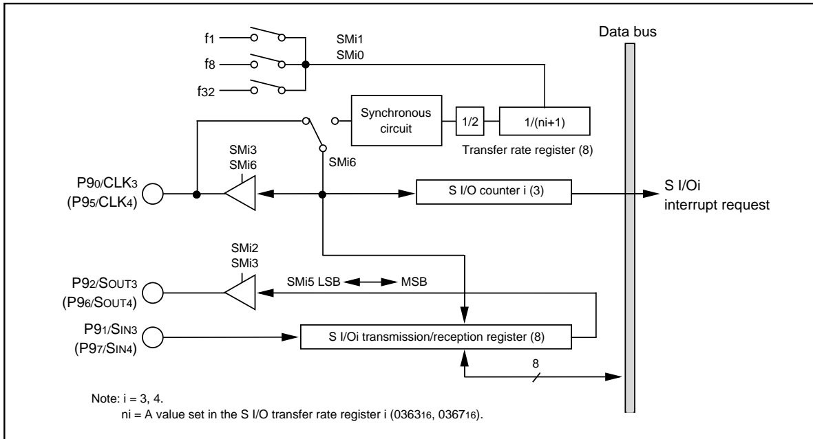
Figure 1.19.31. S I/O3, 4 block diagram
