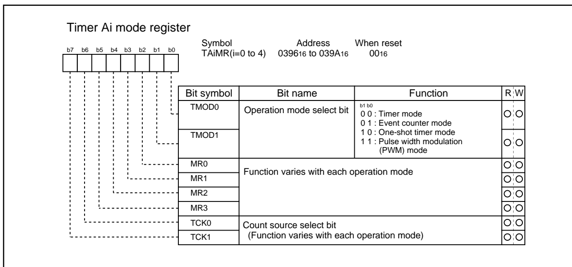
Figure 1.17.4. Timer A-related registers (1)
