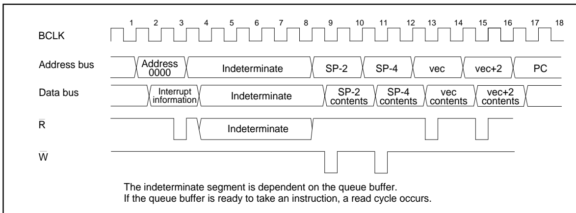
Figure 4.3.2. Time required for executing the interrupt sequence
