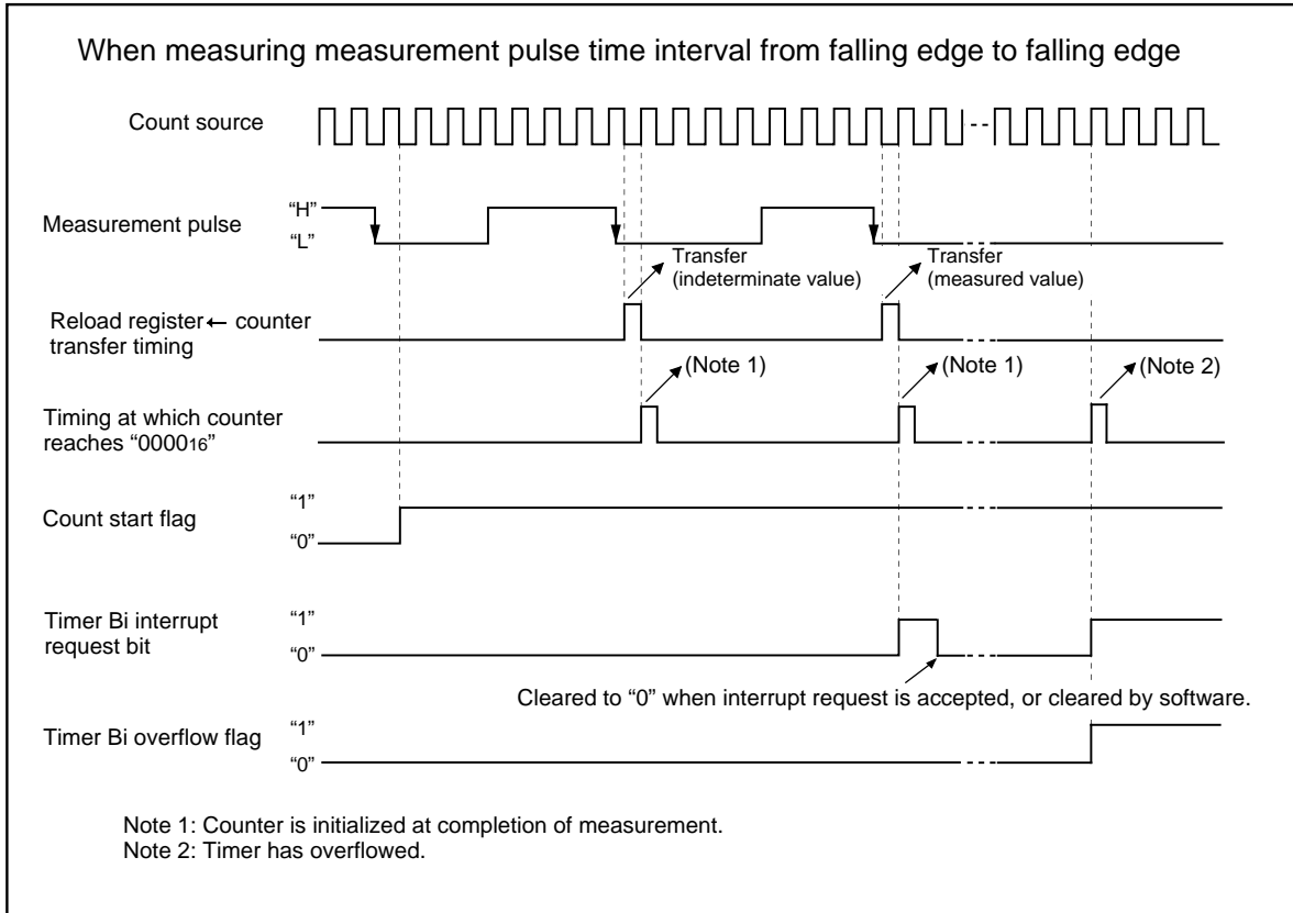
Figure 1.17.20. Operation timing when measuring a pulse period
