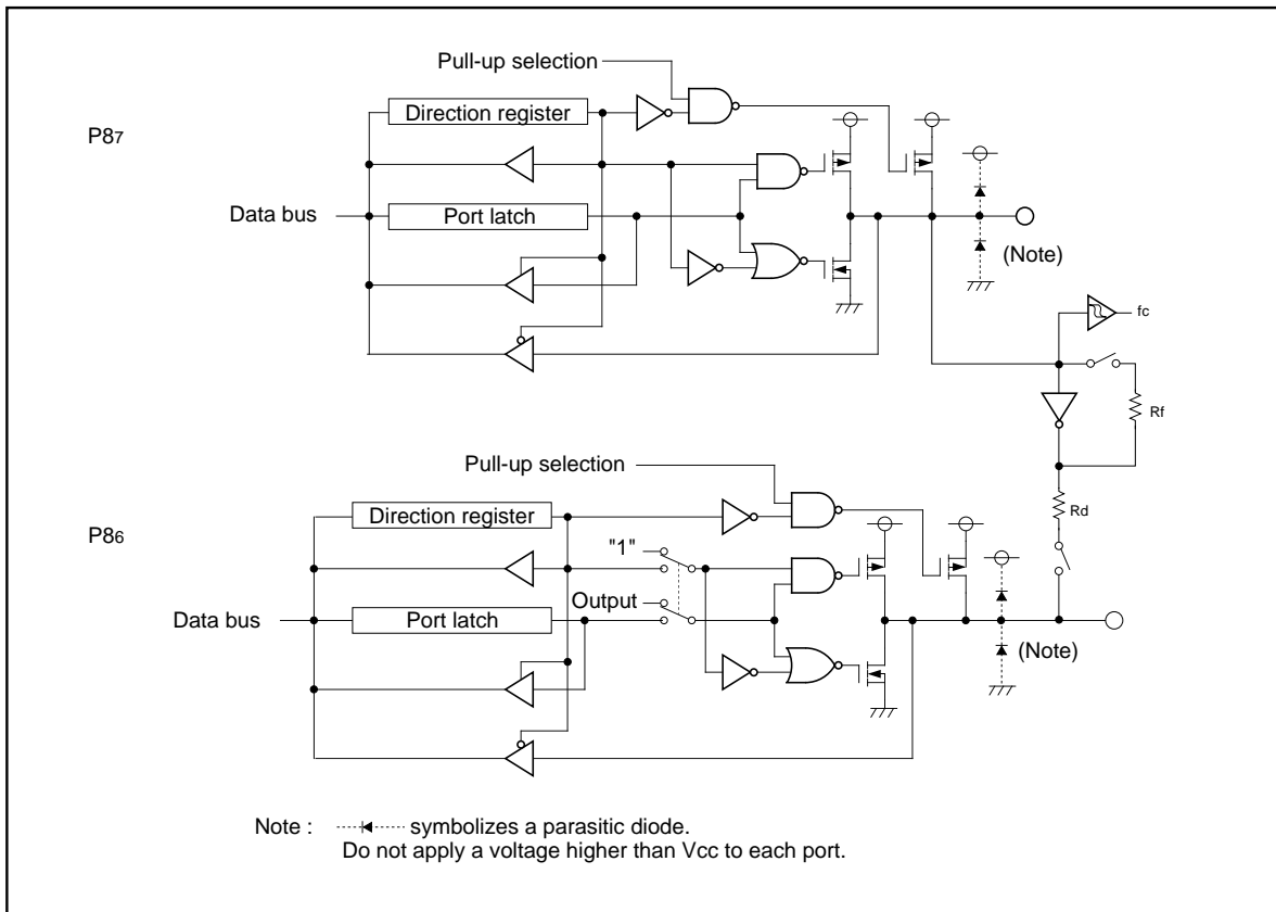
Figure 1.23.4. Programmable I/O ports (4)
