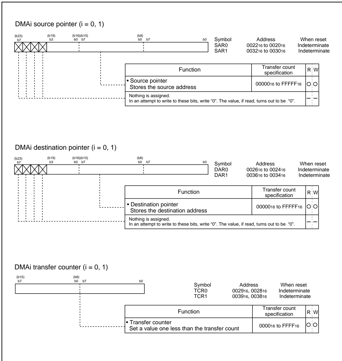
Figure 1.16.4. DMAC register (3)
