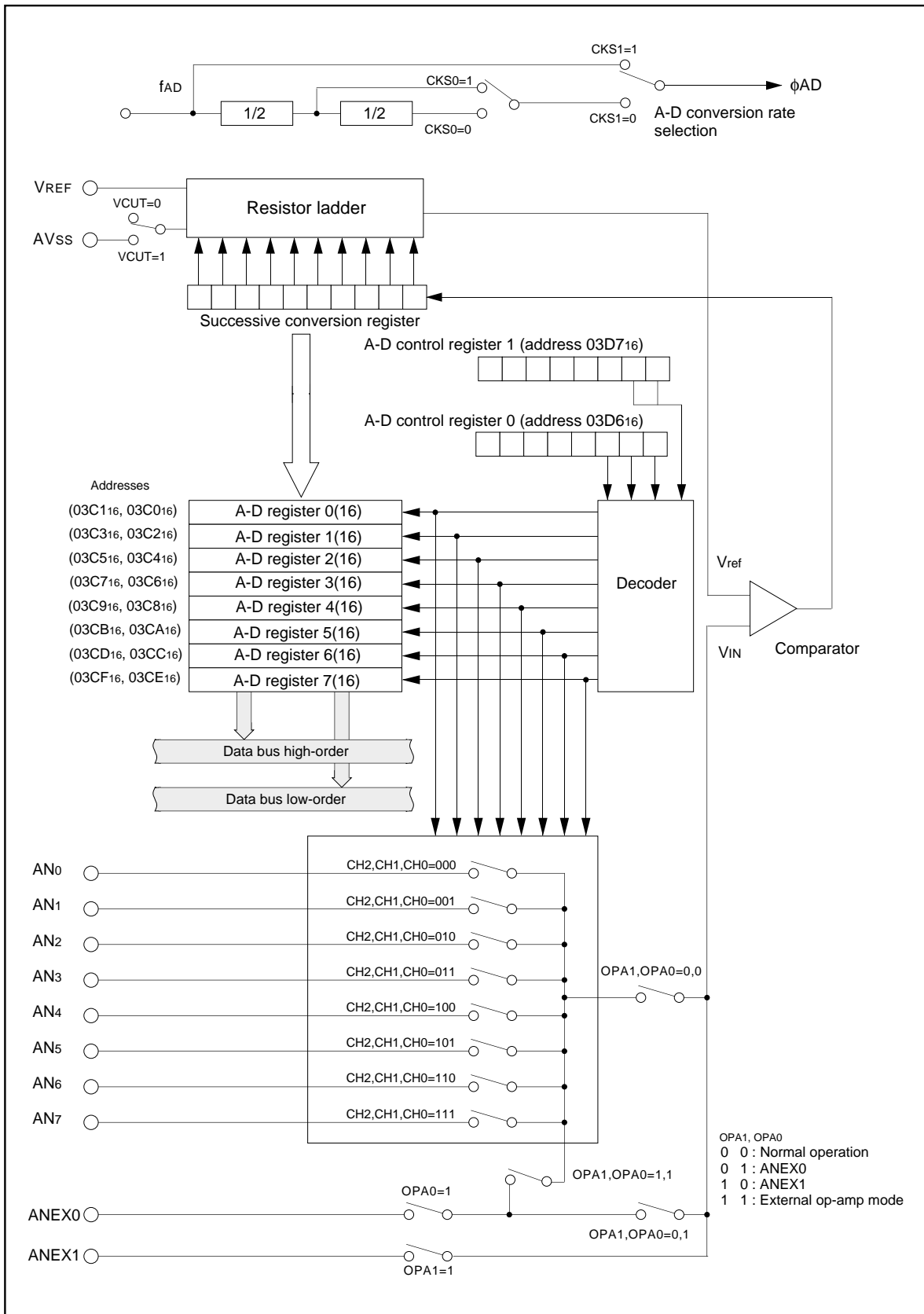
Figure 1.20.1. Block diagram of A-D converter
