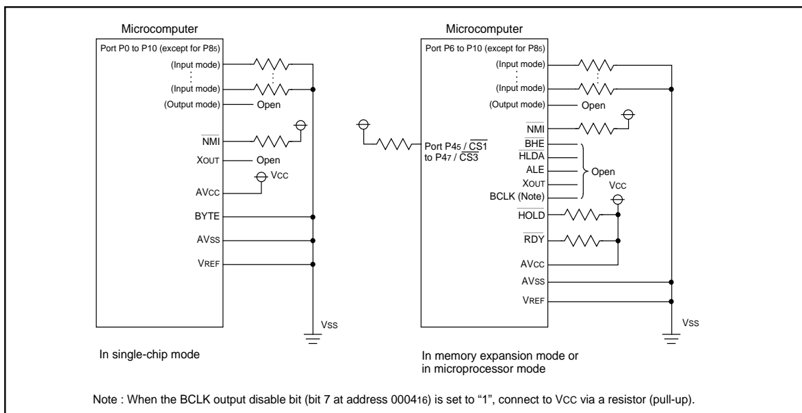
Figure 1.23.10. Example connection of unused pins
