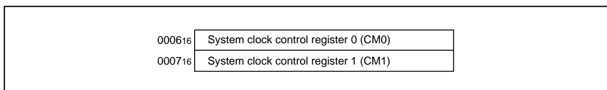
Figure 2.14.3. Memory map of power control-related registers
