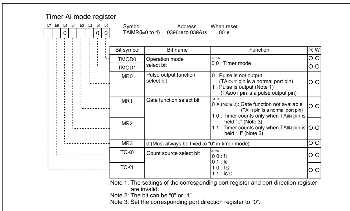
Figure 1.17.7. Timer Ai mode register in timer mode
