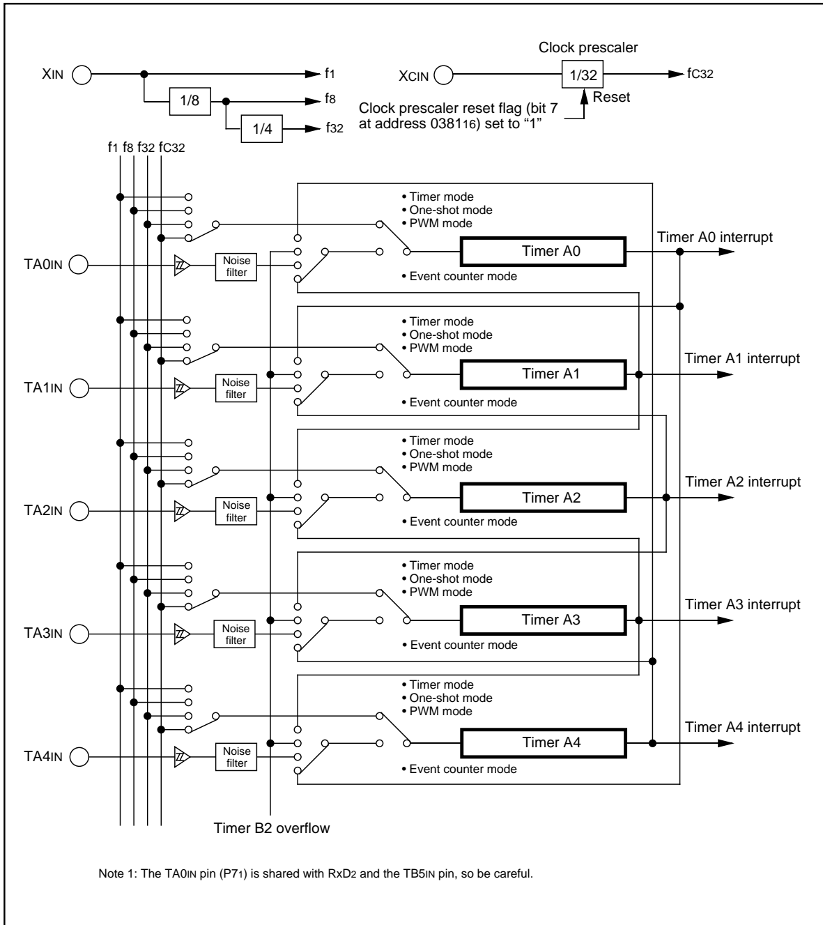
Figure 1.17.1. Timer A block diagram
