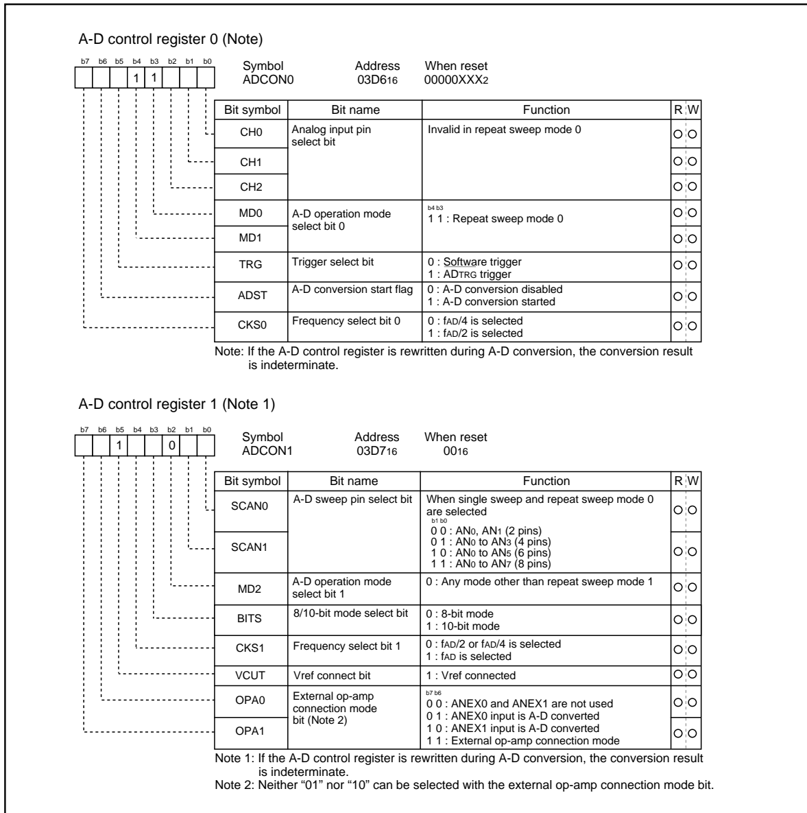
Figure 1.20.7. A-D conversion register in repeat sweep mode 0
