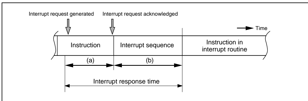
Figure 4.3.1. Interrupt response time
