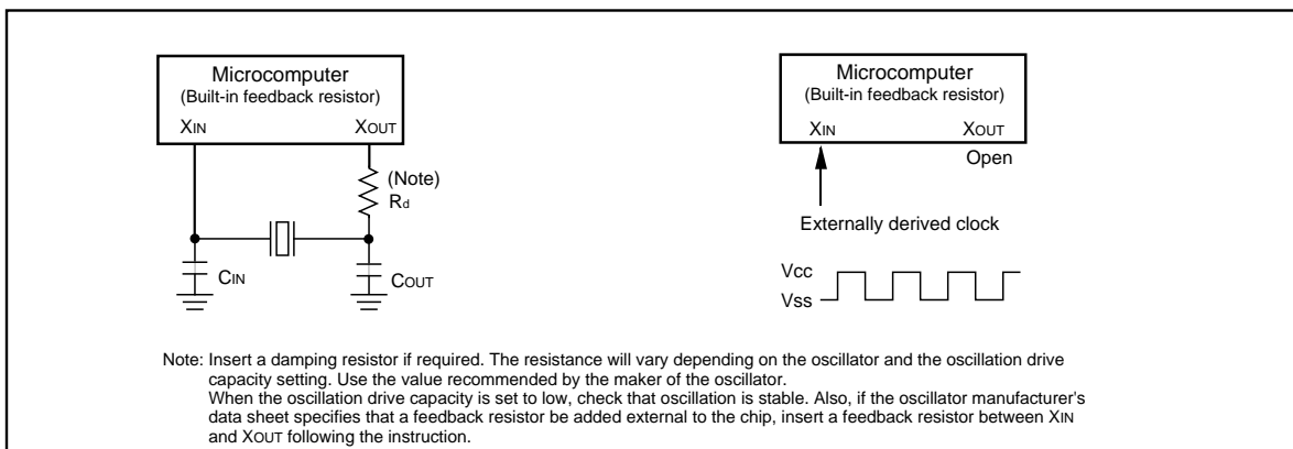
Figure 1.13.1. Examples of main clock
