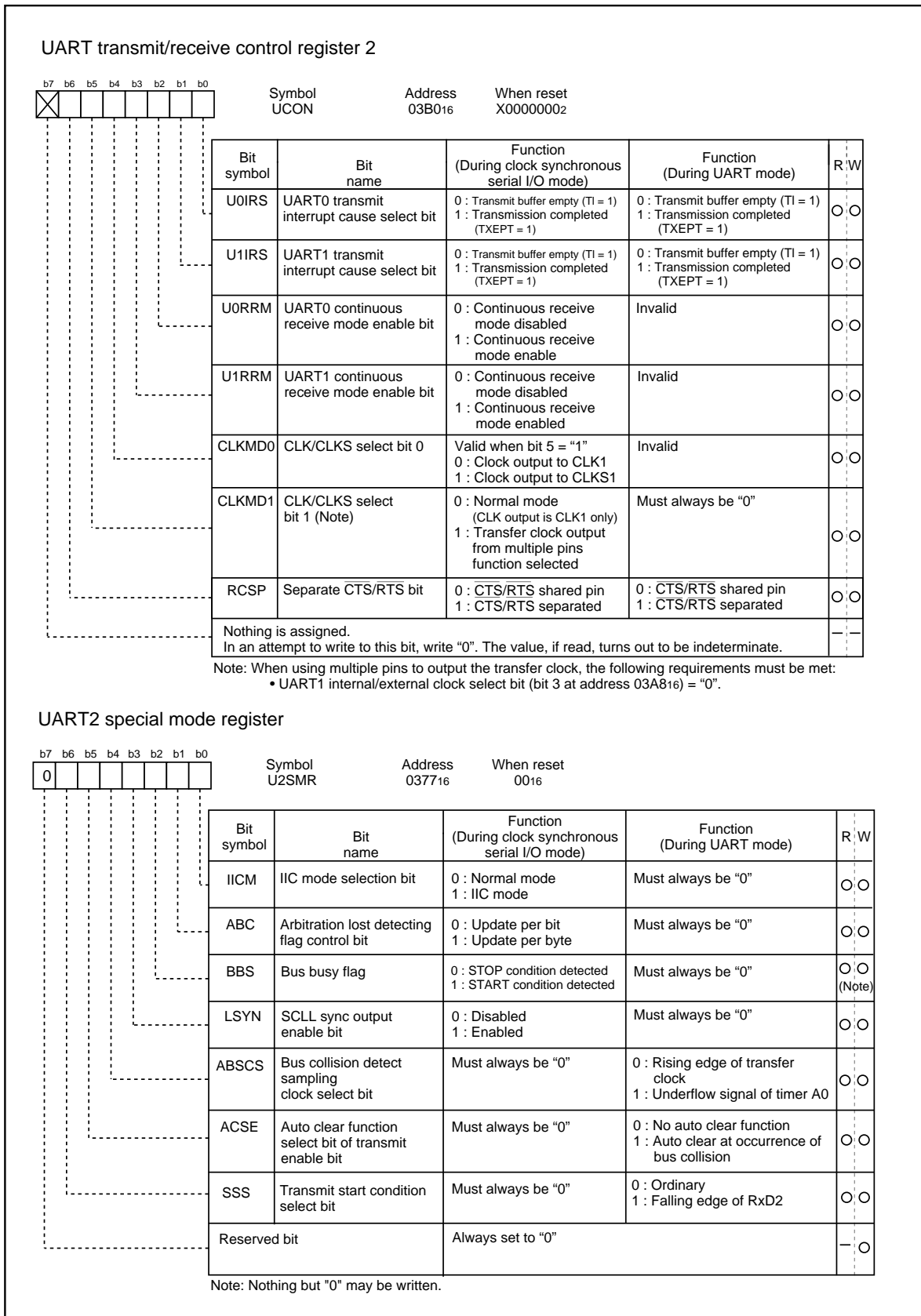
Figure 1.19.8. Serial I/O-related registers (5)
