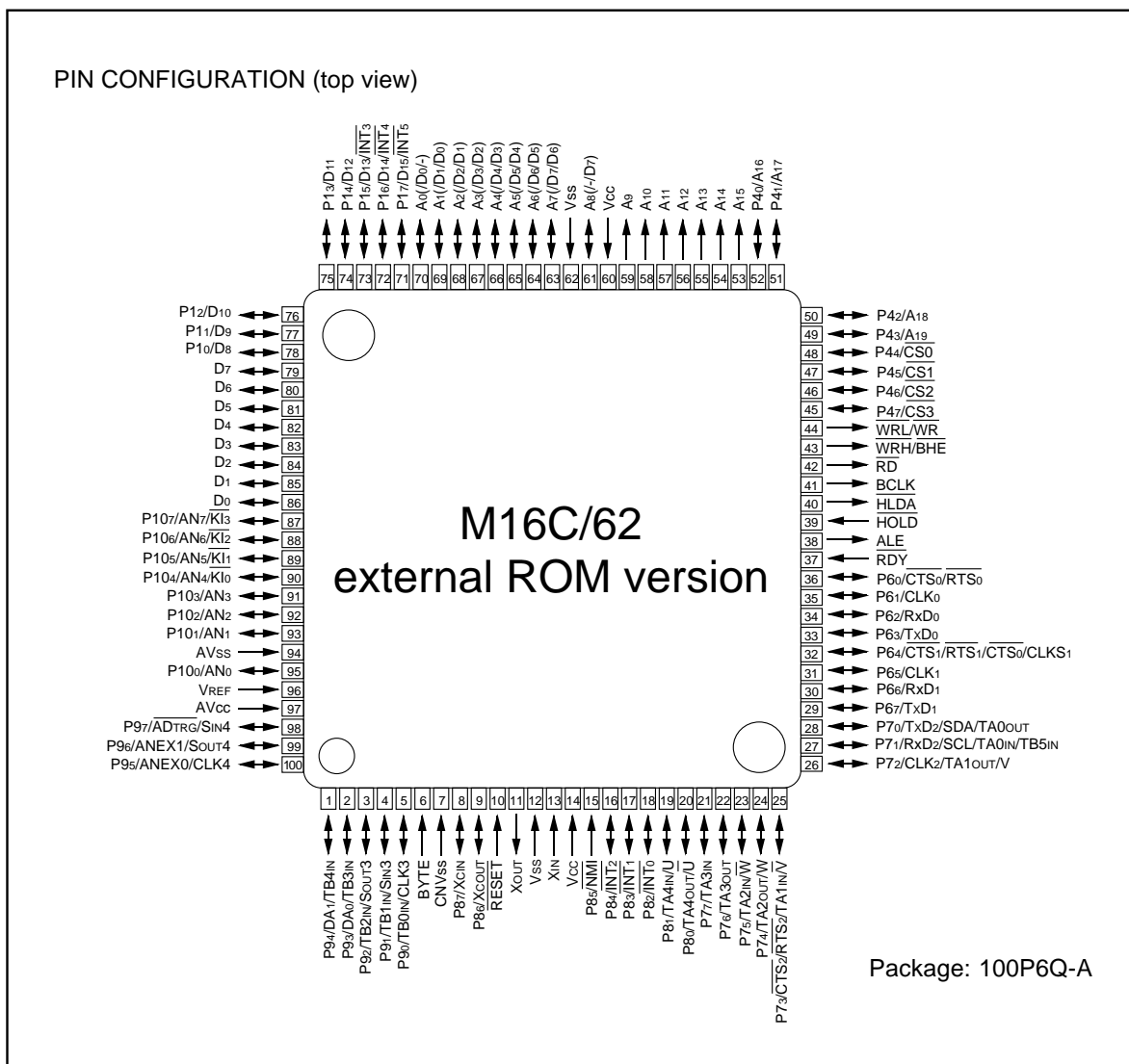
Figure 6.1.2. Pin configuration (top view)
