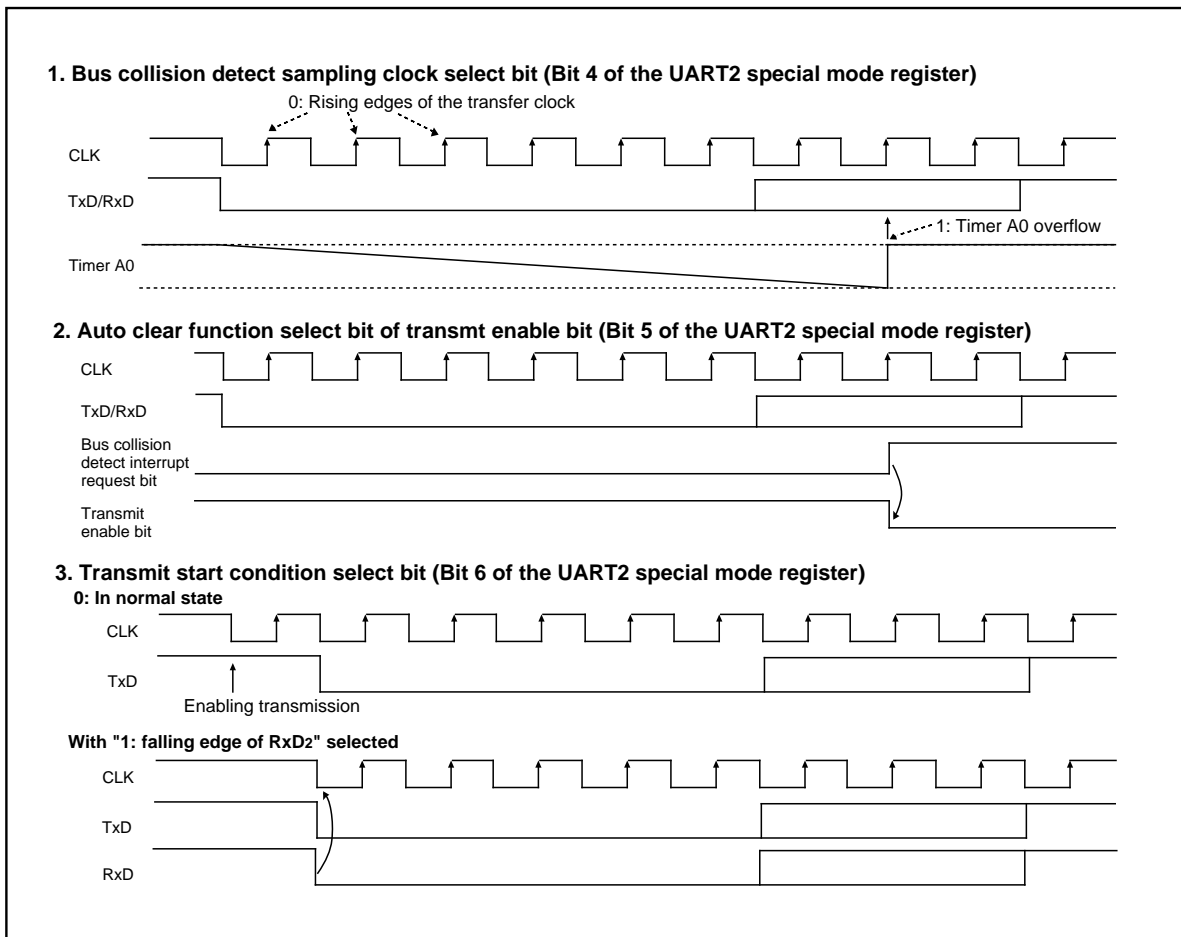
Figure 1.19.28. Some other functions added
