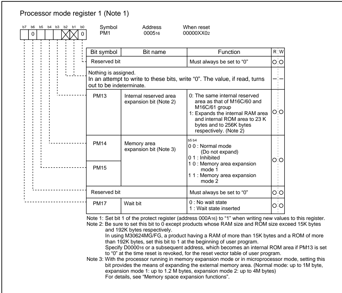
Figure 5.3.1. Processor mode register 1
