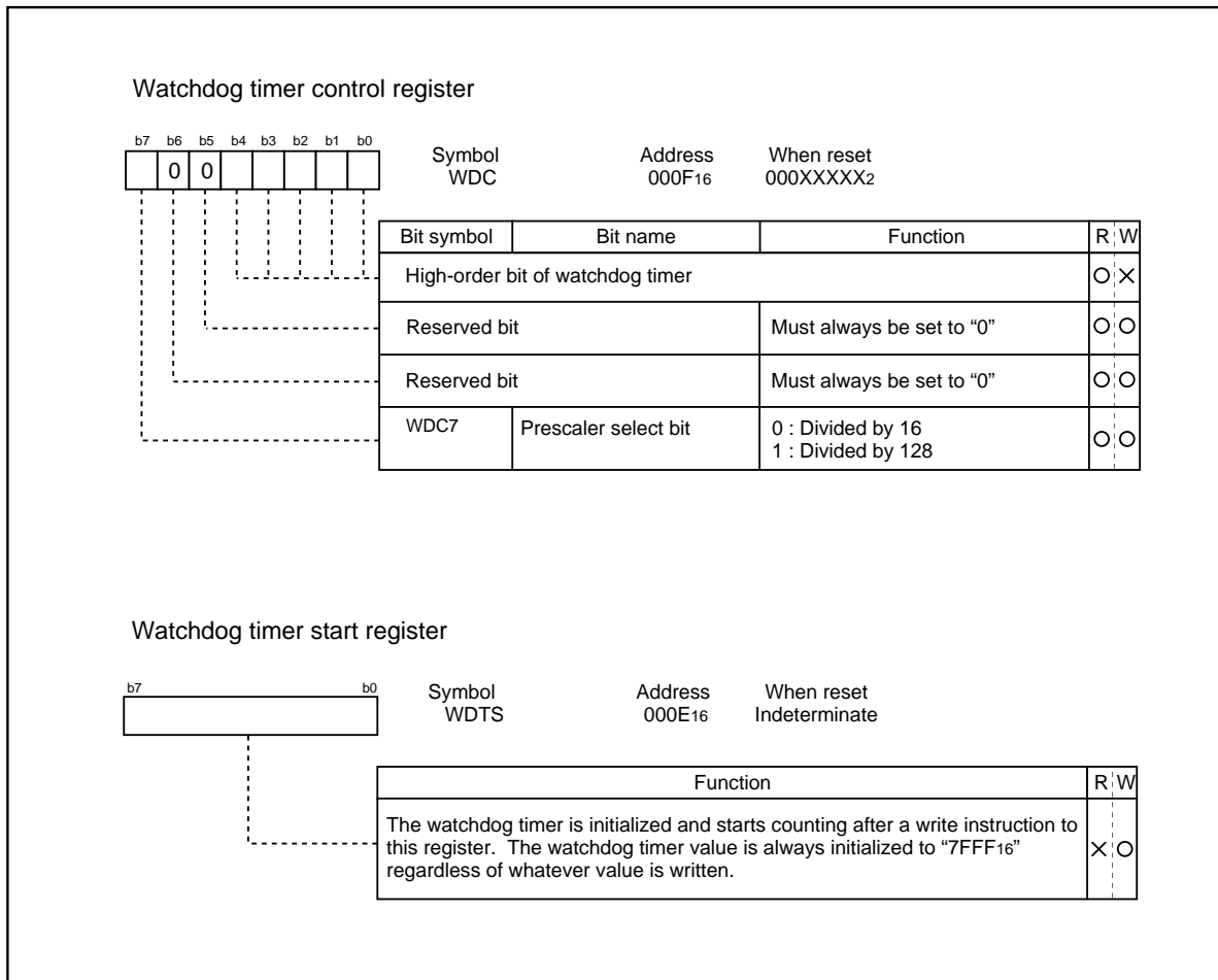
Figure 1.15.2. Watchdog timer control and start registers
