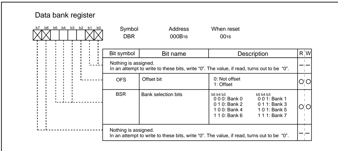
Figure 1.8.4. Data bank register
