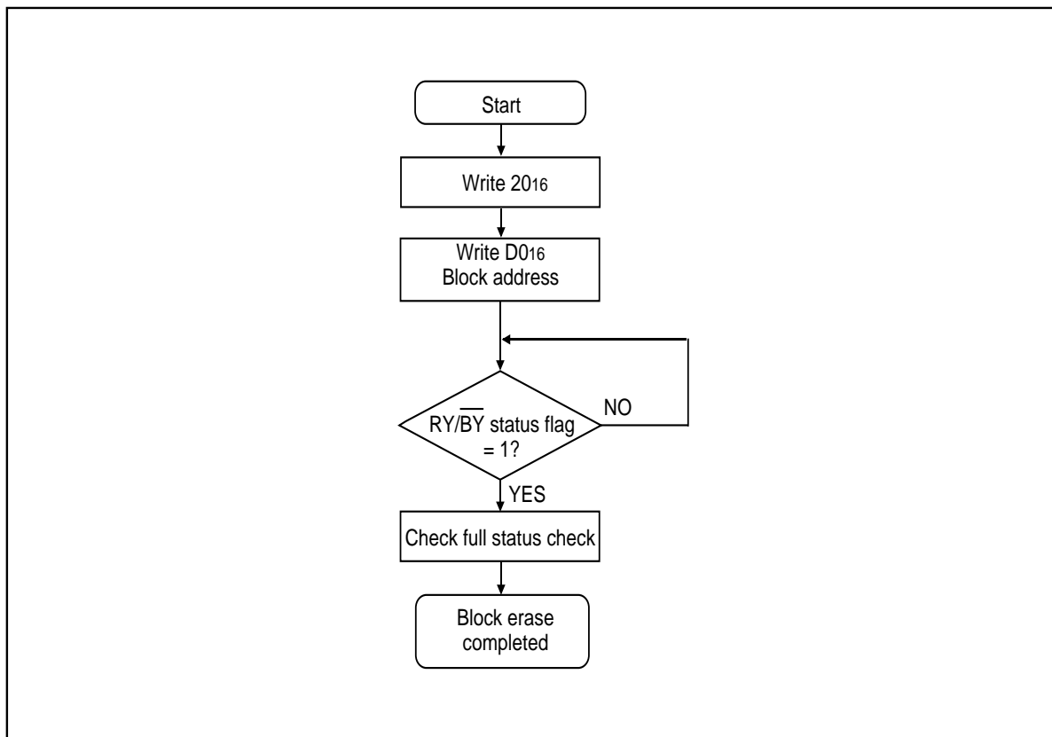
Figure 1.29.5. Block erase flowchart
