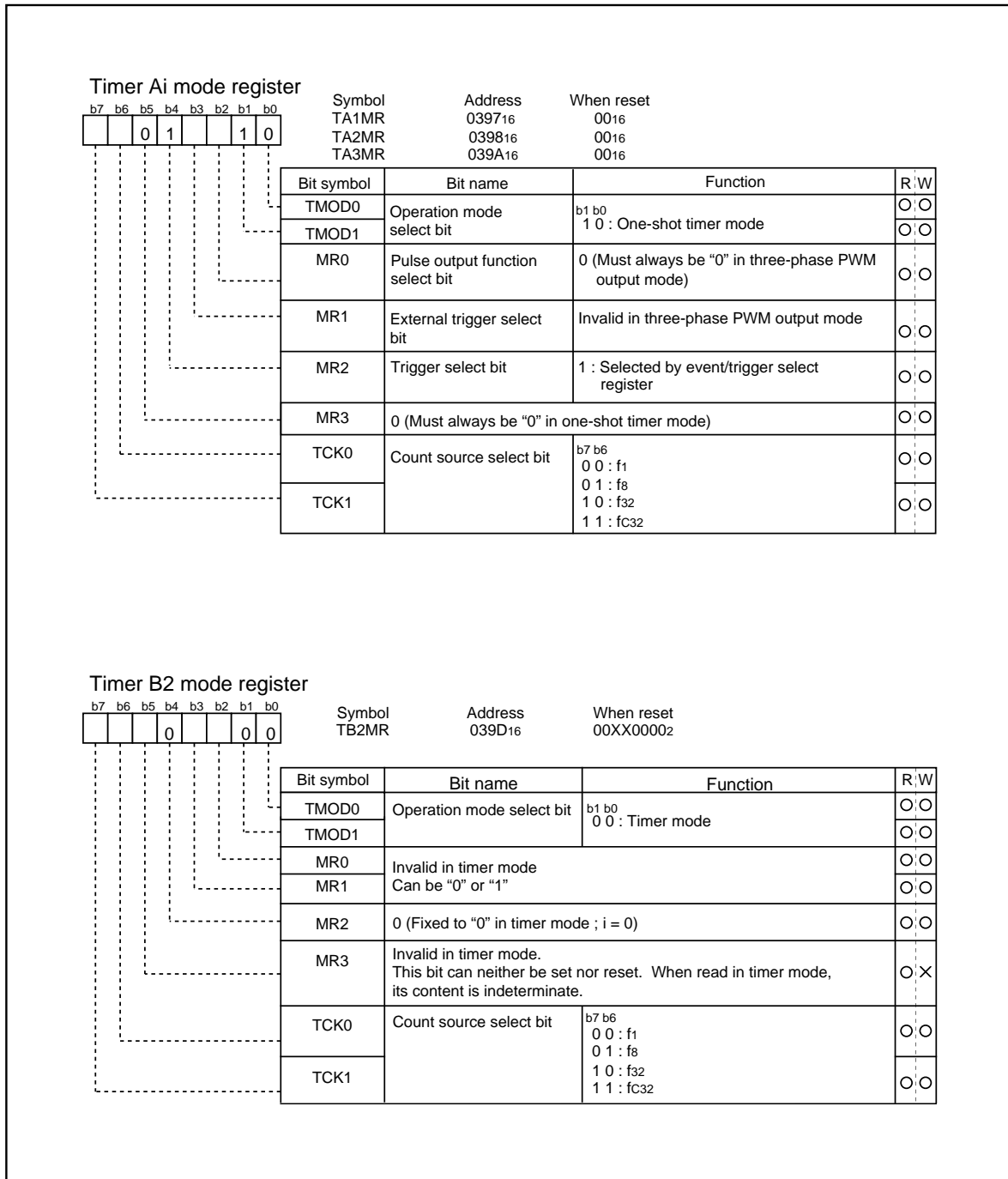
Figure 1.18.4. Timer mode registers in three-phase waveform mode
