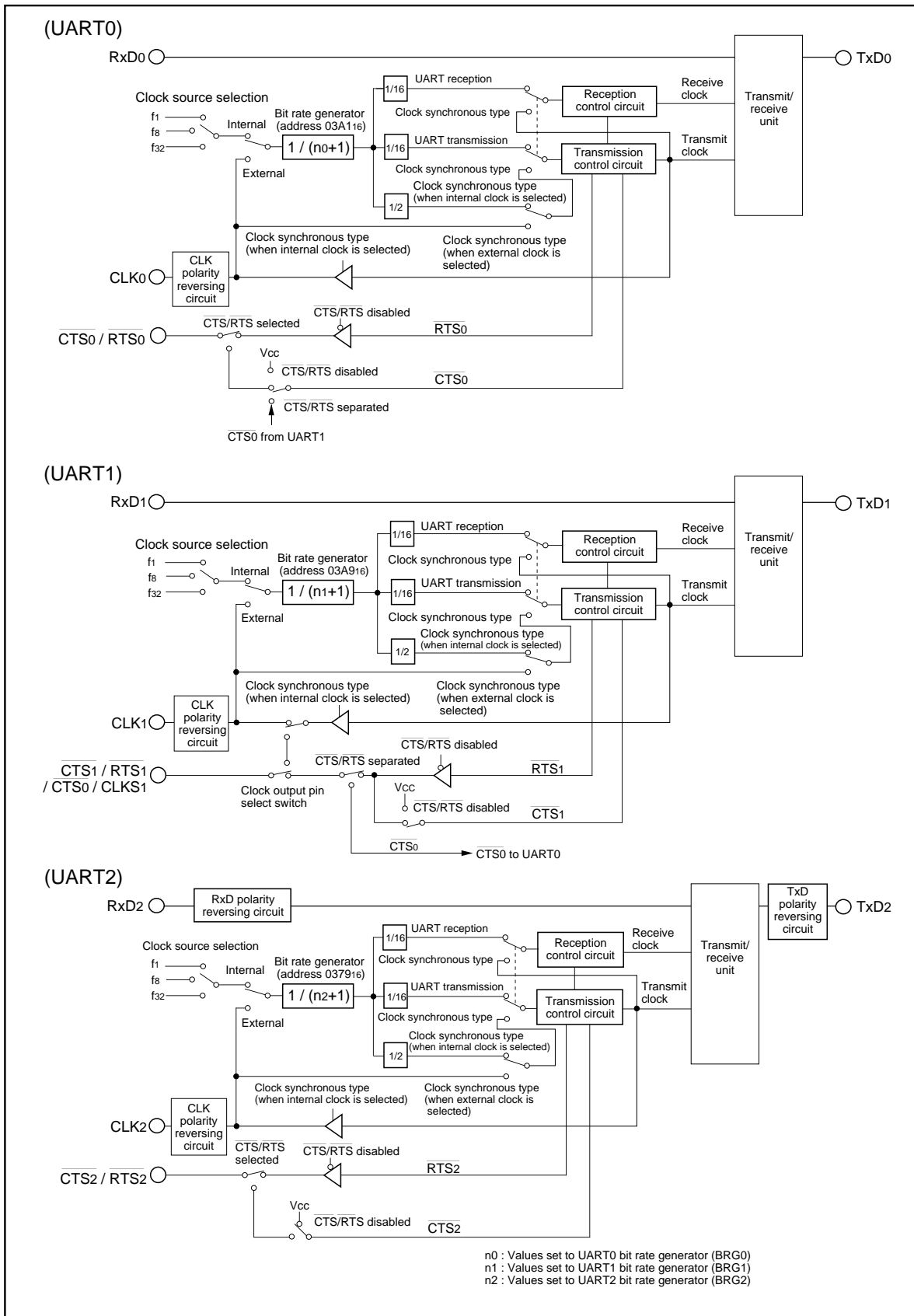
Figure 1.19.1. Block diagram of UARTi (i = 0 to 2)
