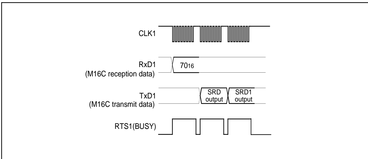
Figure 1.31.4. Timing for reading the status register
