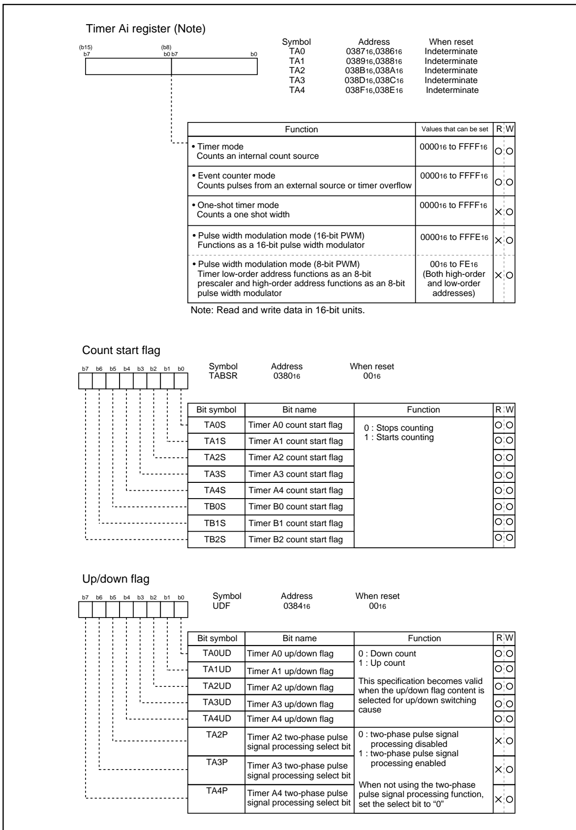
Figure 1.17.5. Timer A-related registers (2)
