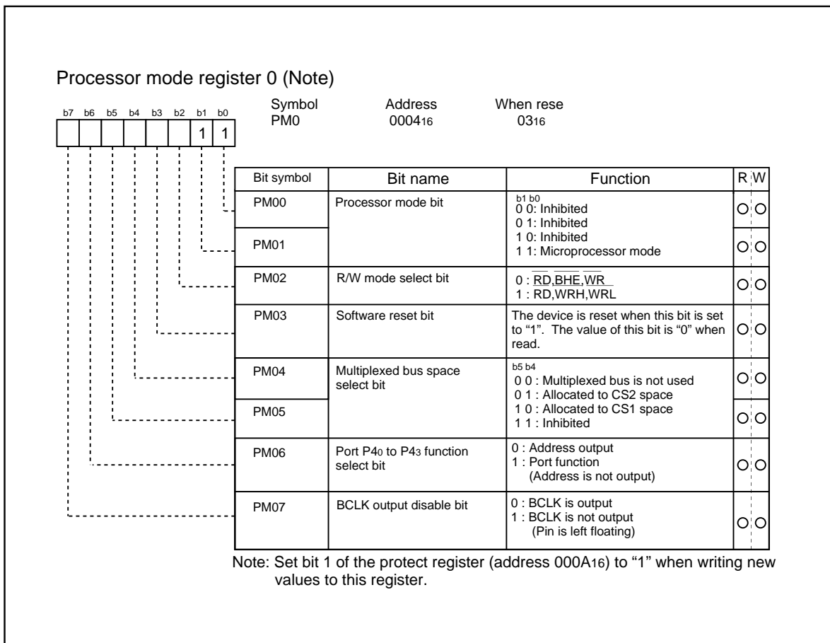
Figure 6.4.1. Processor mode register 0
