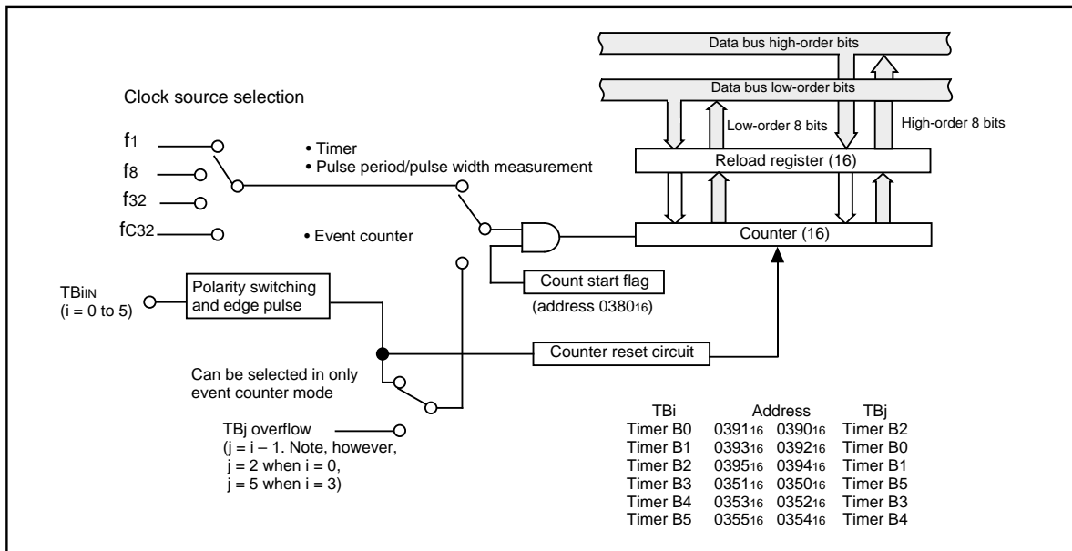
Figure 1.17.14. Block diagram of timer B
