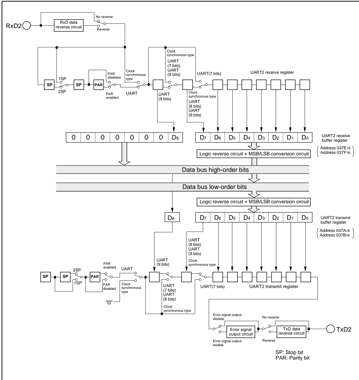
Figure 1.19.3. Block diagram of UART2 transmit/receive unit
