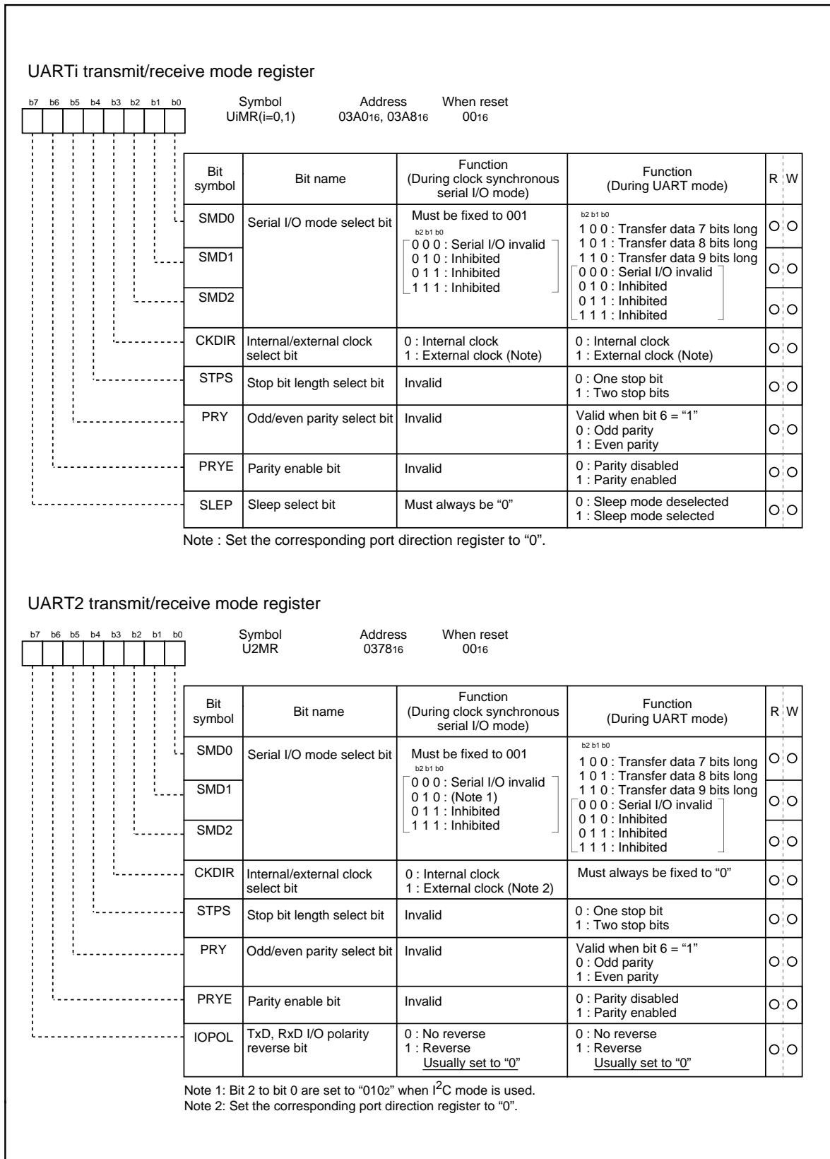
Figure 1.19.5. Serial I/O-related registers (2)
