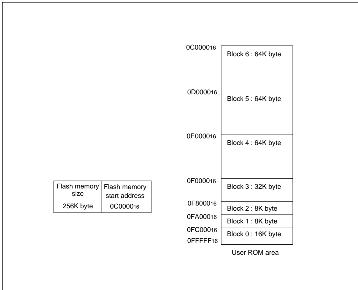
Figure 1.31.18. Blocks in the user area
