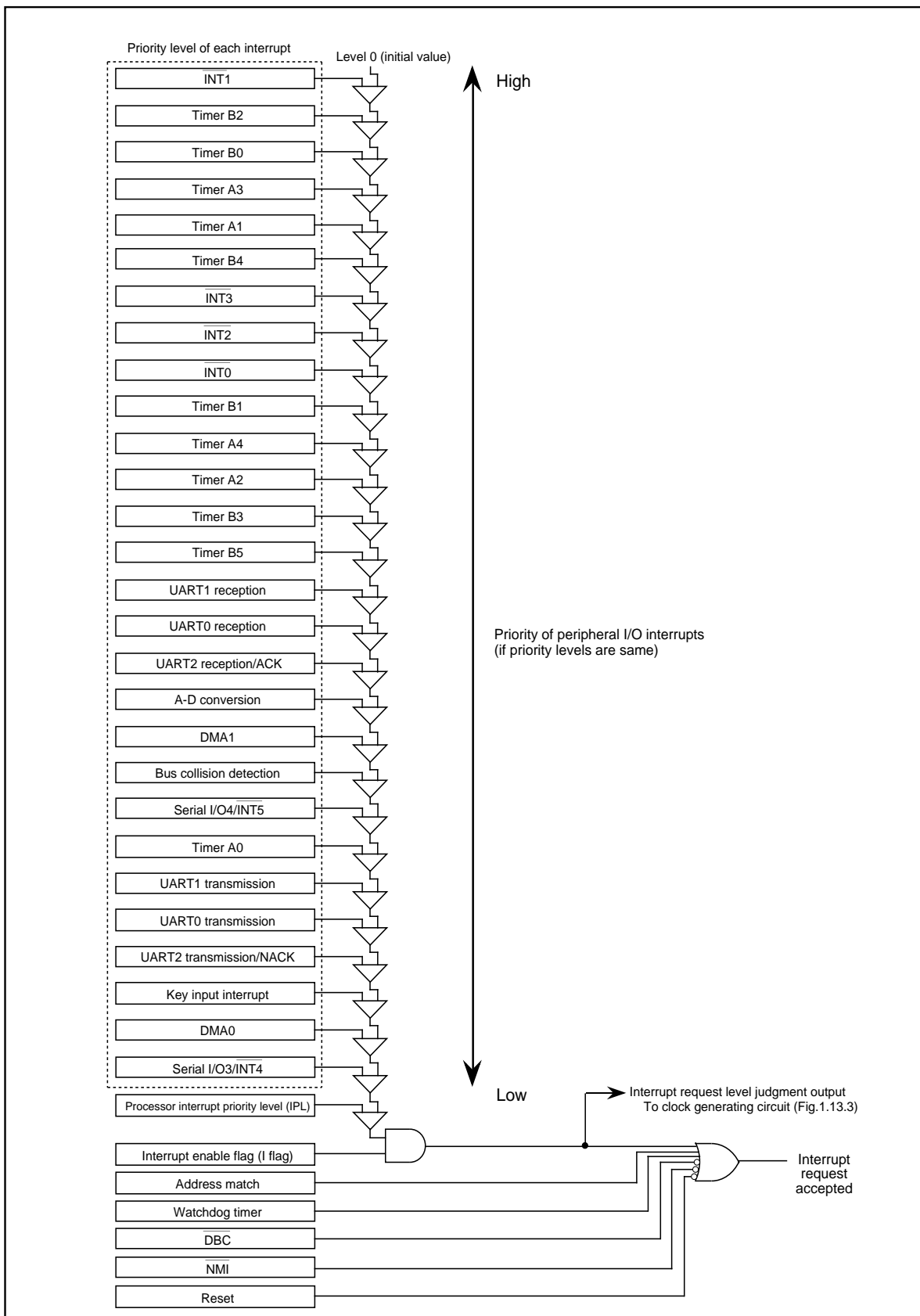
Figure 1.14.9. Maskable interrupts priorities (peripheral I/O interrupts)
