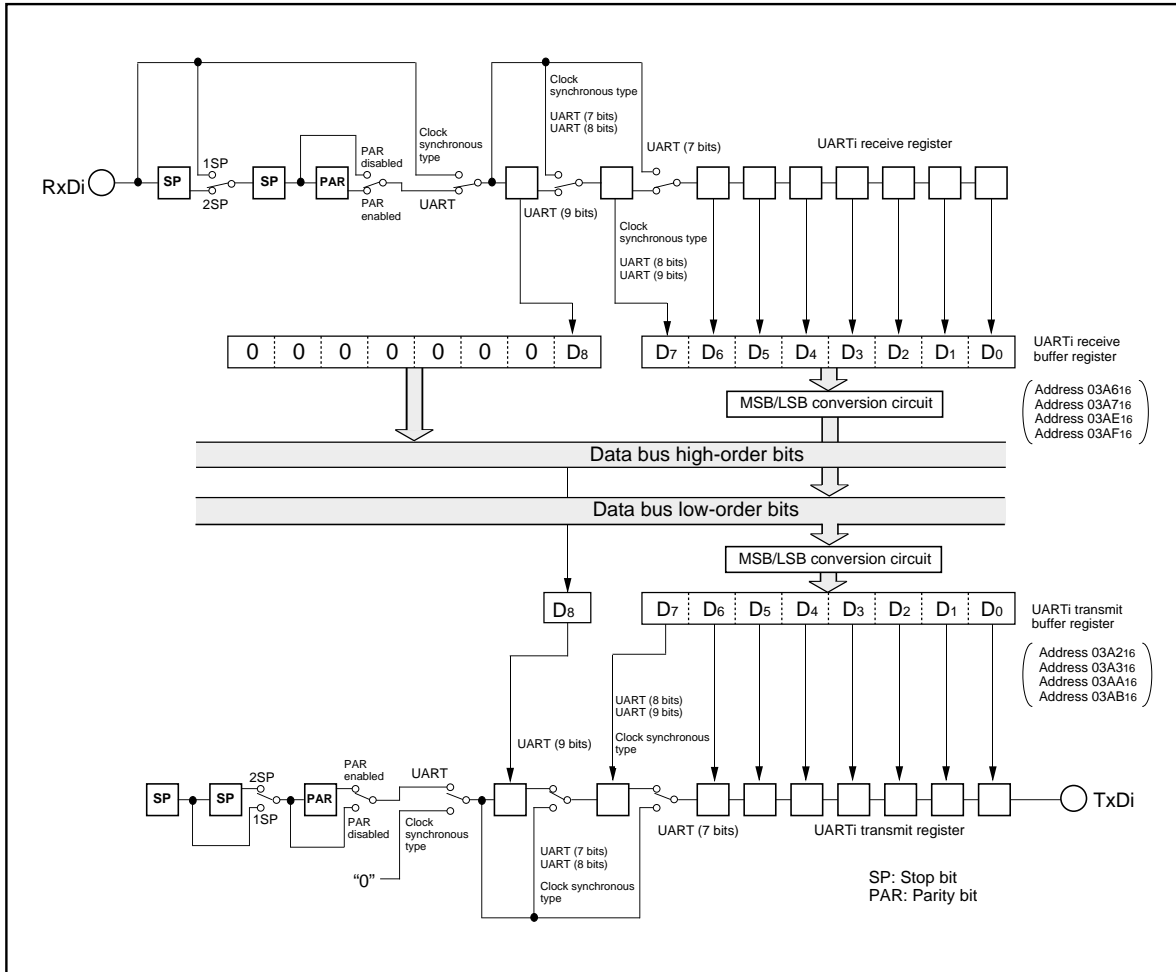
Figure 1.19.2. Block diagram of UARTi (i = 0, 1) transmit/receive unit
