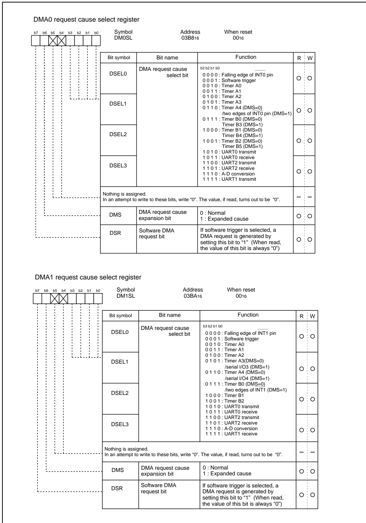
Figure 2.9.2. DMAC-related registers (1)
