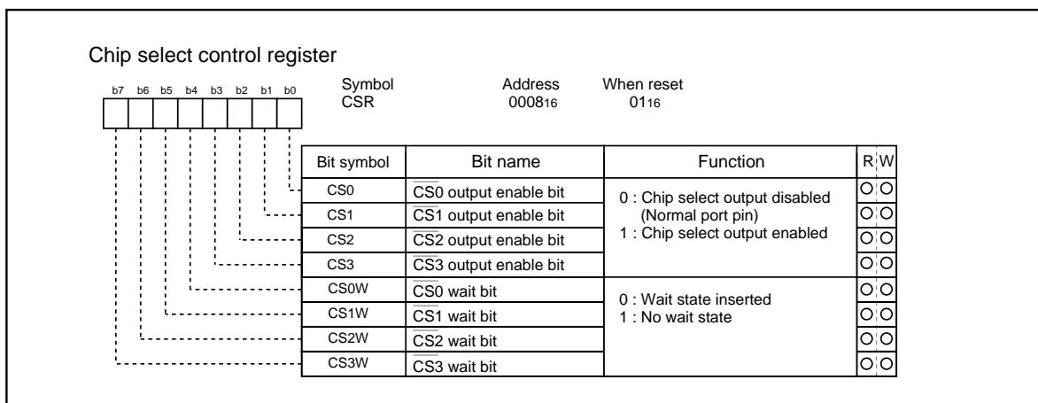
Figure 5.2.3. Chip select control register
