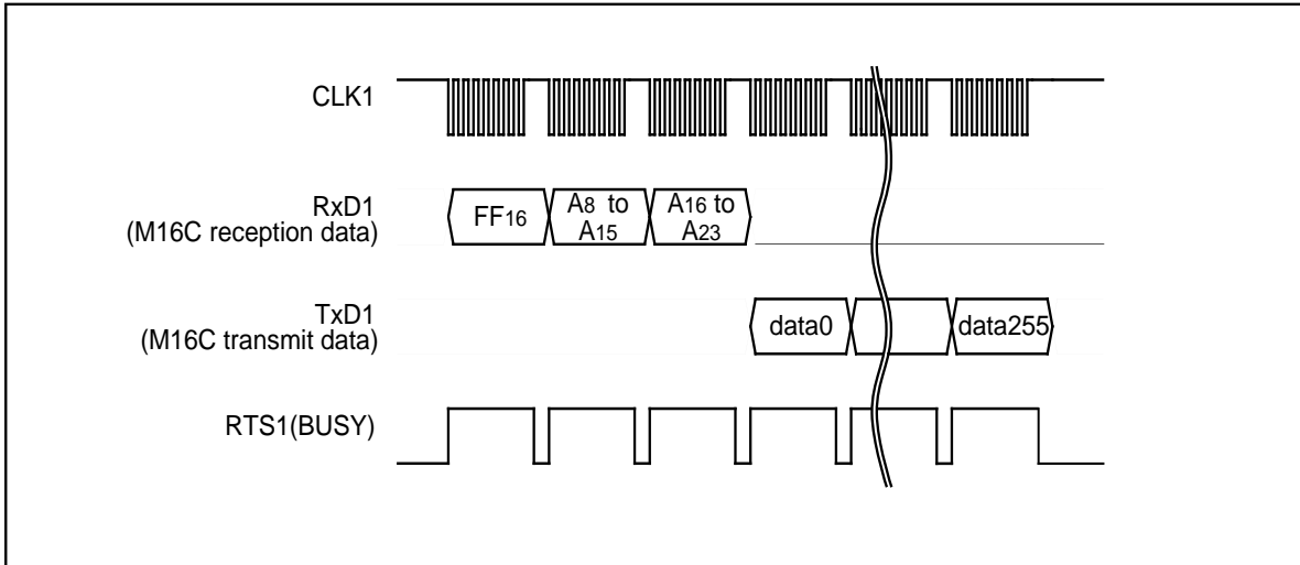
Figure 1.31.3. Timing for page read
