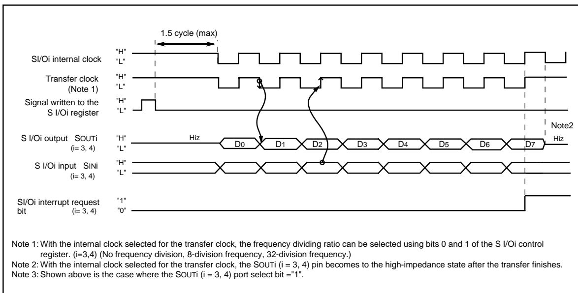
Figure 1.19.34. S I/Oi operation timing chart
