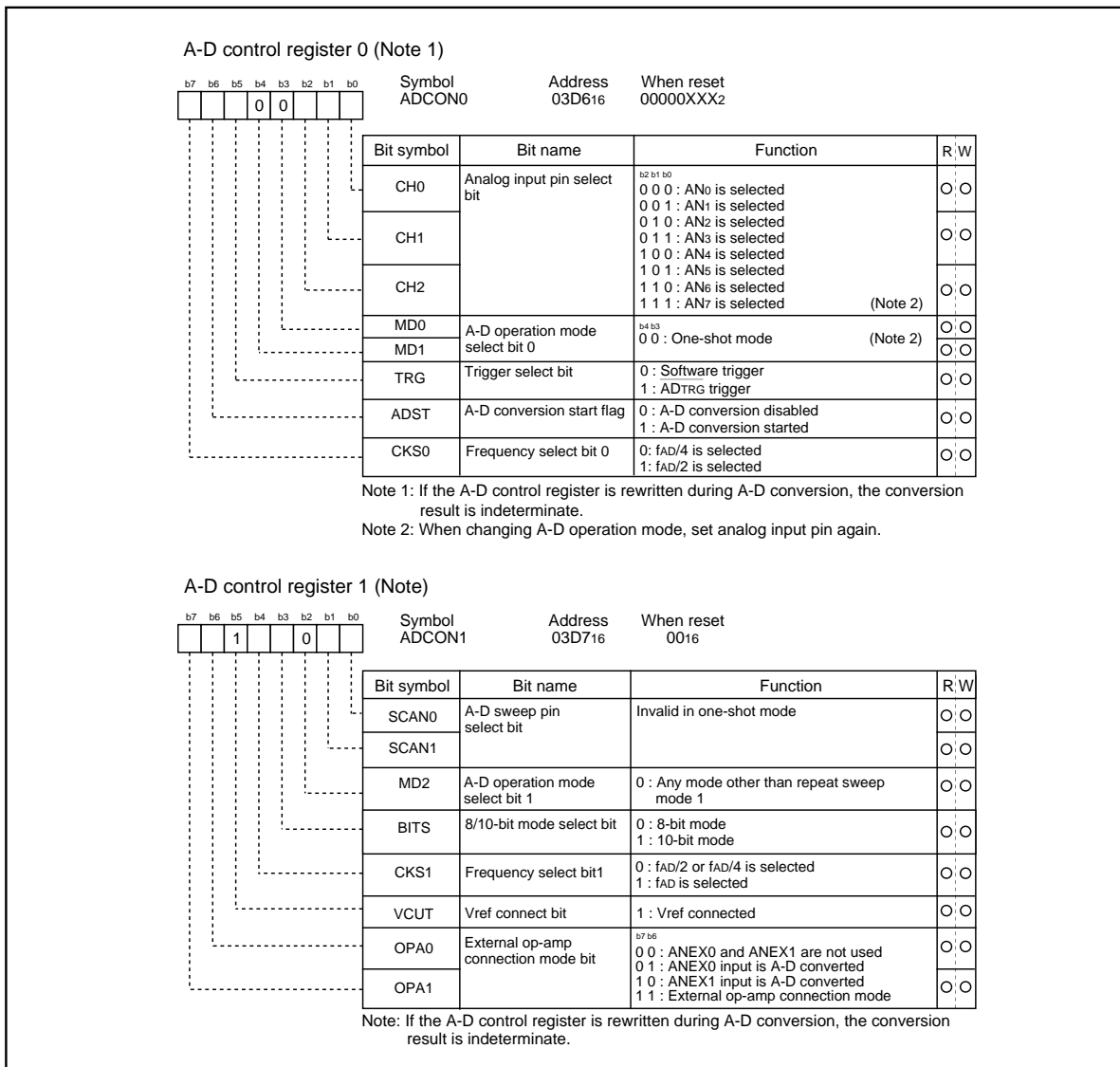
Figure 1.20.4. A-D conversion register in one-shot mode
