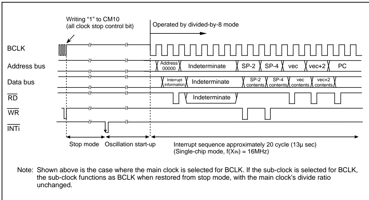
Figure 2.14.2. Sequence of returning from stop mode
