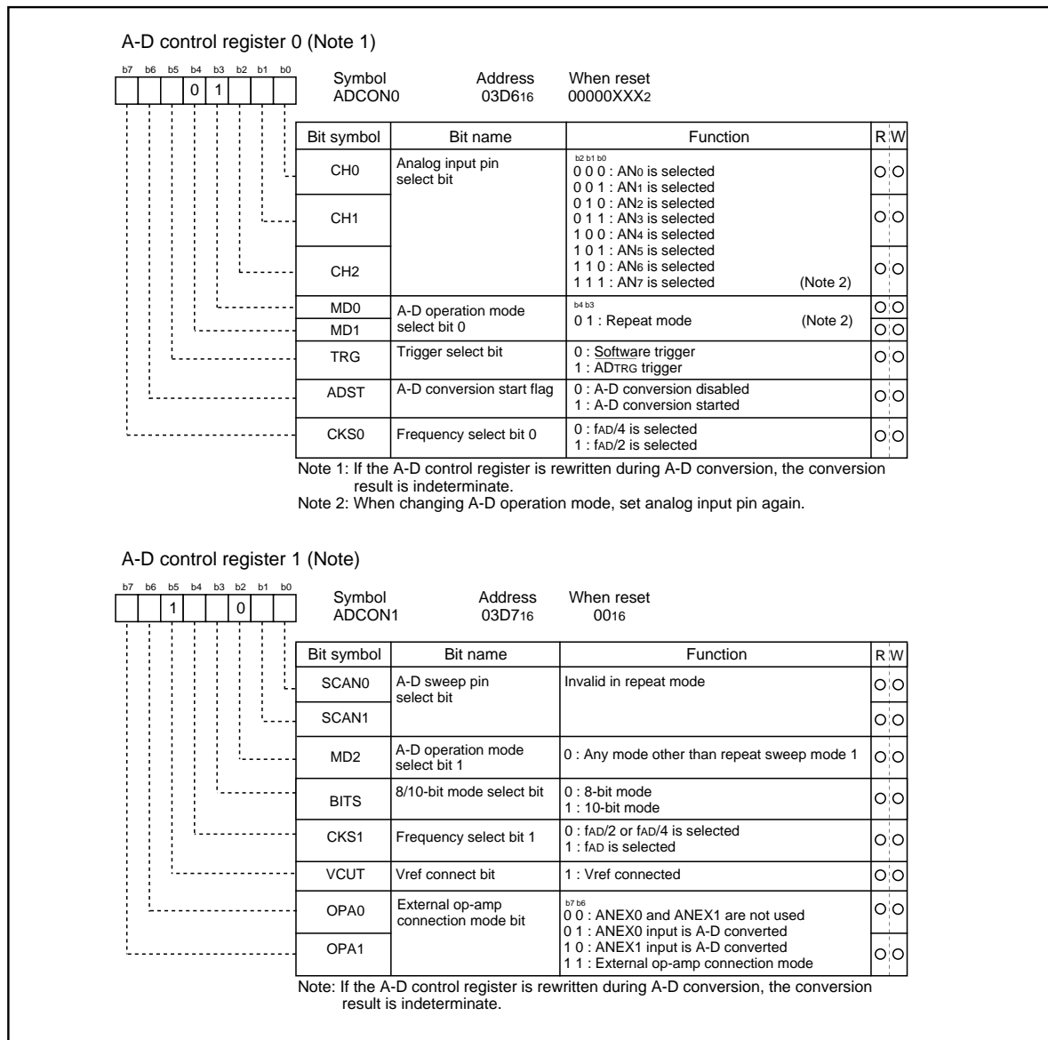
Figure 1.20.5. A-D conversion register in repeat mode
