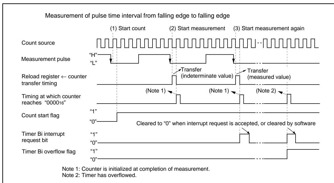
Figure 2.3.8. Operation timing of pulse period measurement mode
