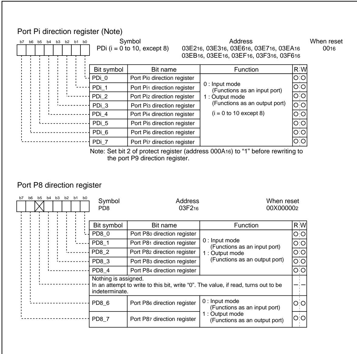
Figure 1.23.6. Direction register
