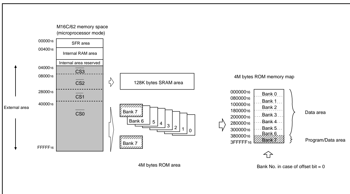
Figure 5.3.7. Memory map
