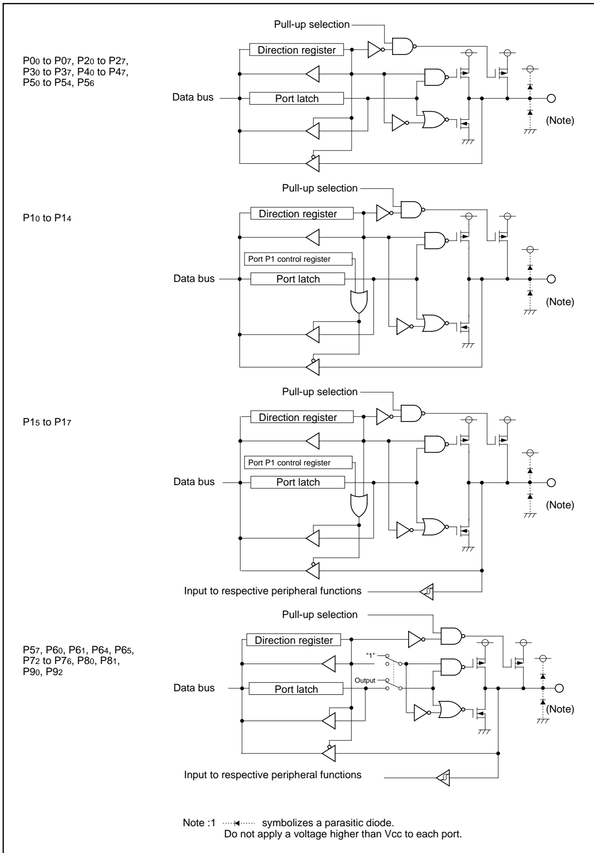
Figure 1.23.1. Programmable I/O ports (1)
