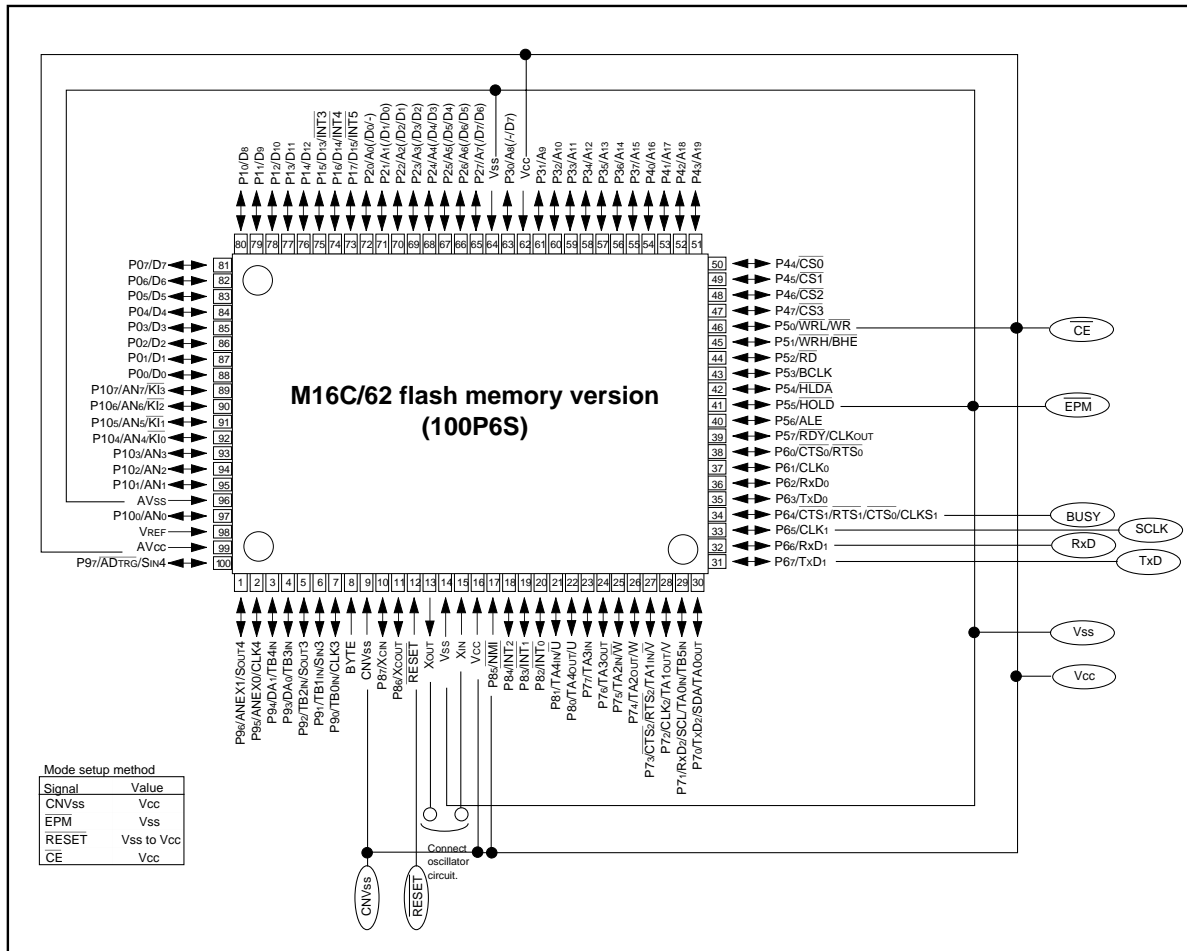
Figure 1.31.1. Pin connections for serial I/O mode (1)
