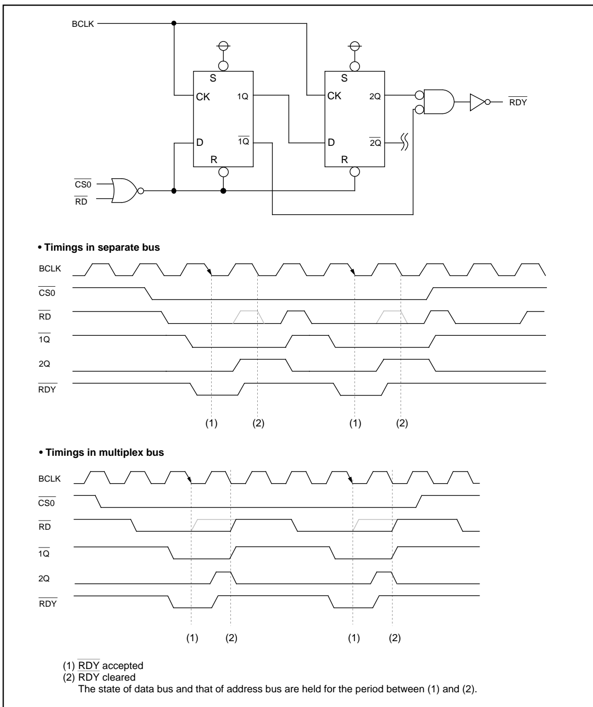
Figure 5.5.6. Example of \overline{RDY} circuit holding state of bus for 1 BCLK
