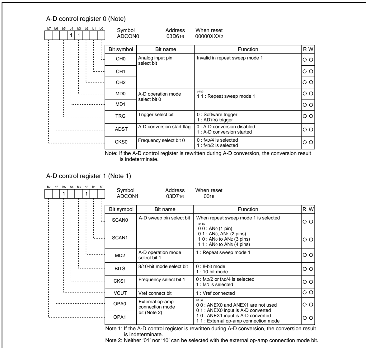
Figure 1.20.8. A-D conversion register in repeat sweep mode 1
