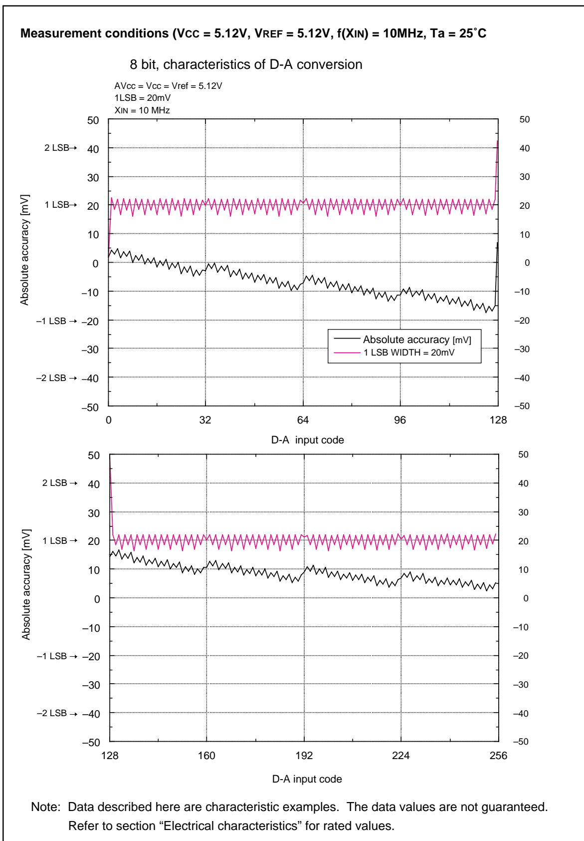
Figure 7.3.1. Characteristics of the D-A converter
