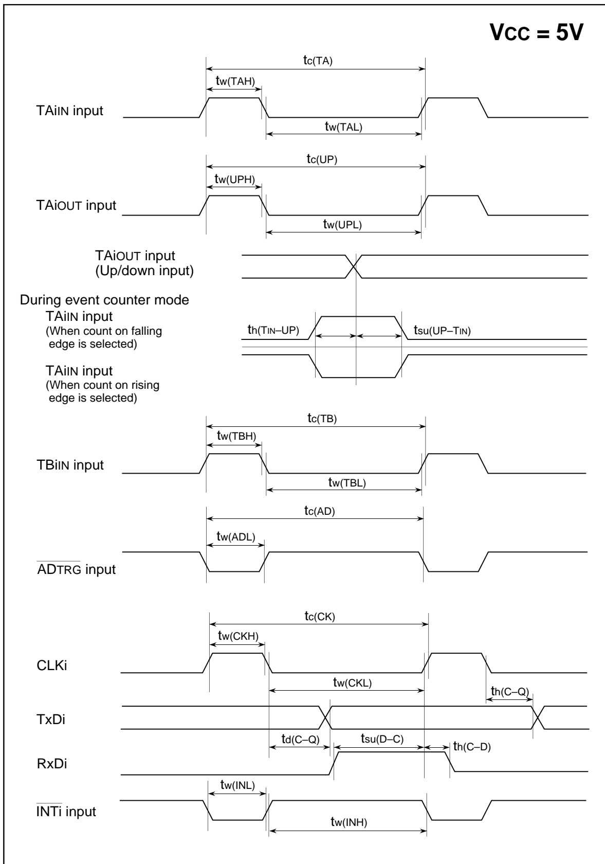
Figure 1.26.2. V_{CC}=5V timing diagram (1)
