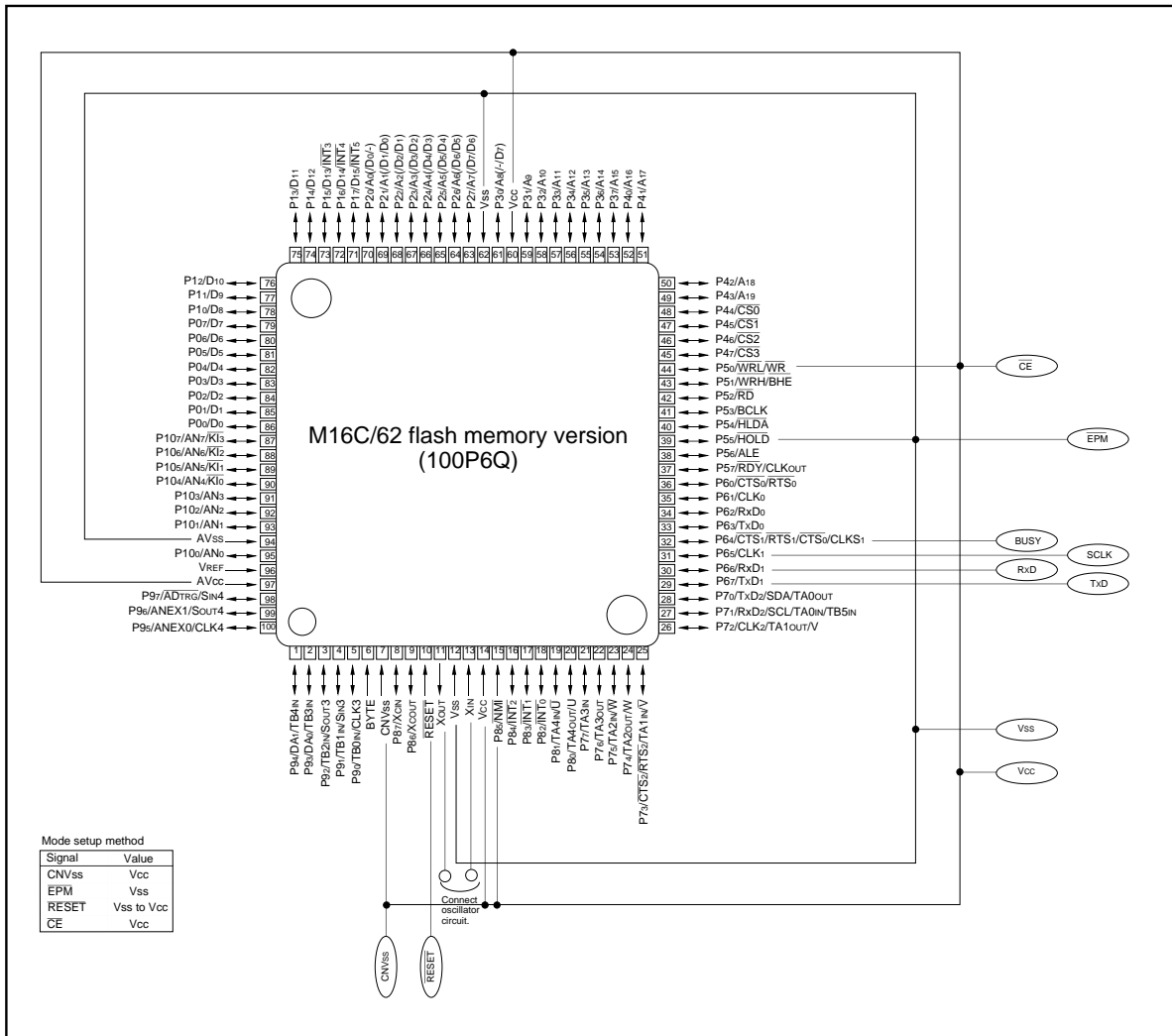
Figure 1.31.2. Pin connections for serial I/O mode (2)
