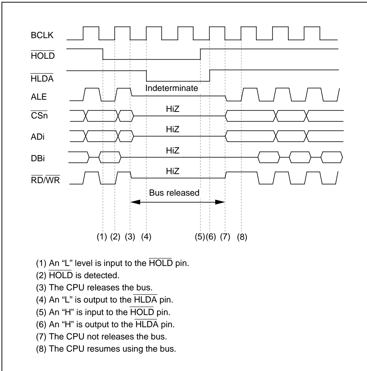
Figure 5.6.1. Example of releasing the external bus
