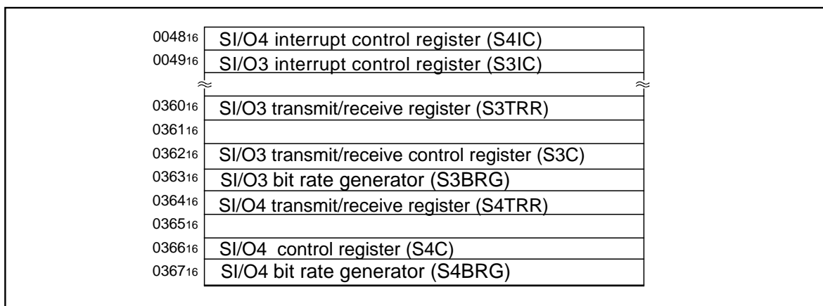
Figure 2.6.1. Memory map of serial I/O3, 4-related registers
