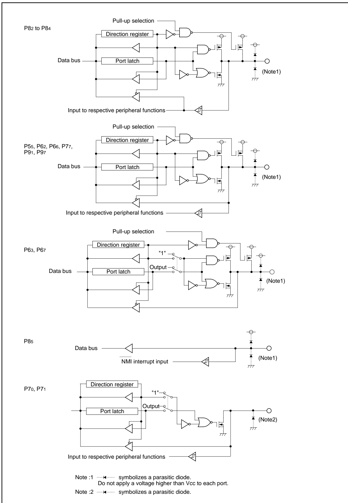
Figure 1.23.2. Programmable I/O ports (2)
