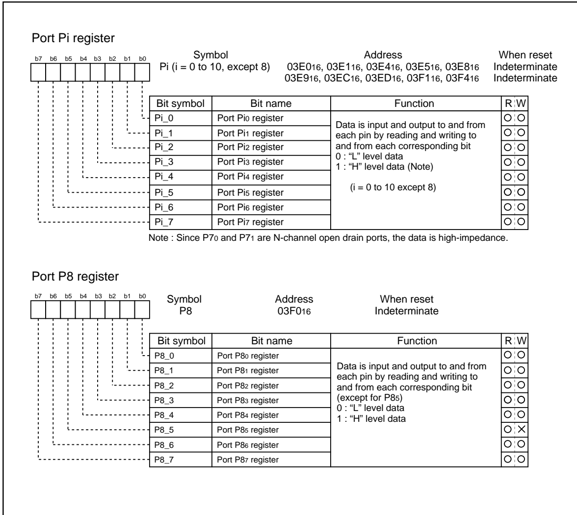
Figure 2.15.3. Programmable I/O ports-related registers (2)
