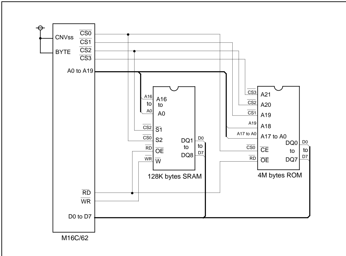
Figure 5.3.6. 4-Mbyte ROM and 128-Kbyte SRAM Connection Example
