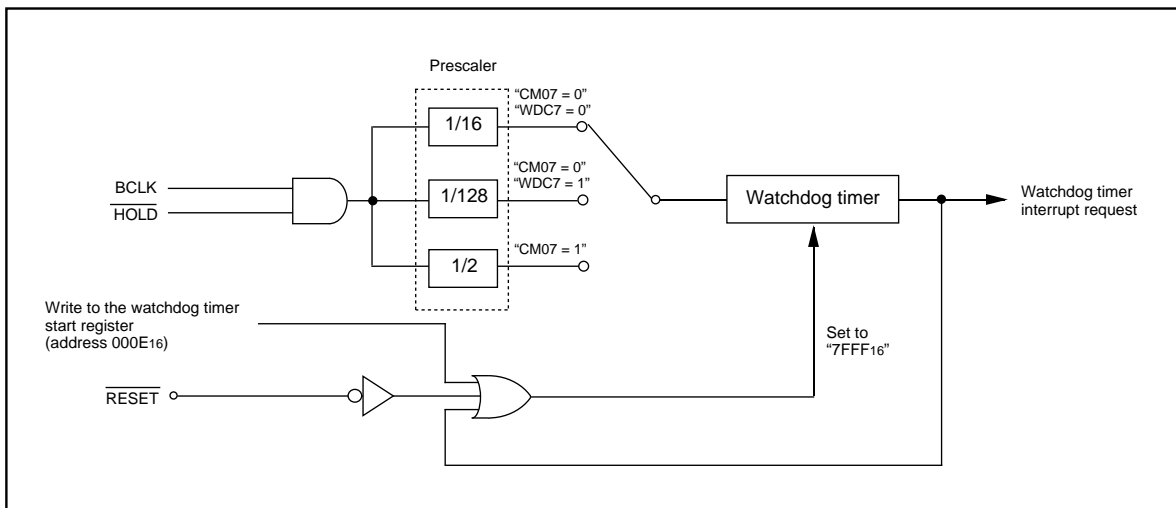
Figure 1.15.1. Block diagram of watchdog timer
