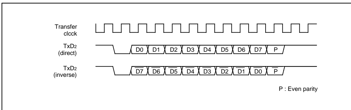
Figure 1.19.24. SIM interface format
