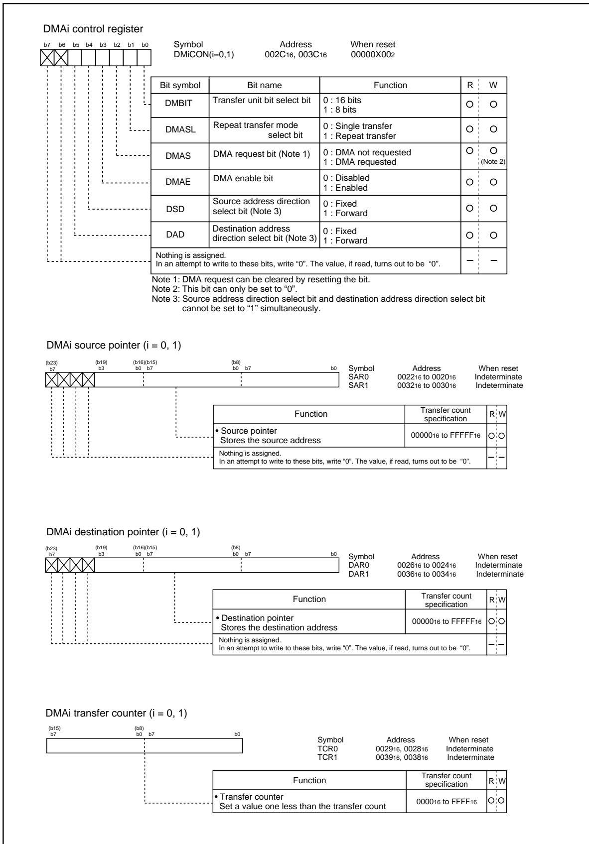
Figure 2.9.3. DMAC-related registers (2)
