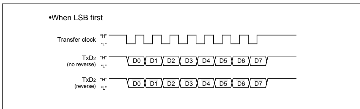
Figure 1.19.14. Serial data logic switch timing
