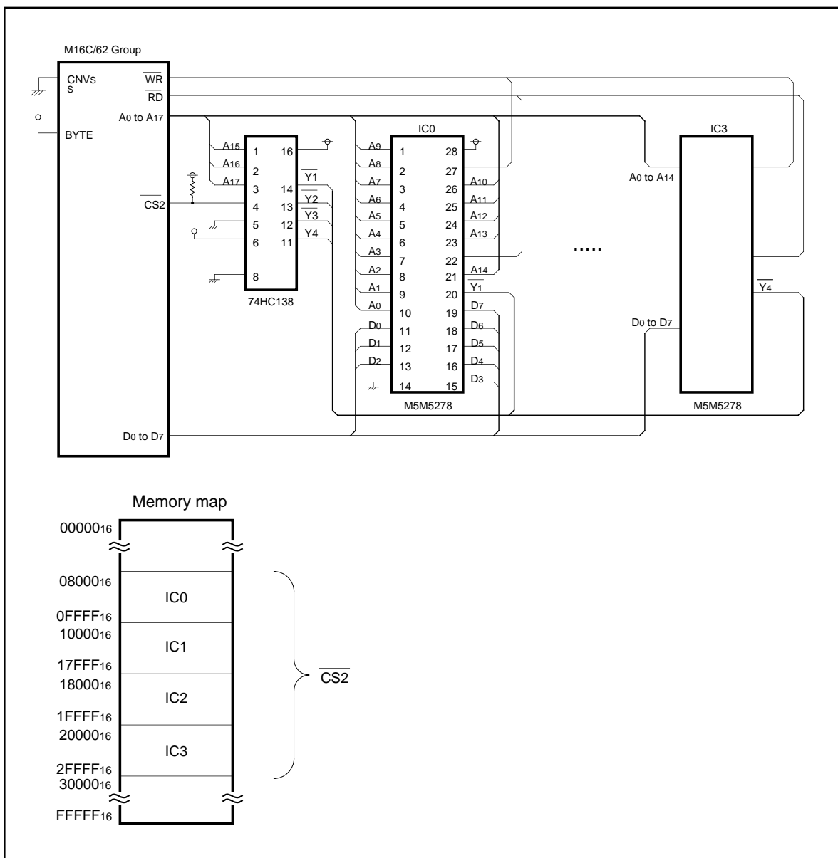
Figure 5.4.9. Chip selects and address bus
