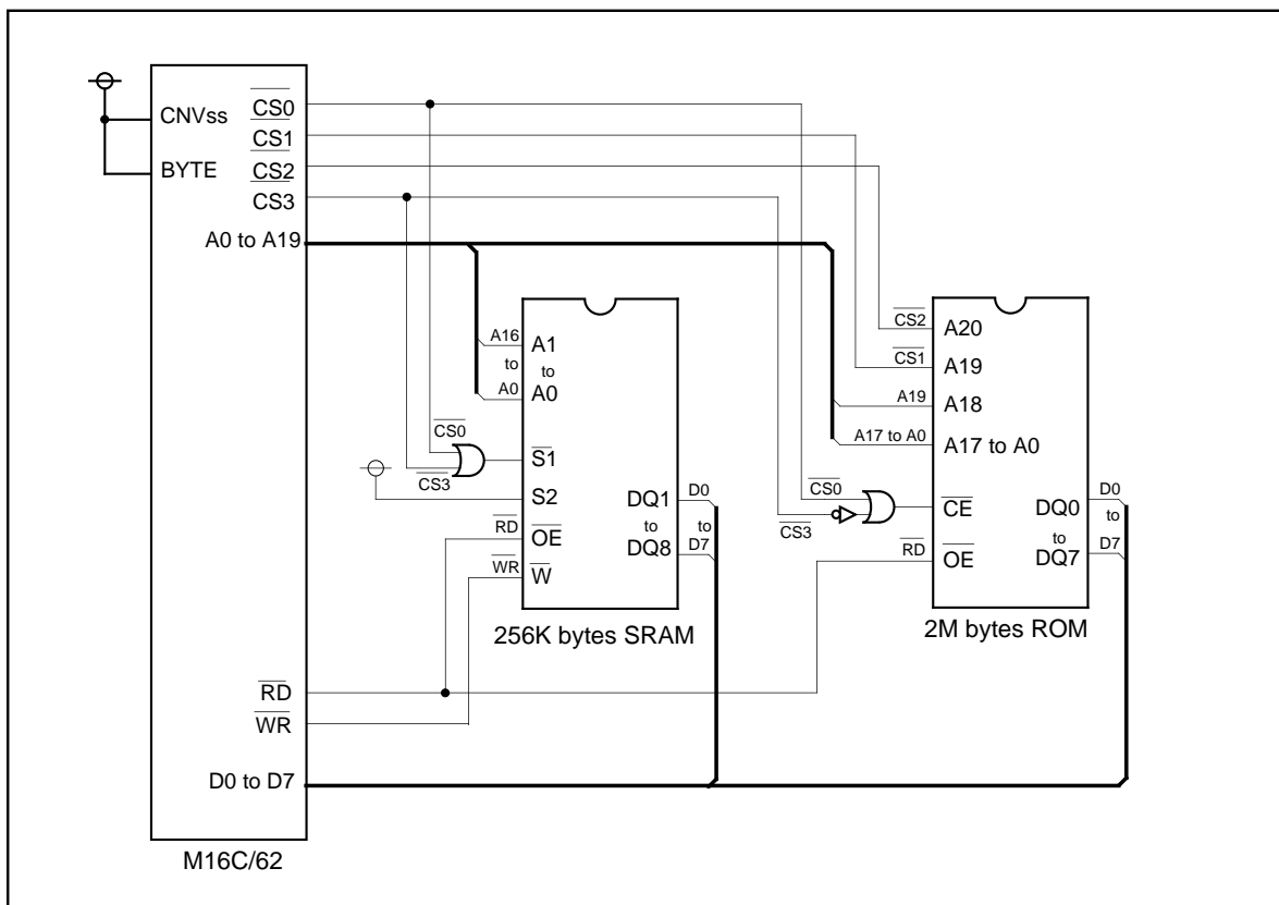
Figure 5.3.8. 2-Mbyte ROM and 256-Kbyte SRAM Connection Example
