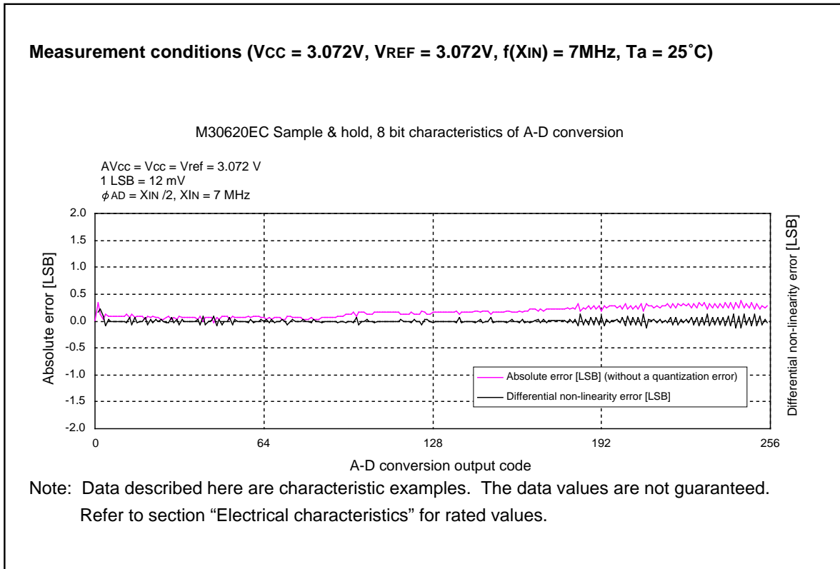
Figure 7.2.2. Standard characteristics of the A-D converter
