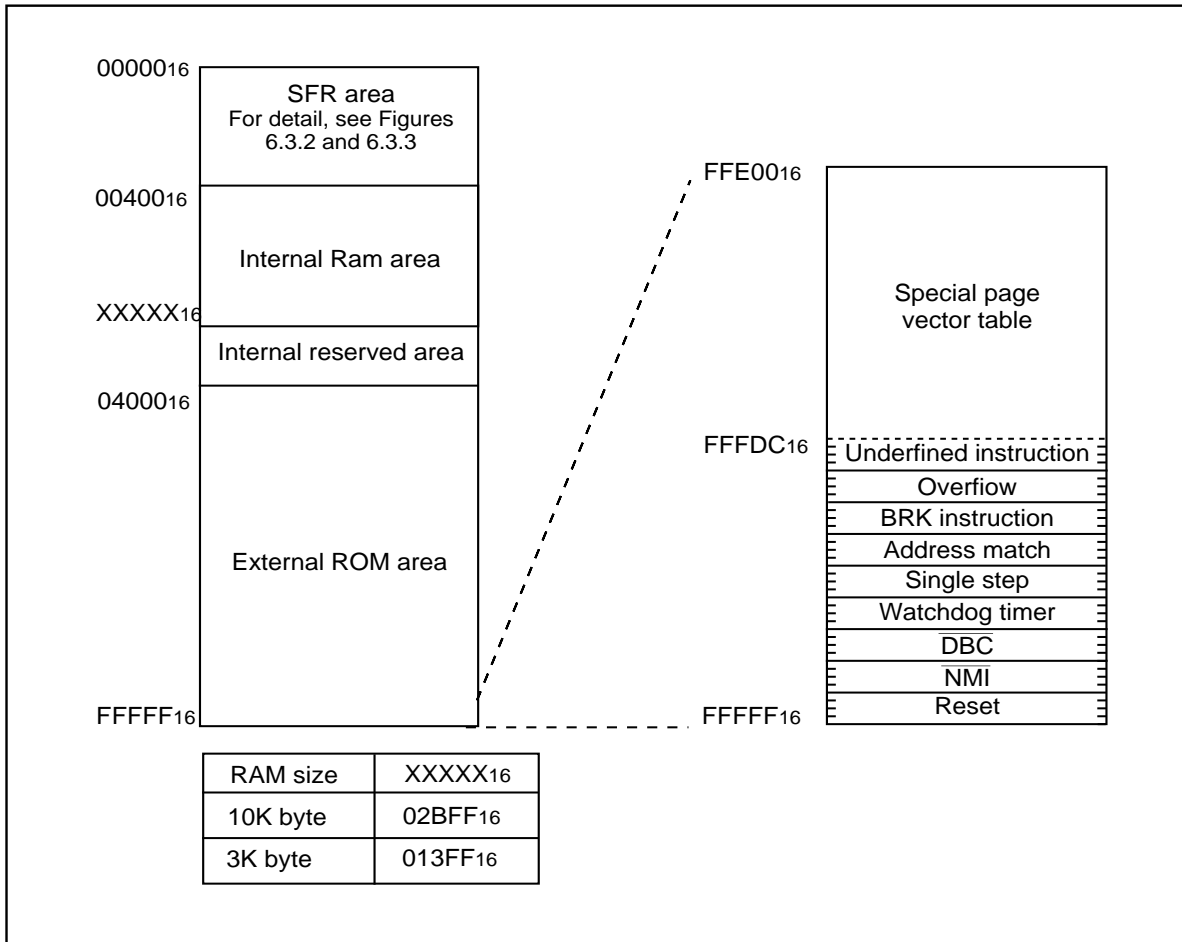
Figure 6.3.1. Memory map
