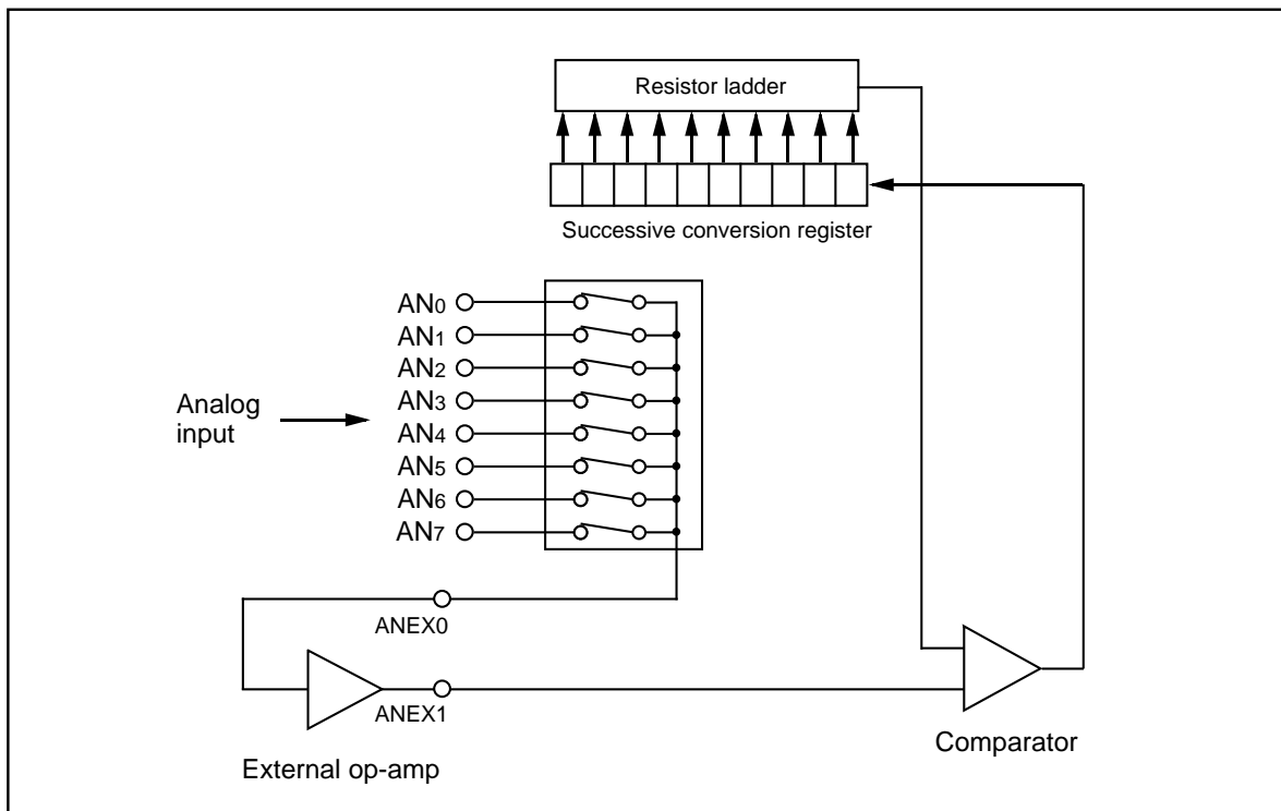
Figure 1.20.9. Example of external op-amp connection mode
