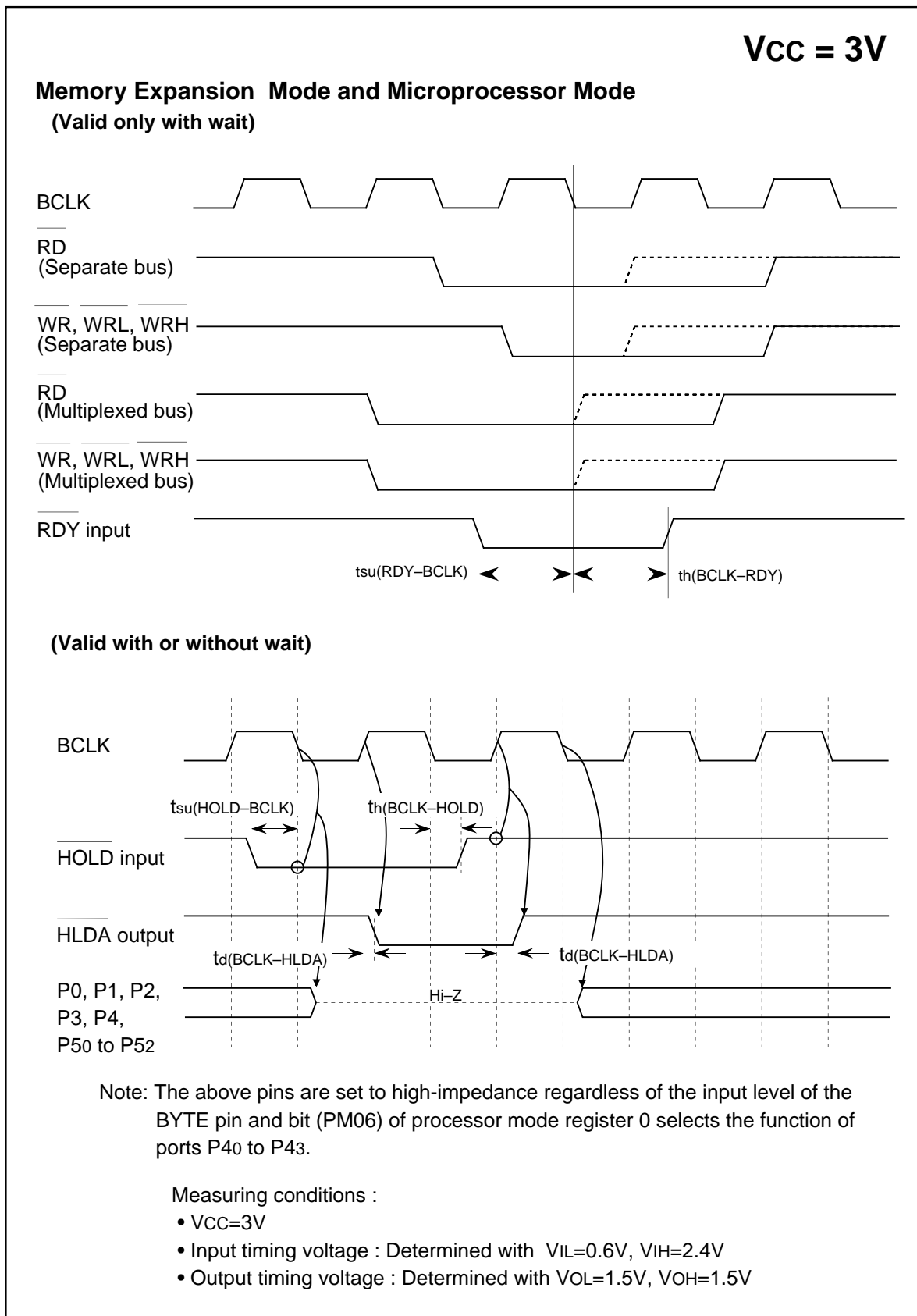
Figure 1.26.8. V_{CC}=3V timing diagram (2)
