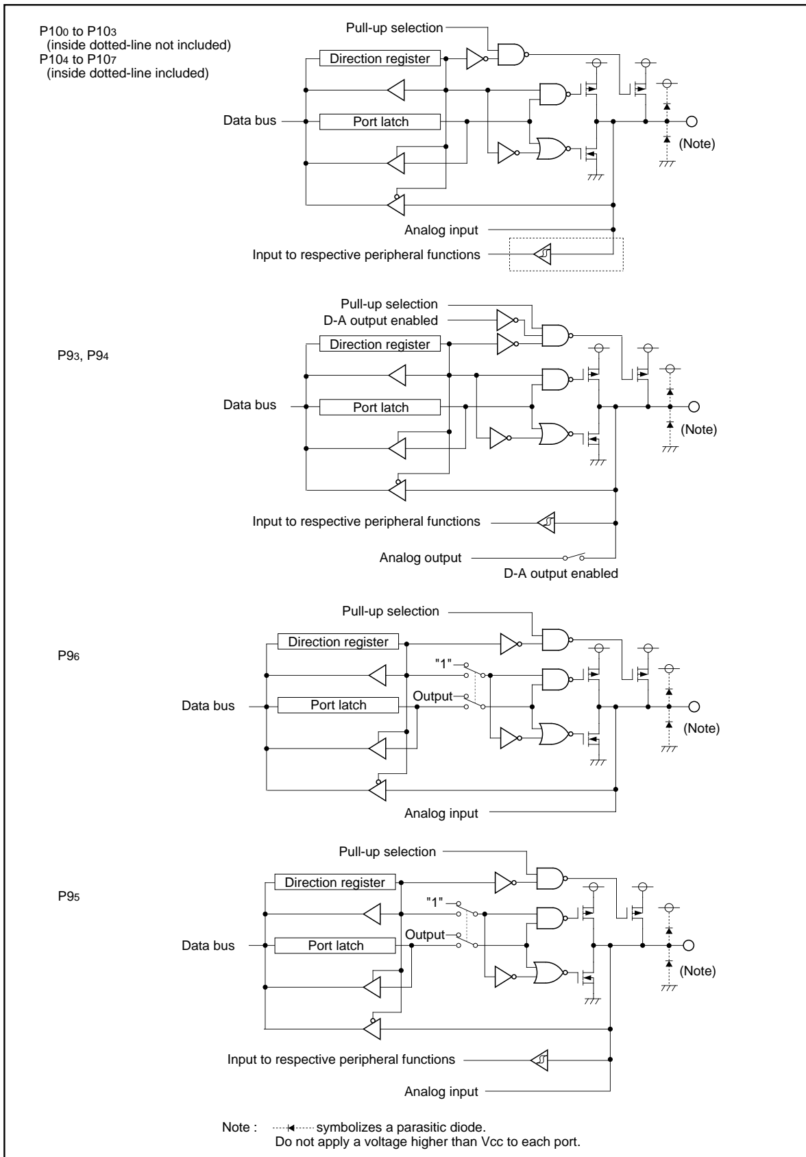
Figure 1.23.3. Programmable I/O ports (3)
