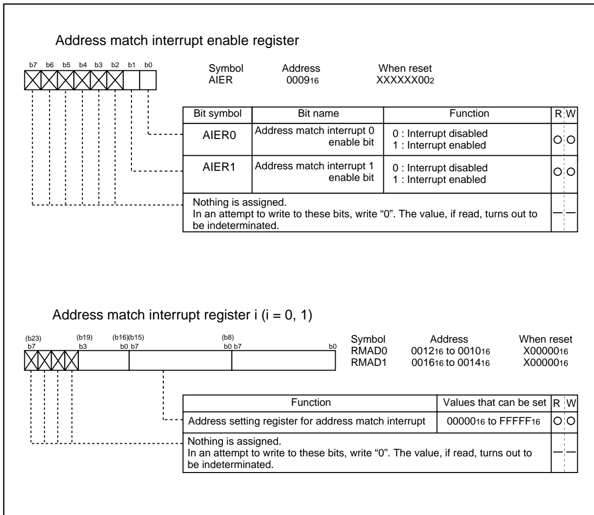
Figure 1.14.12. Address match interrupt-related registers
