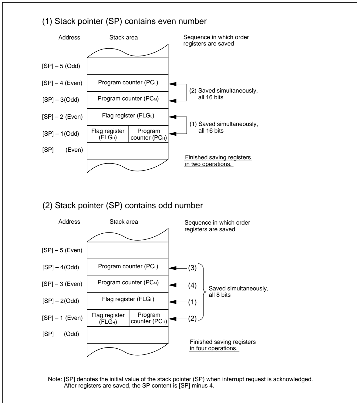
Figure 1.14.7. Operation of saving registers
