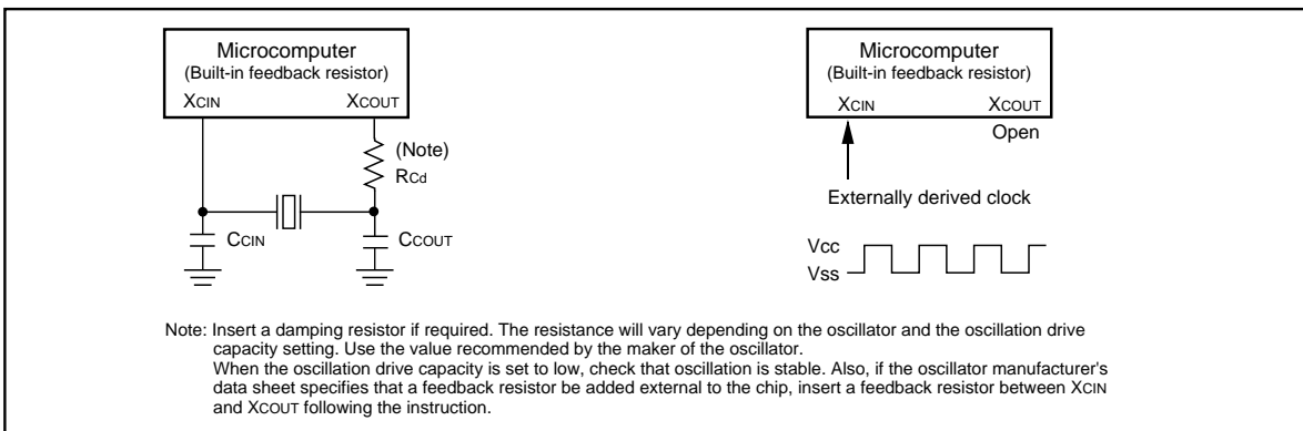
Figure 1.13.2. Examples of sub-clock
