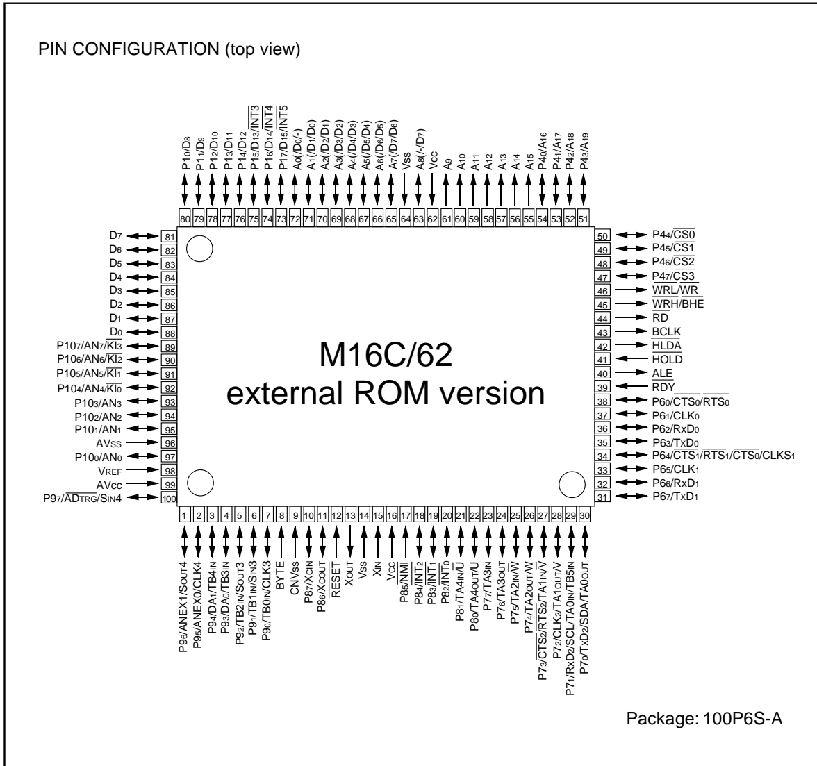
Figure 6.1.1. Pin configuration (top view)
