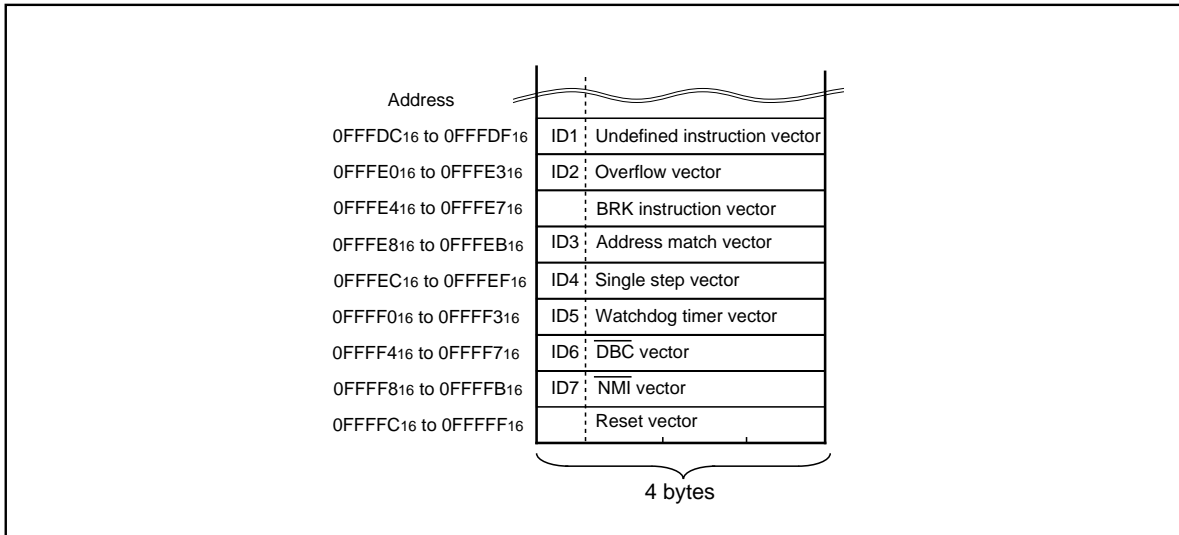
Figure 1.29.10. ID code store addresses
