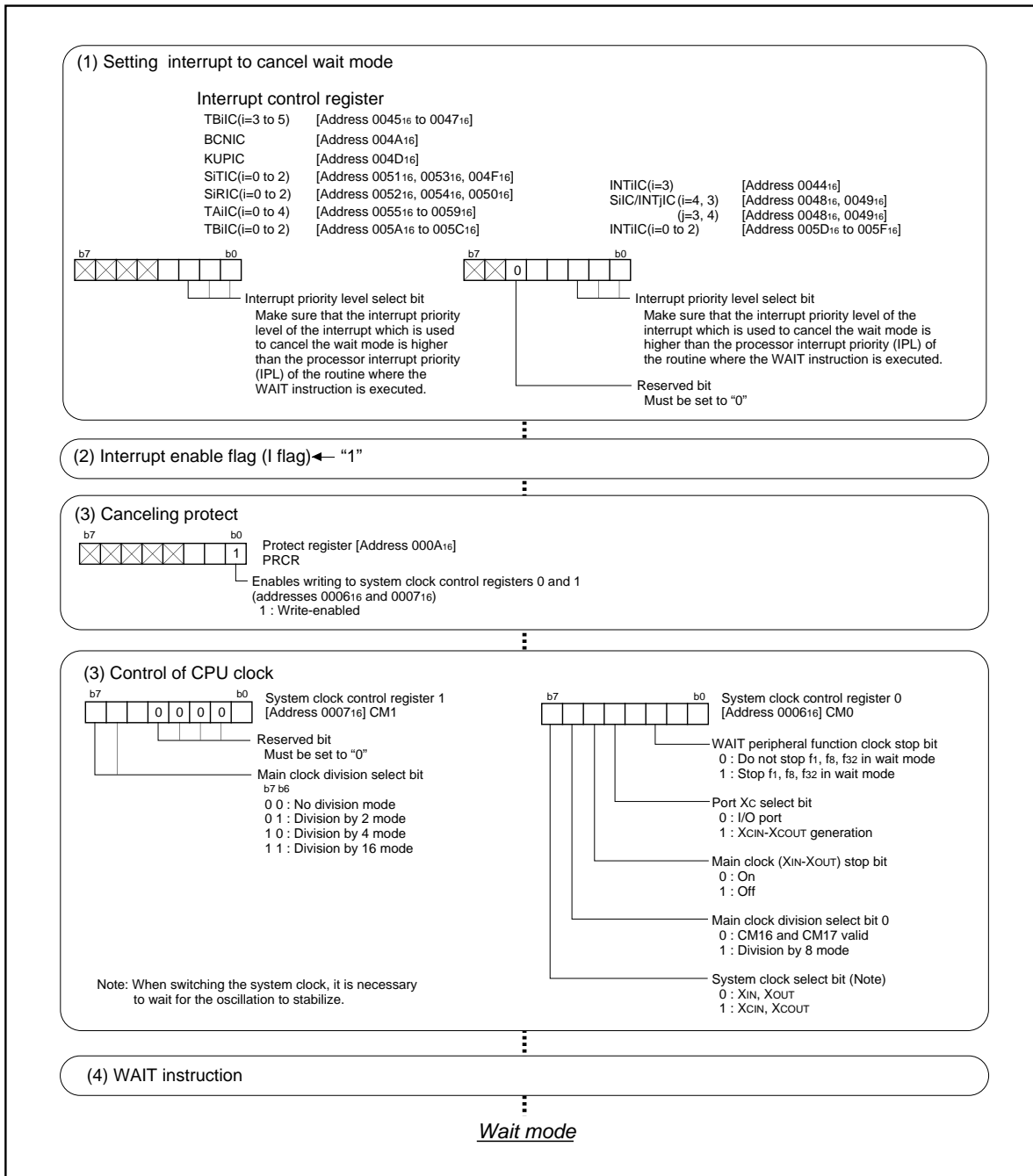
Figure 2.14.6. Example of wait mode set-up
