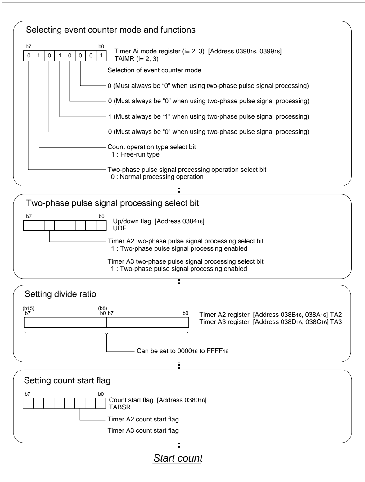
Figure 2.2.17. Set-up procedure of 2-phase pulse signal process in event counter mode, normal mode selected
