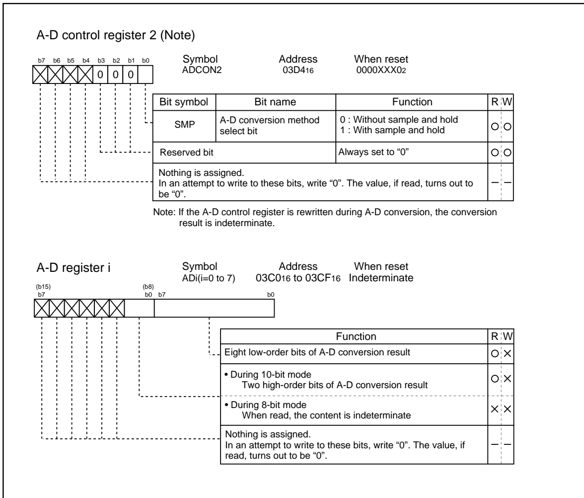
Figure 1.20.3. A-D converter-related registers (2)
