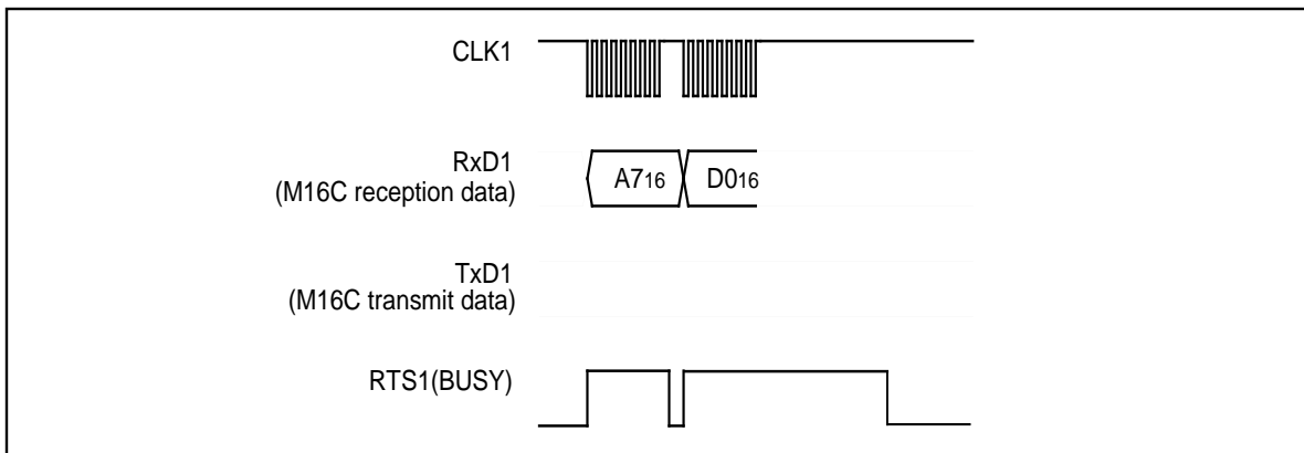
Figure 1.31.8. Timing for erasing all unlocked blocks
