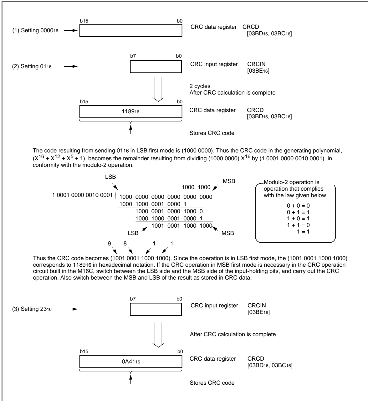
Figure 1.22.3. Calculation example using the CRC calculation circuit
