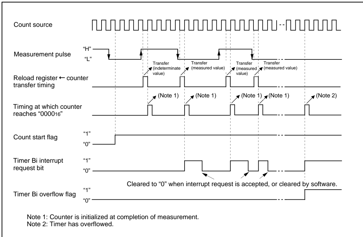
Figure 1.17.21. Operation timing when measuring a pulse width
