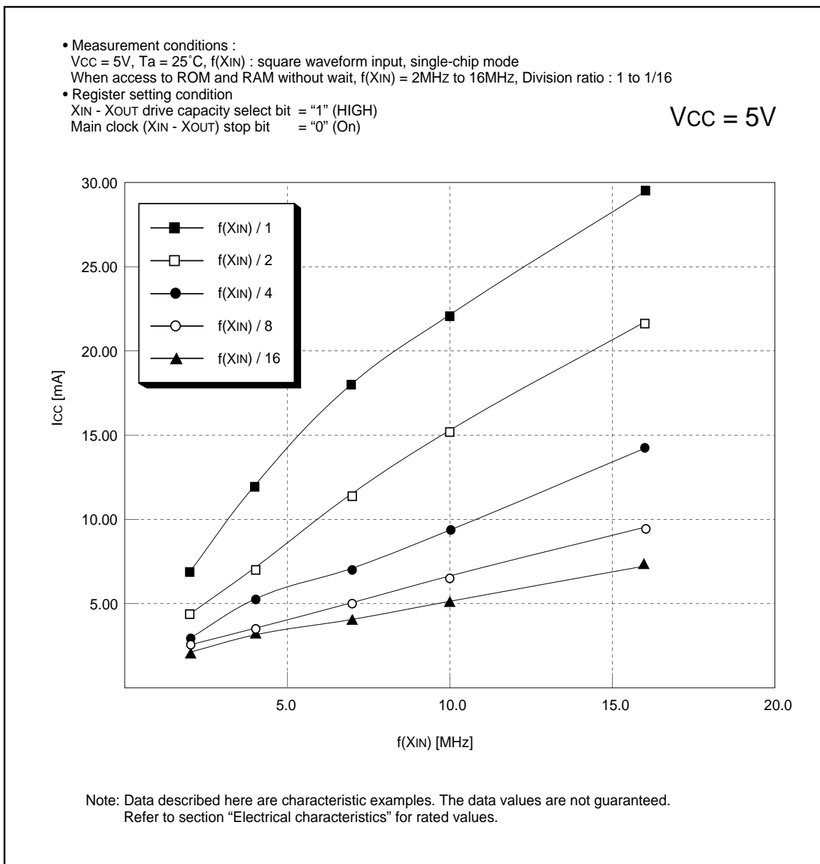
Figure 7.1.5. Standard characteristics of I_{CC} - f(XIN) (VCC = 5V)
