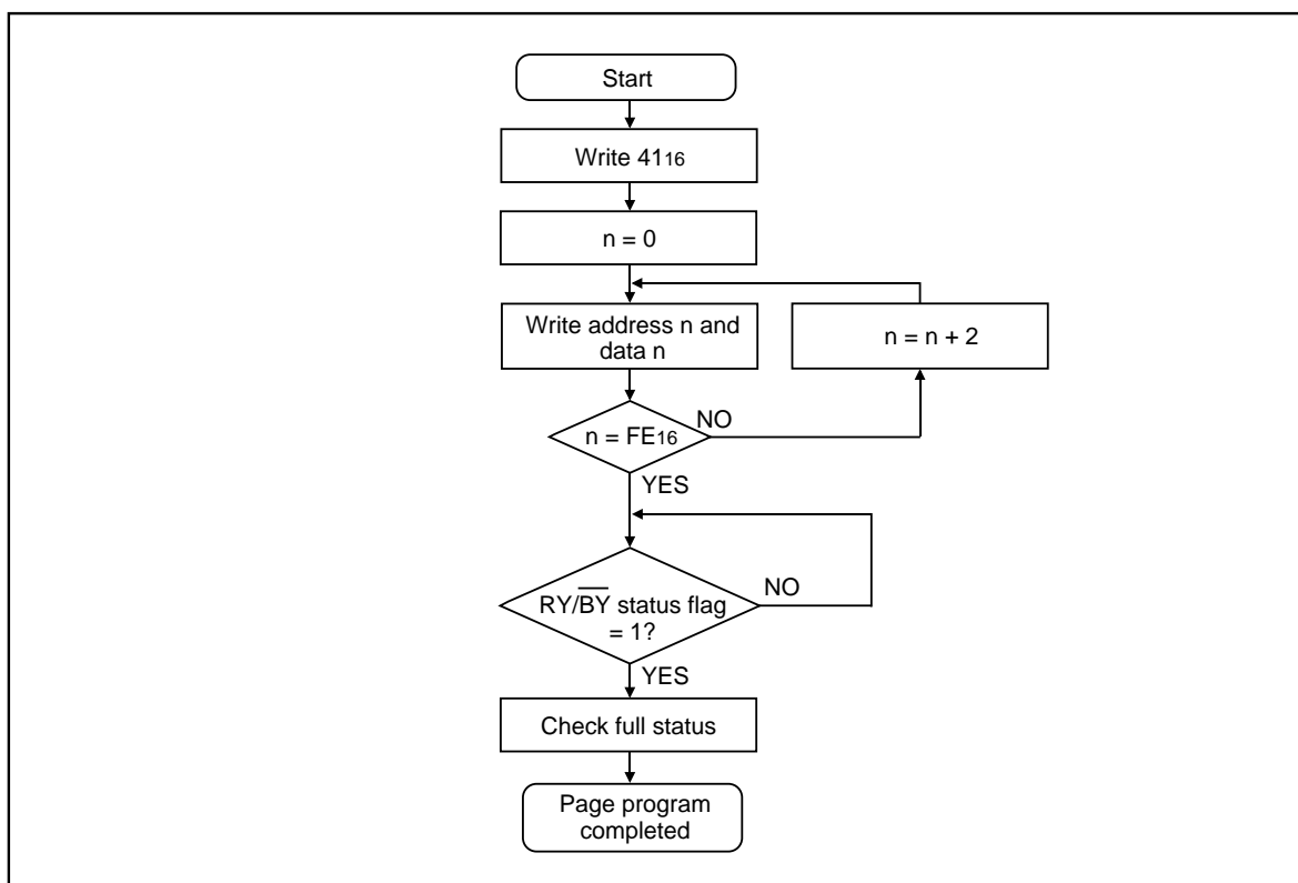
Figure 1.29.4. Page program flowchart
