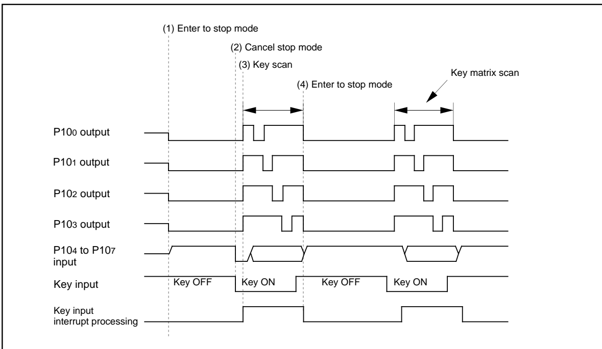
Figure 2.13.4. Example of operation of key-input interrupt
