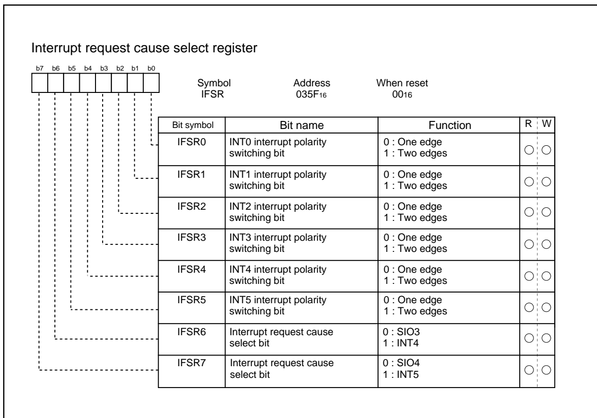
Figure 1.14.10. Interrupt request cause select register
