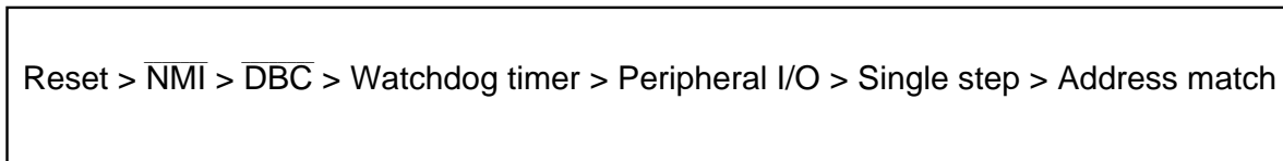
Figure 4.5.2. Hardware interrupts priorities
