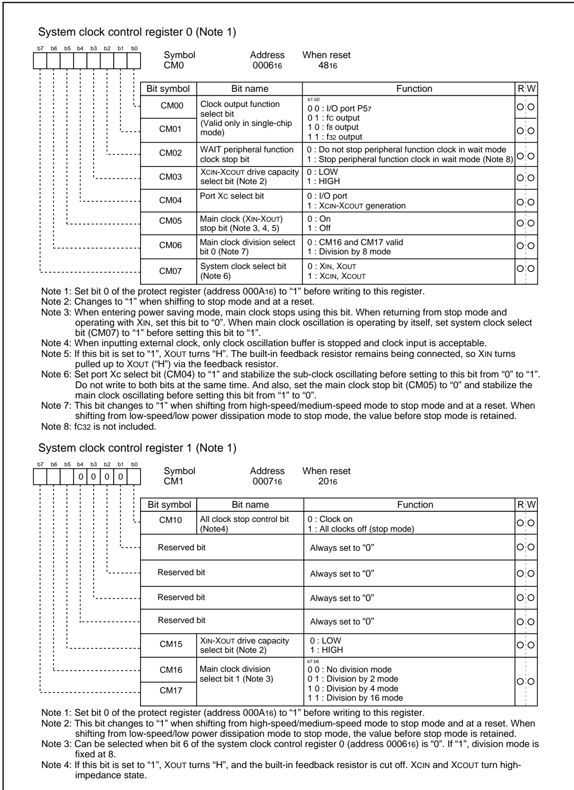
Figure 1.13.4. Clock control registers 0 and 1
