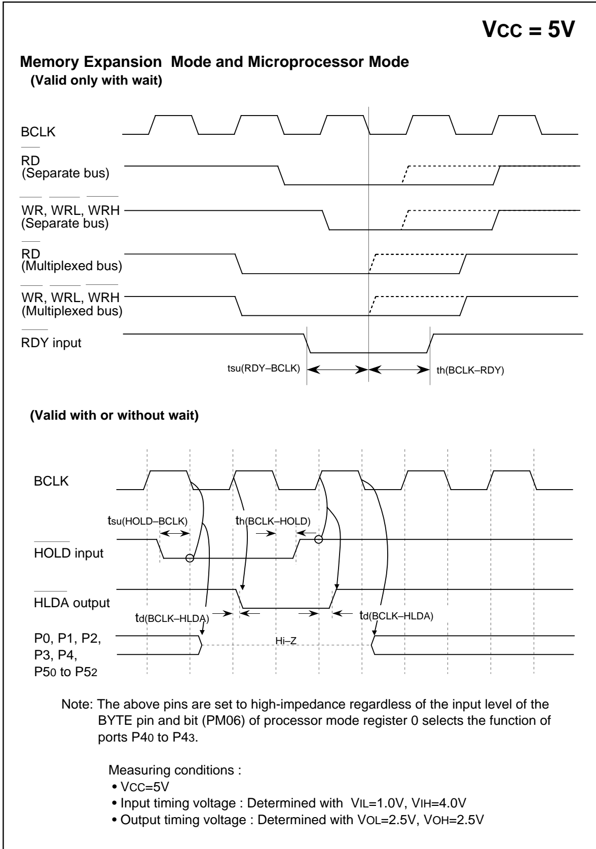
Figure 1.26.3. Vcc=5V timing diagram (2)
