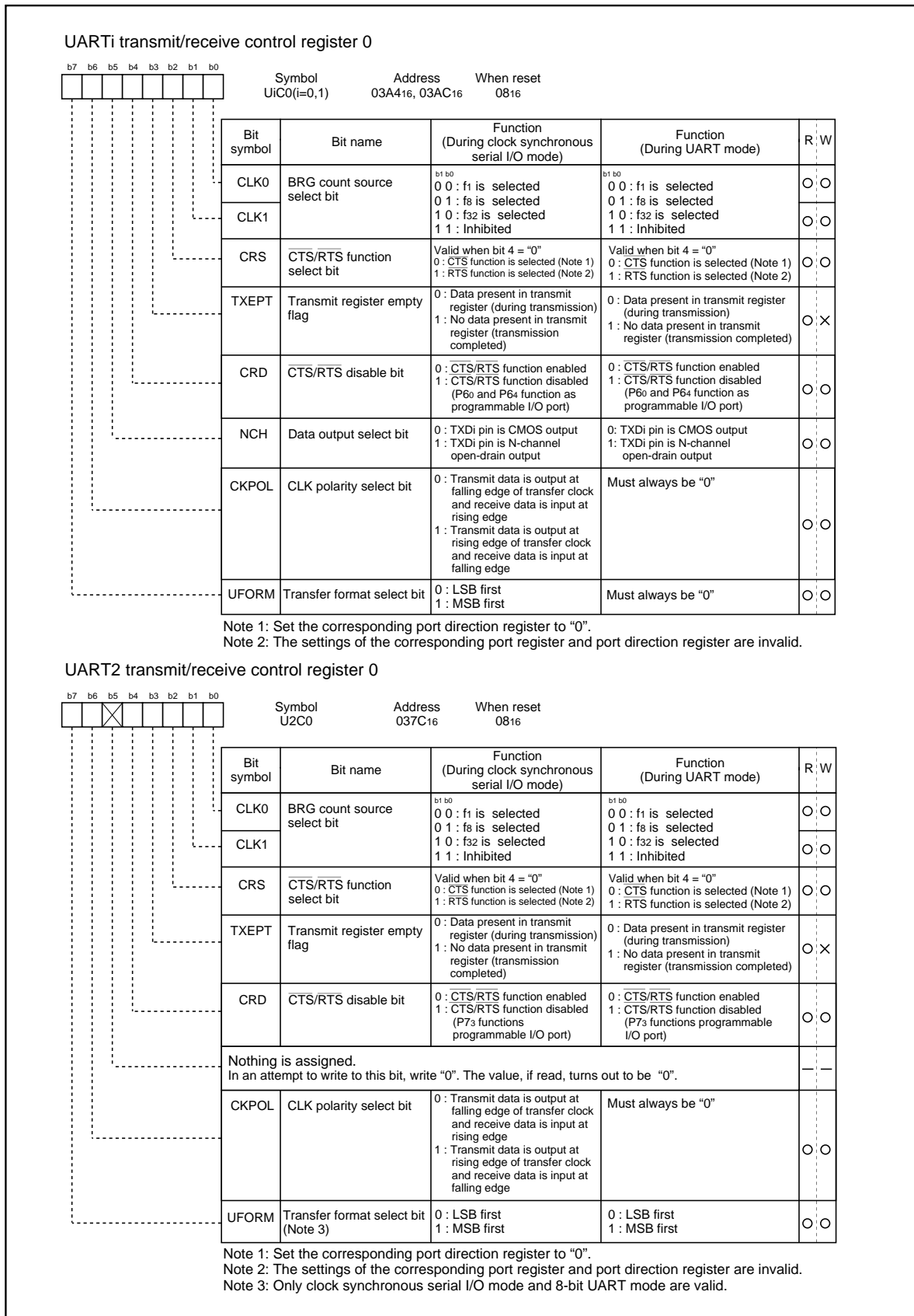
Figure 1.19.6. Serial I/O-related registers (3)
