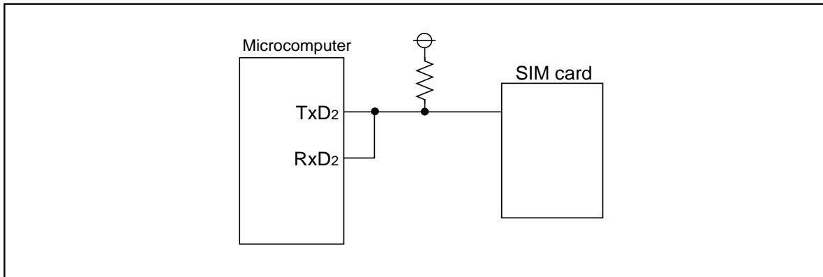
Figure 1.19.25. Connecting the SIM interface
