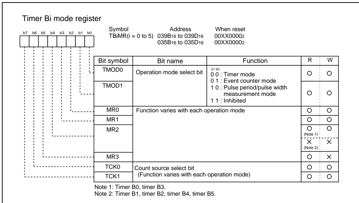
Figure 1.17.15. Timer B-related registers (1)
