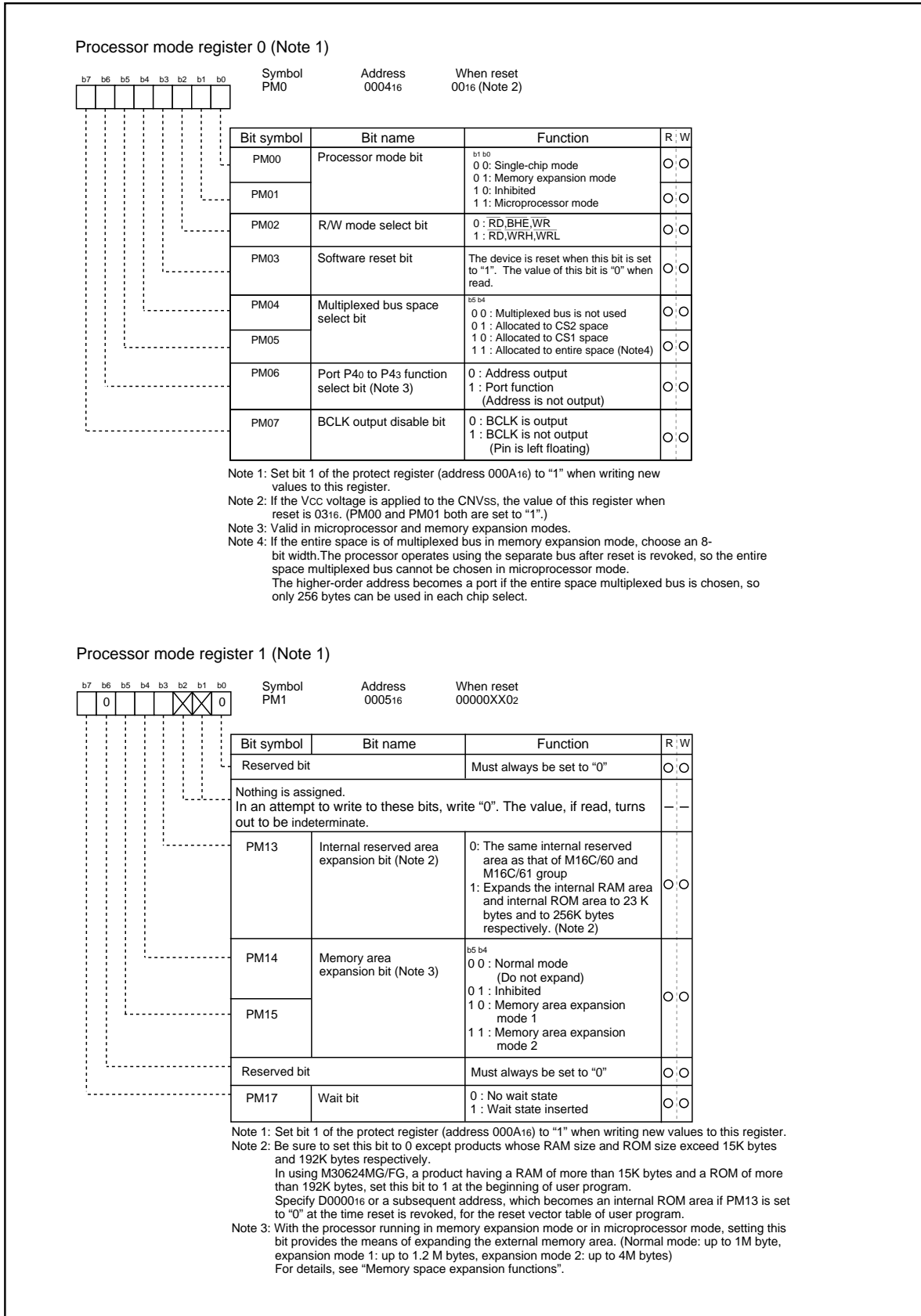
Figure 1.9.1. Processor mode register 0 and 1
