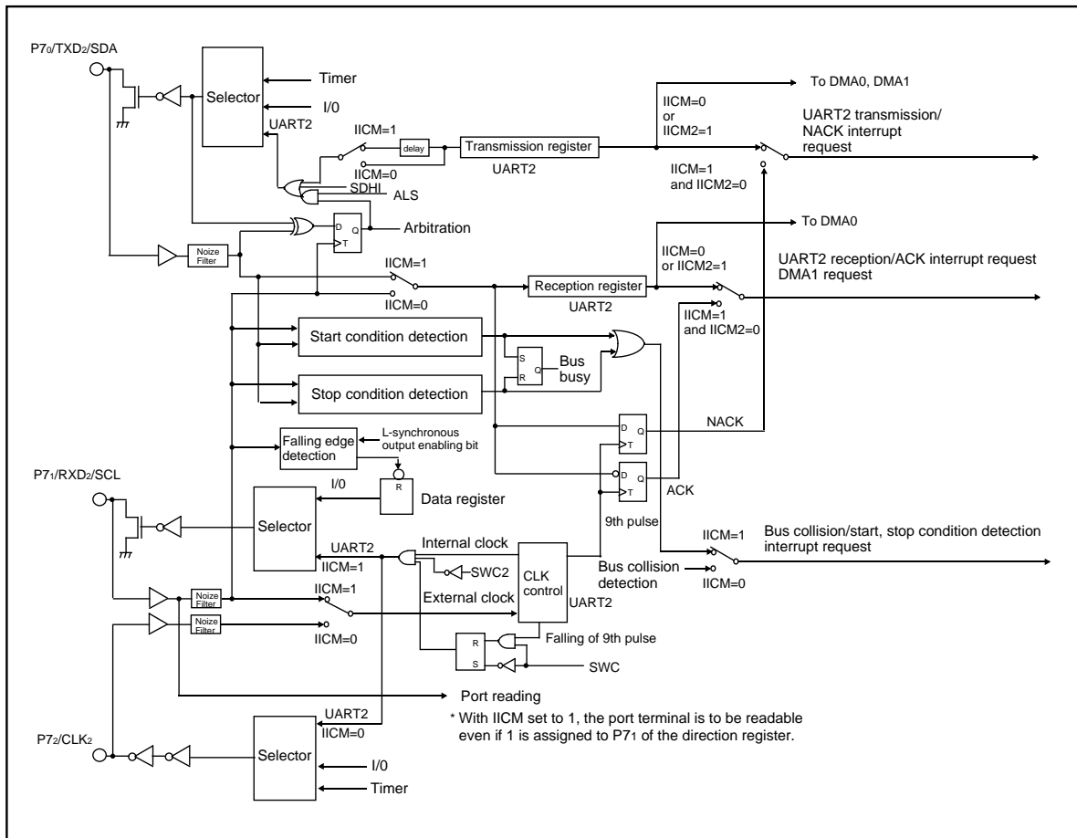
Figure 1.19.30. Functional block diagram for I 2 C mode
