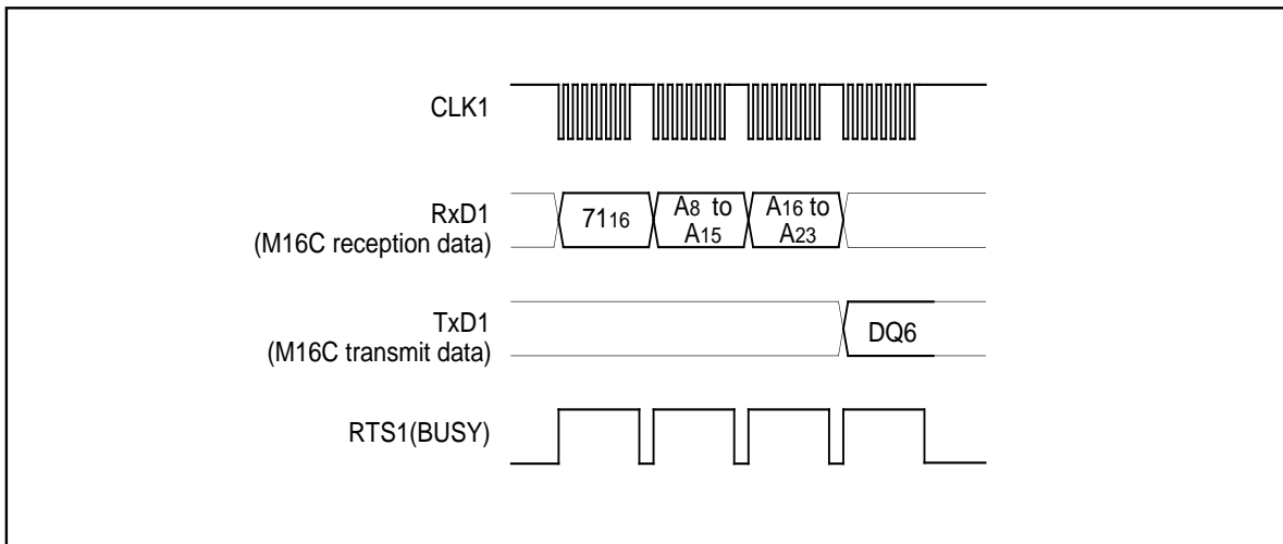
Figure 1.31.10. Timing for reading lock bit status
