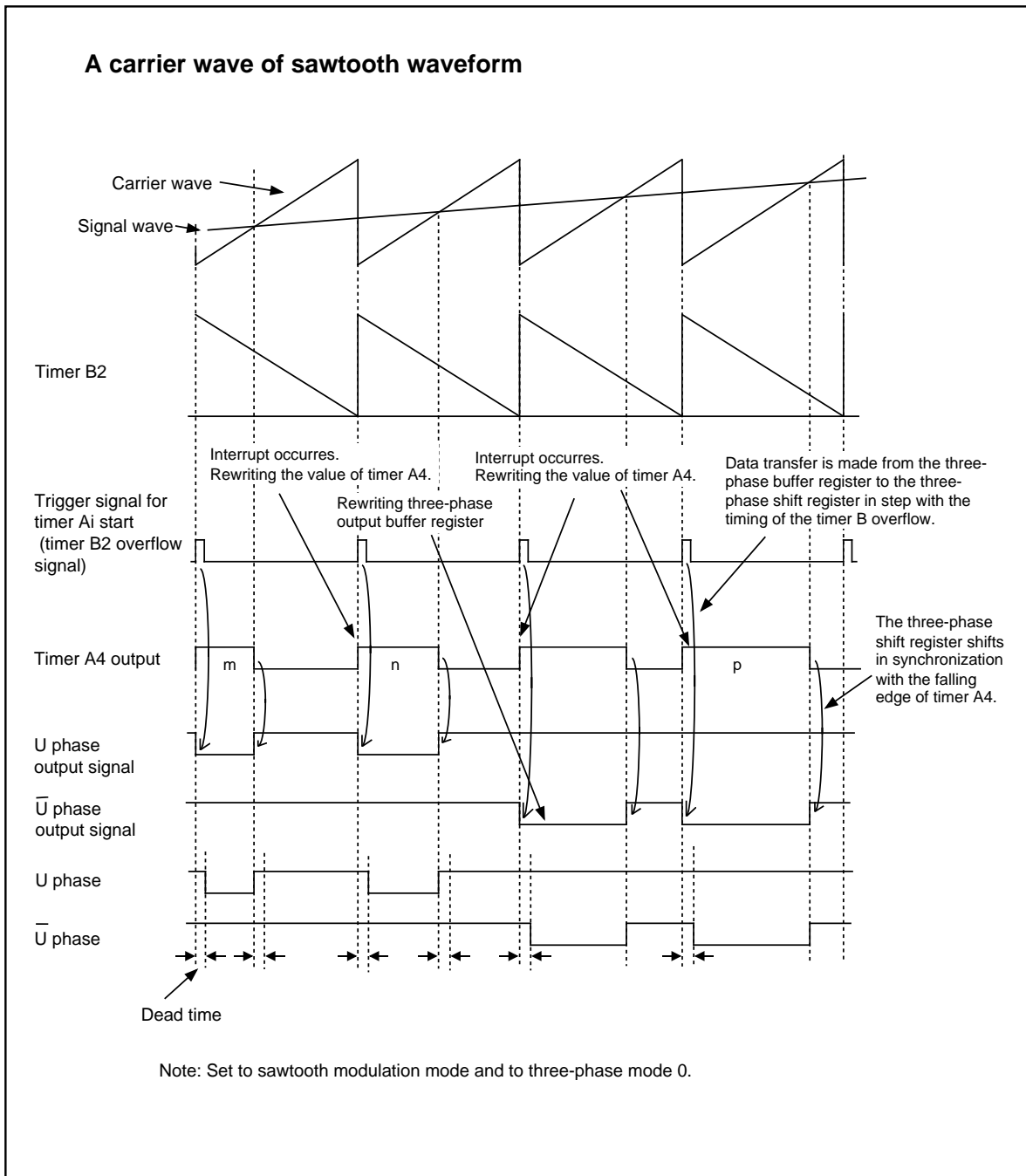
Figure 1.18.9. Timing chart of operation (4)
