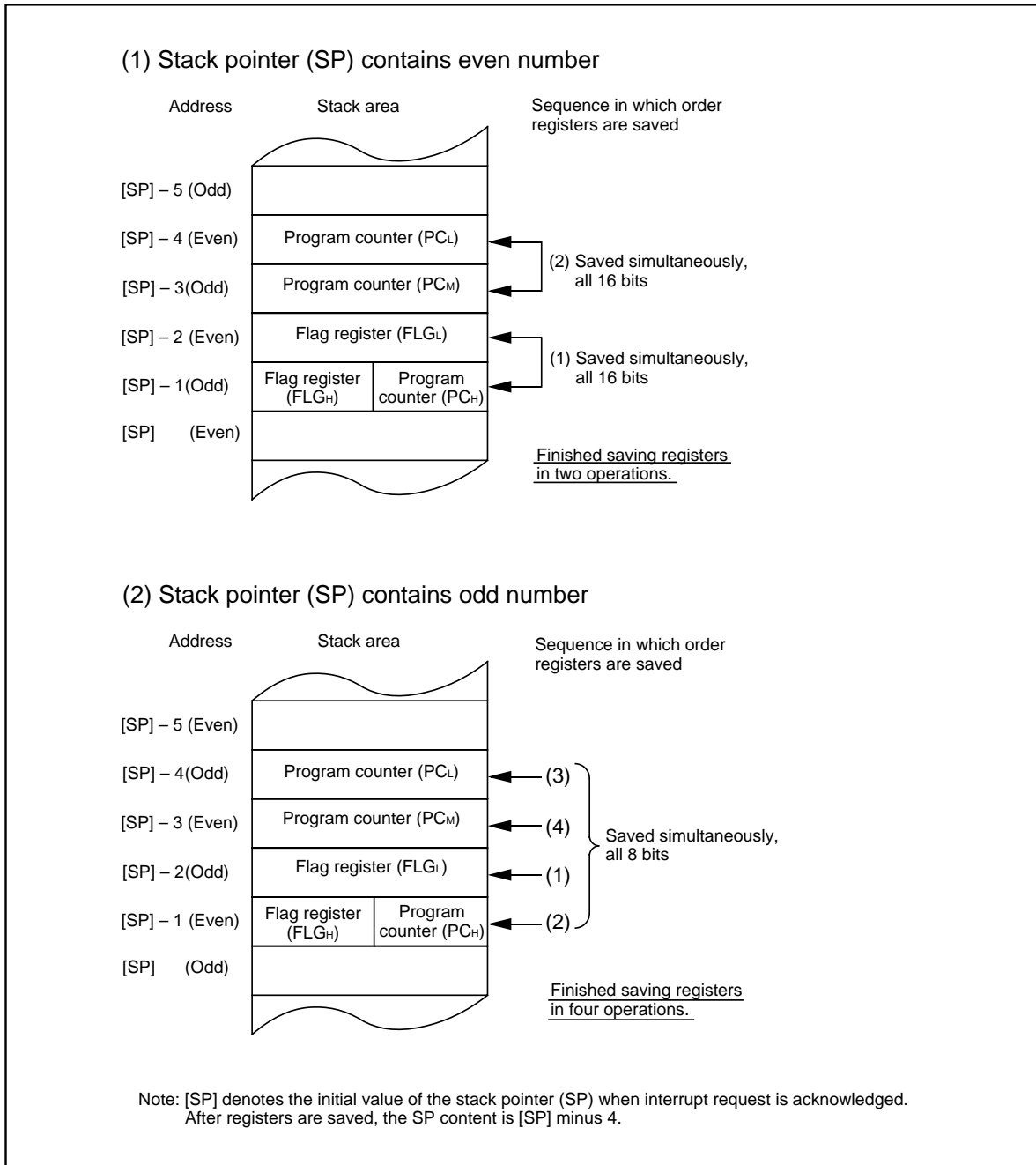
Figure 4.3.4. Operation of saving registers
