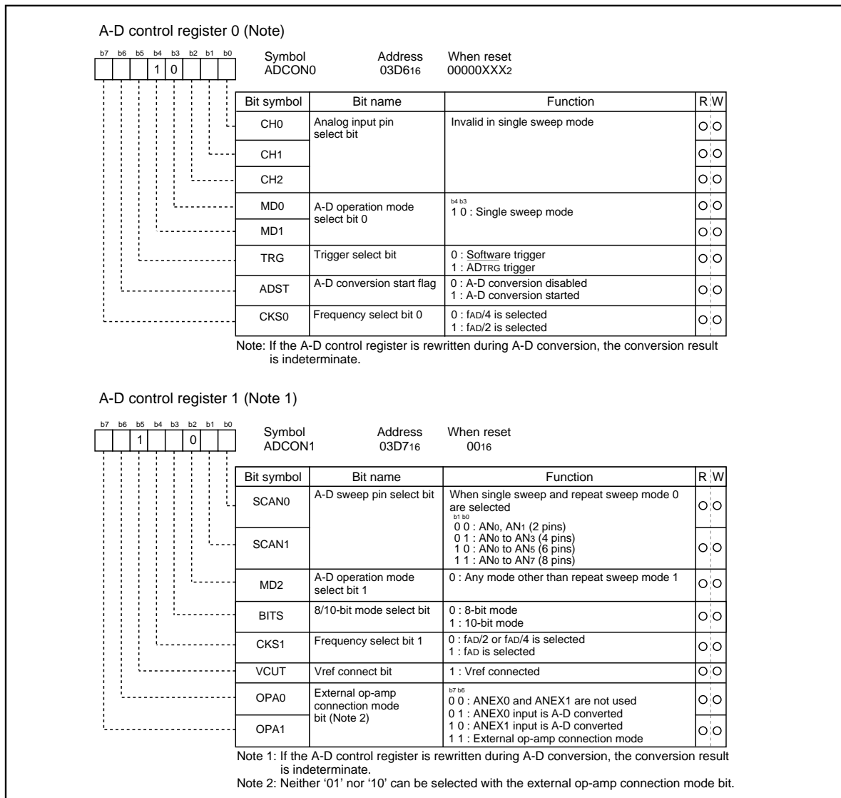
Figure 1.20.6. A-D conversion register in single sweep mode
