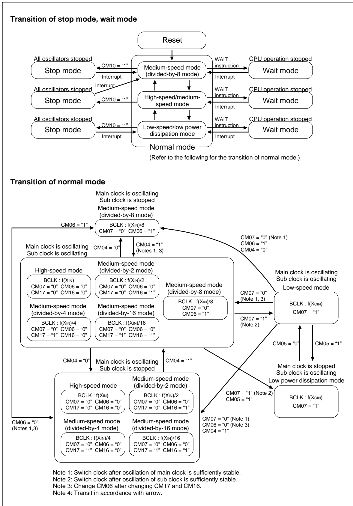
Figure 2.14.1. State transition diagram of power control mode
