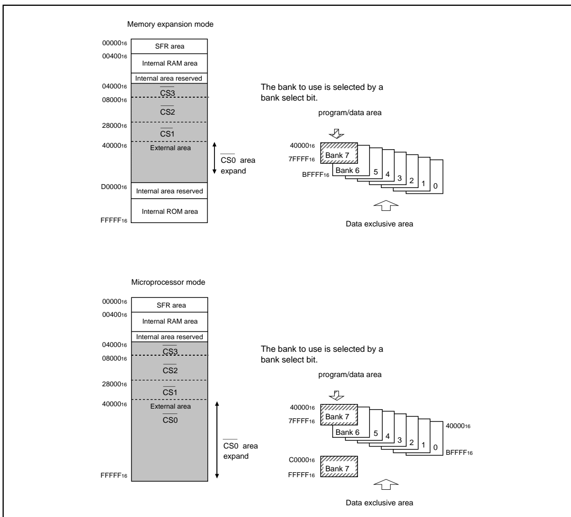
Figure 5.3.4. Memory Map in Memory space expansion mode 2
