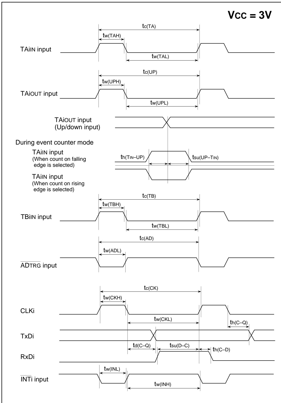
Figure 1.26.7. V_{CC}=3V timing diagram (1)
