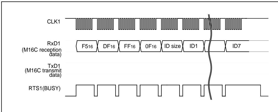
Figure 1.31.16. Timing for the ID check
