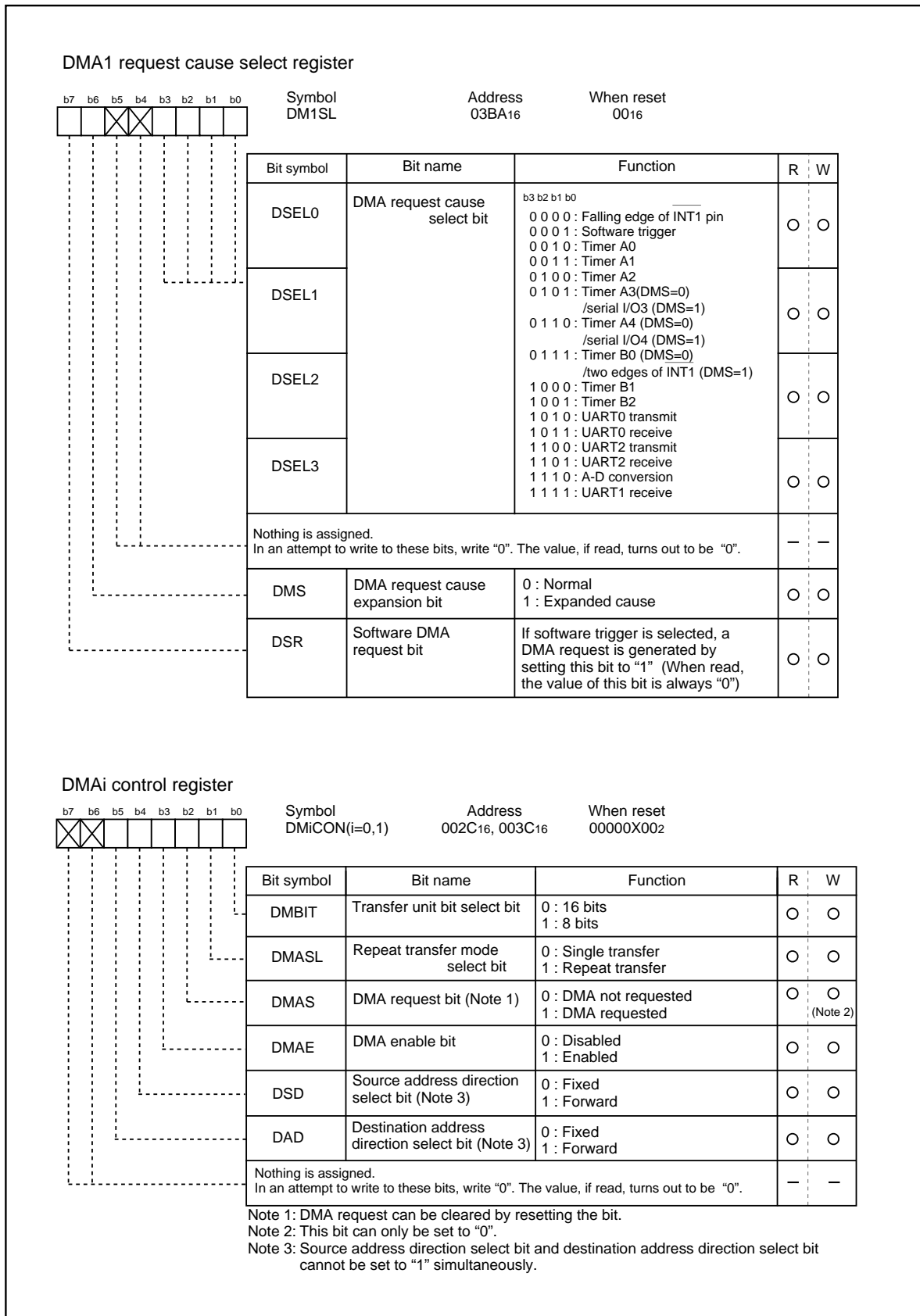
Figure 1.16.3. DMAC register (2)
