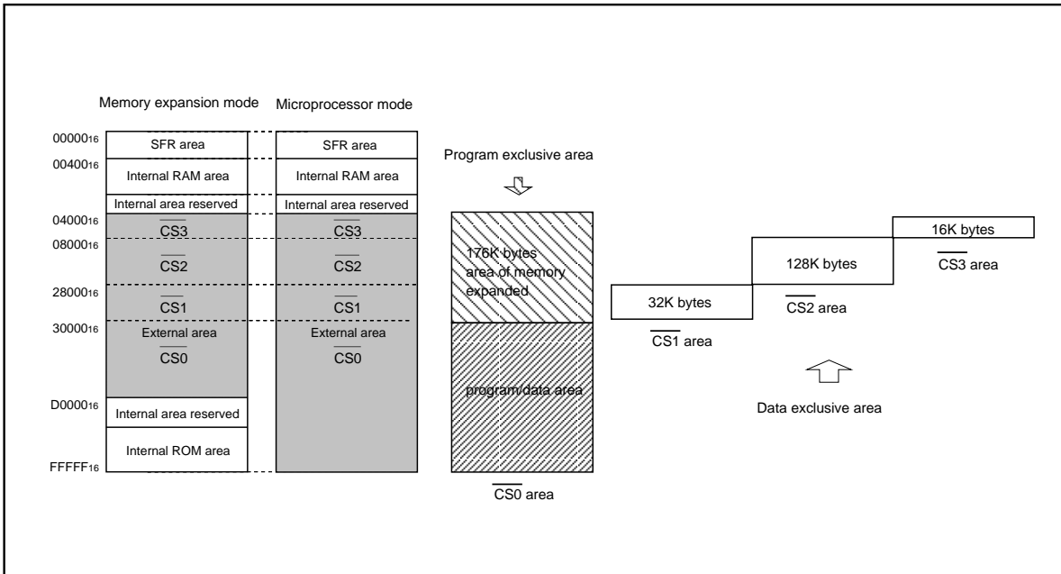
Figure 5.3.3. Memory Map in Memory space expansion mode 1
