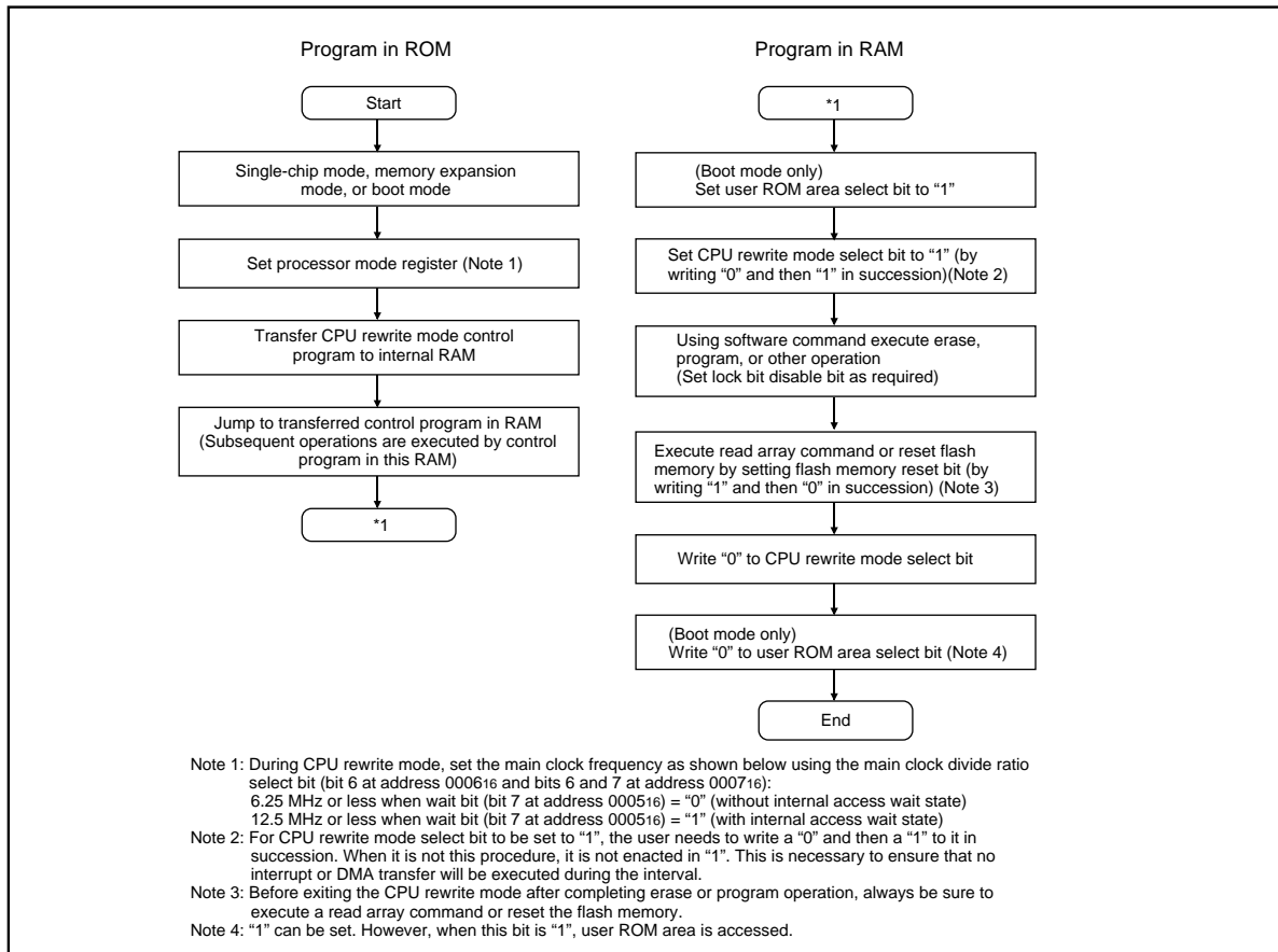
Figure 1.29.2. CPU Rewrite Mode Set/Reset Flowchart
