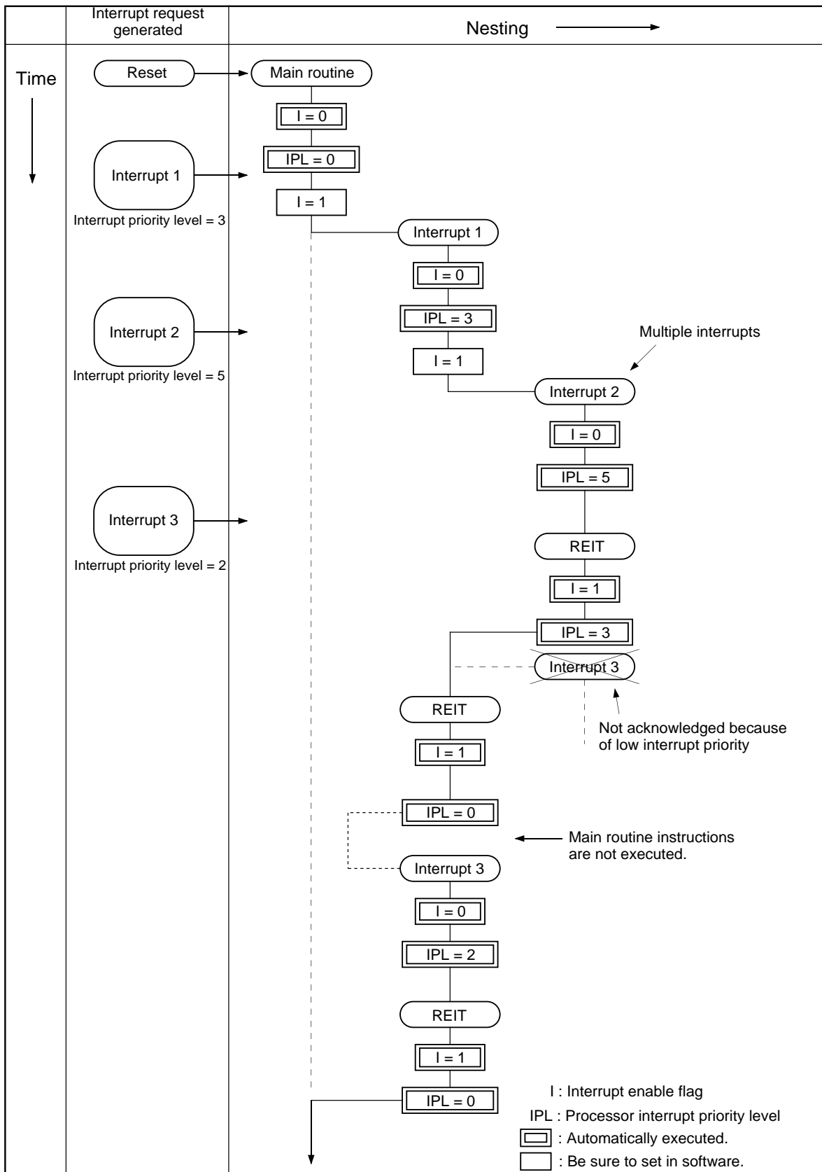
Figure 4.6.1. Multiple interrupts
