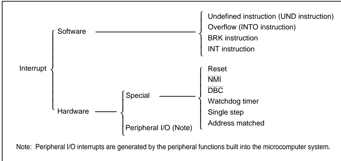
Figure 4.1.1. Classification of interrupts
