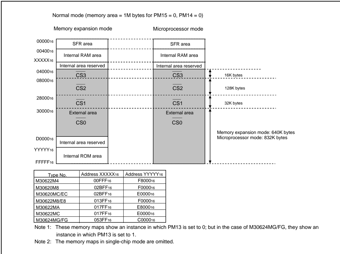
Figure 5.3.2. Memory Map in Nomal Mode
