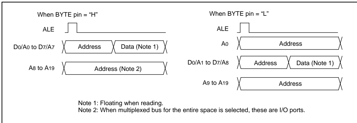
Figure 1.12.2. ALE signal and address/data bus
