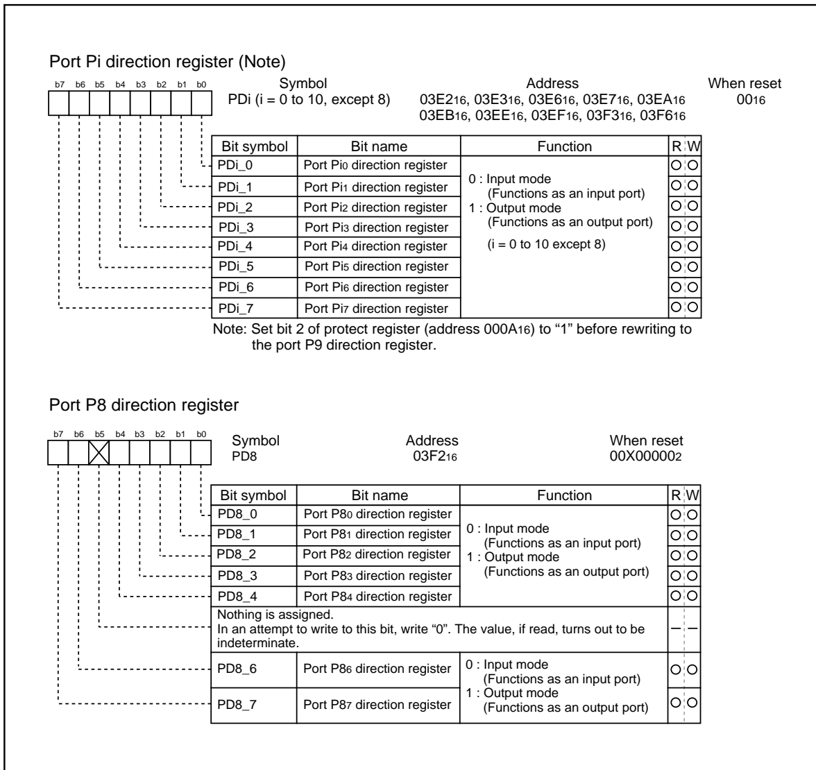
Figure 2.15.2. Programmable I/O ports-related registers (1)
