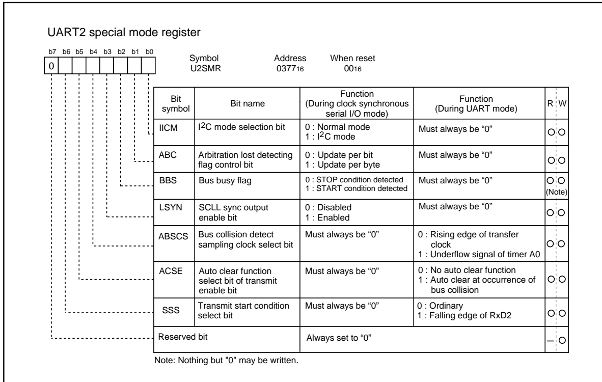
Figure 1.19.26. UART2 special mode register
