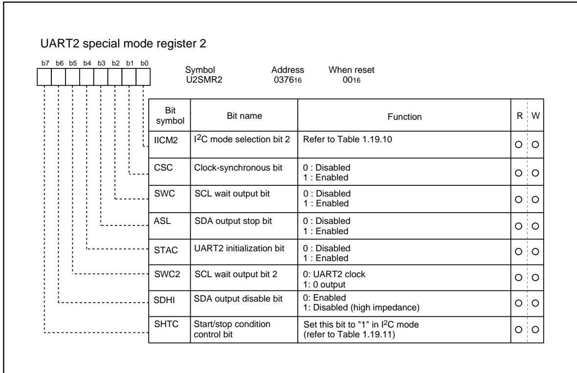
Figure 1.19.29. UART2 special mode register 2
