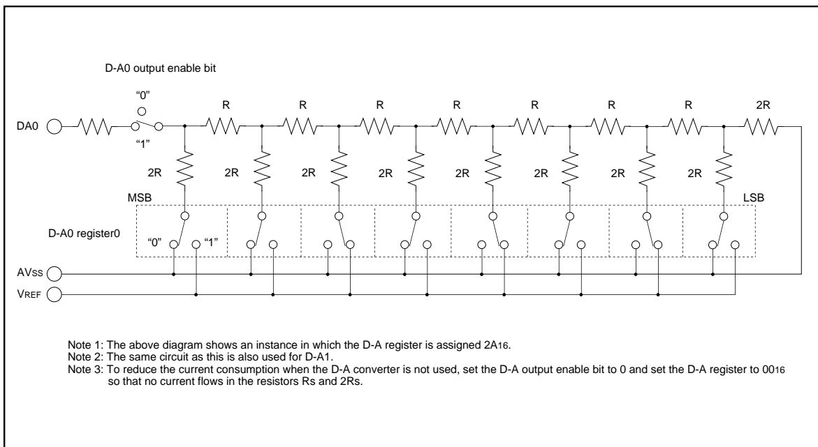
Figure 1.21.3. D-A converter equivalent circuit
