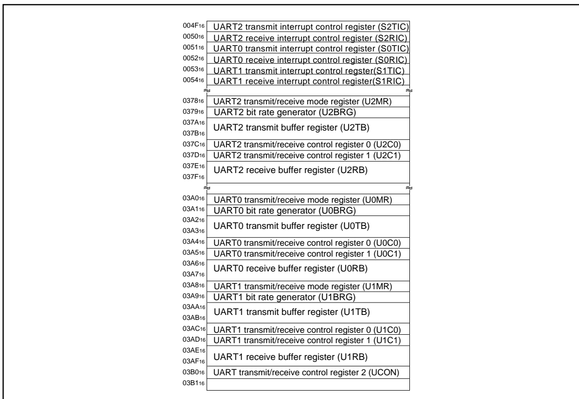
Figure 2.4.1. Memory map of serial I/O-related registers
