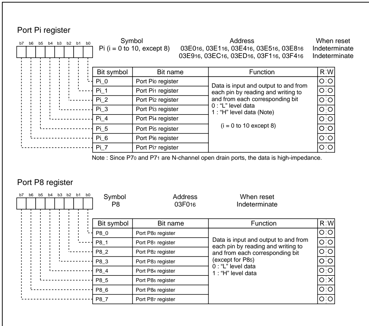
Figure 1.23.7. Port register
