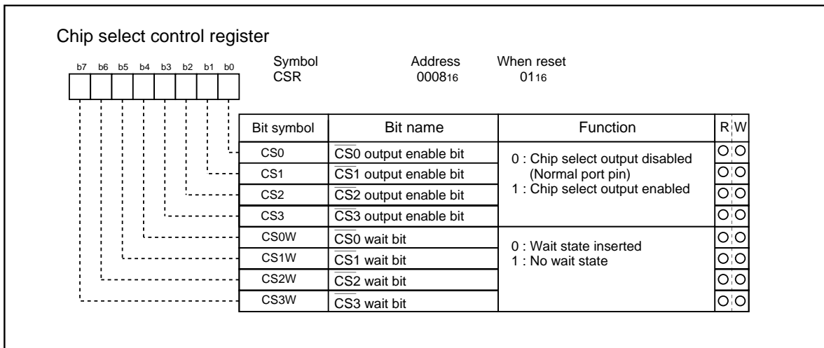
Figure 1.12.1. Chip select control register
