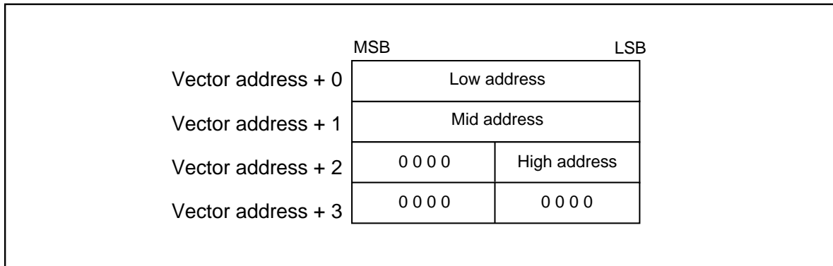
Figure 1.14.2. Format for specifying interrupt vector addresses
