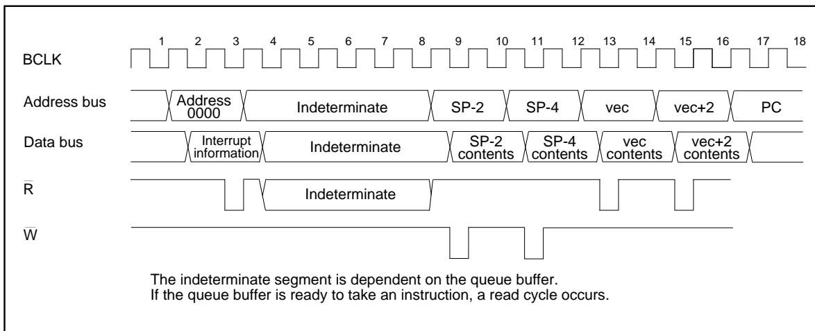
Figure 1.14.5. Time required for executing the interrupt sequence
