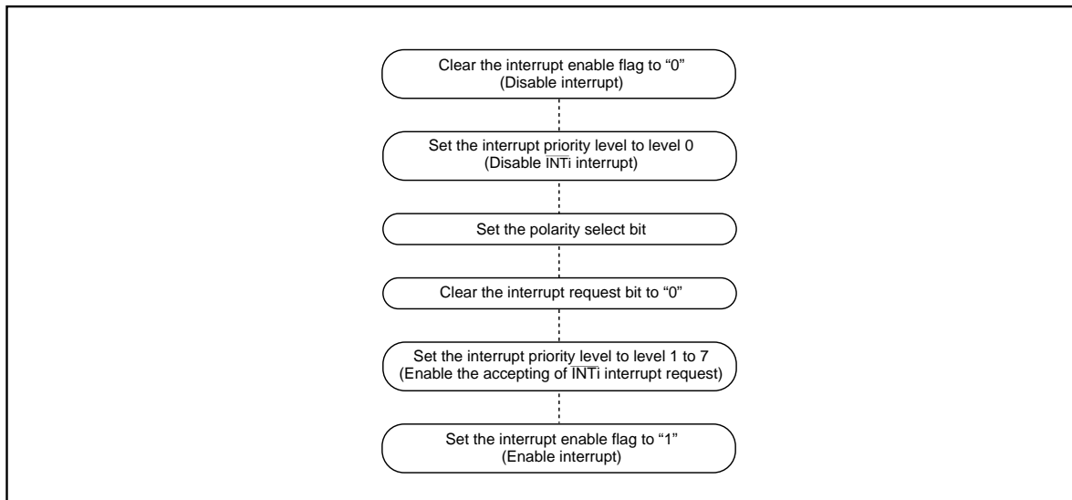
Figure 1.14.13. Switching condition of INT interrupt request
