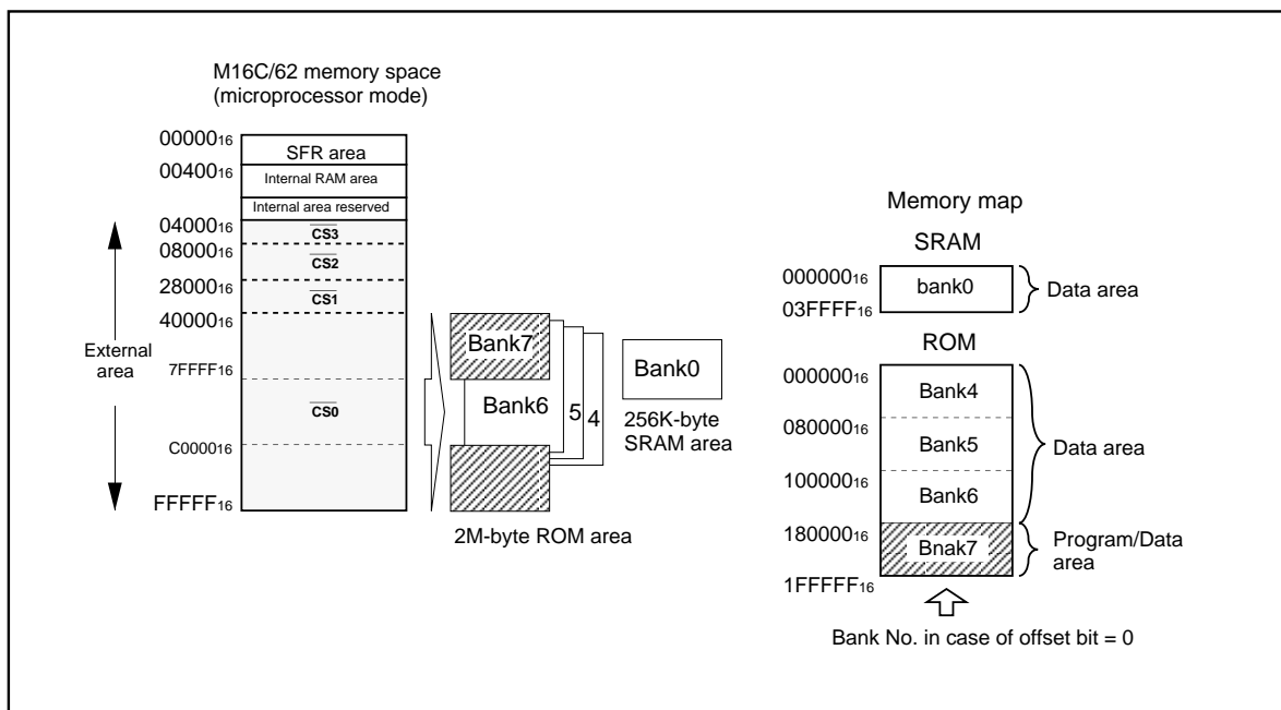
Figure 5.3.9. Memory map
