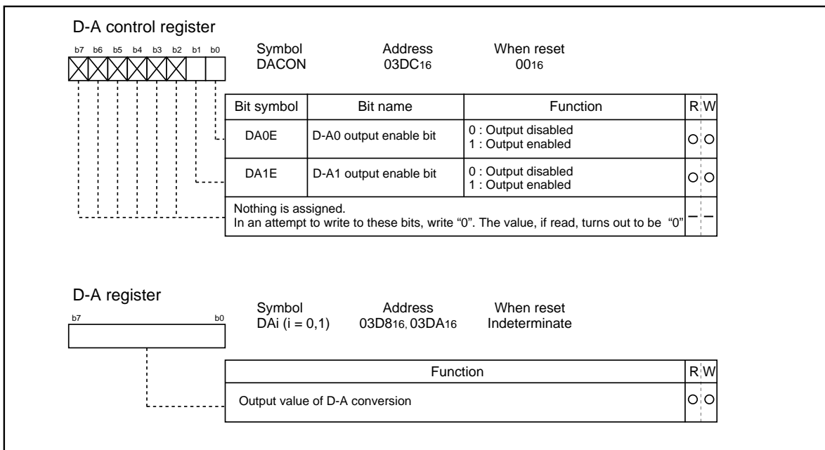
Figure 1.21.2. D-A control register
