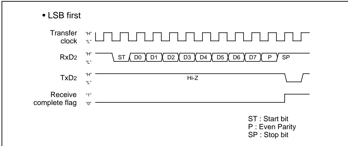
Figure 1.19.23. Output timing of the parity error signal
