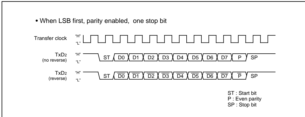
Figure 1.19.20. Timing for switching serial data logic
