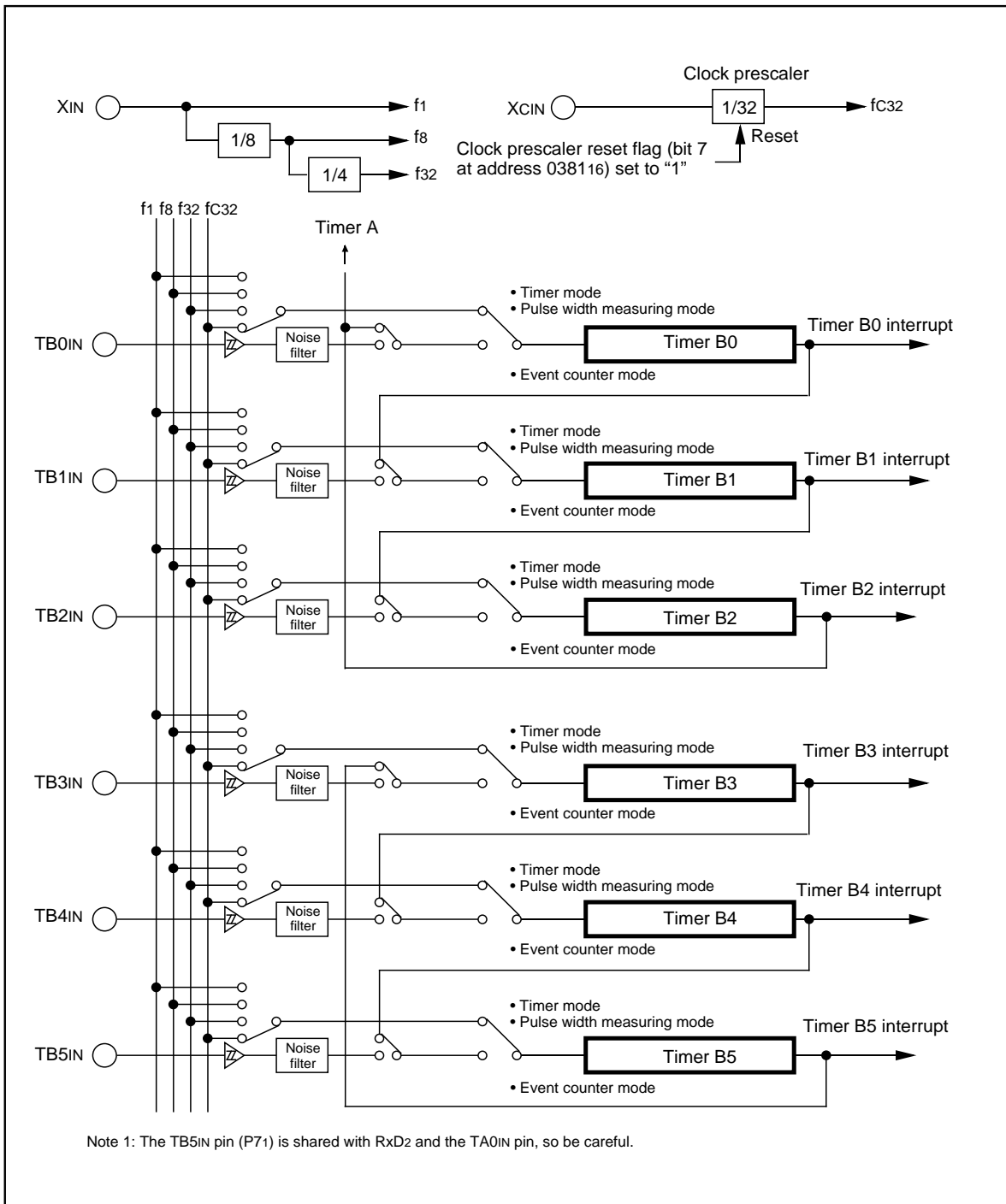
Figure 1.17.2. Timer B block diagram
