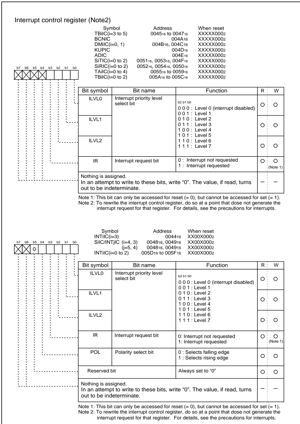
Figure 4.2.2. Interrupt control registers
