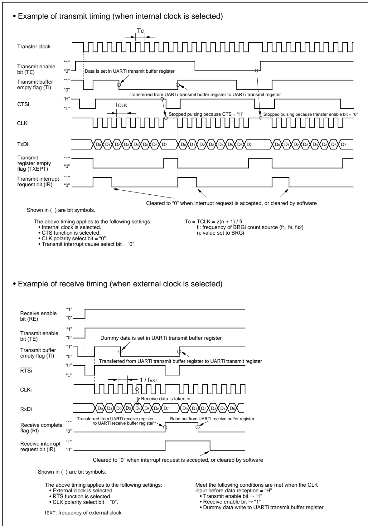
Figure 1.19.10. Typical transmit/receive timings in clock synchronous serial I/O mode
