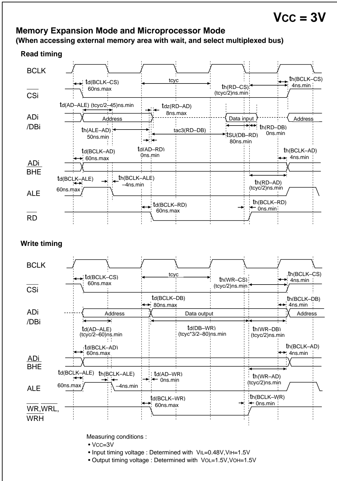
Figure 1.26.11. V_{CC}=3V timing diagram (5)
