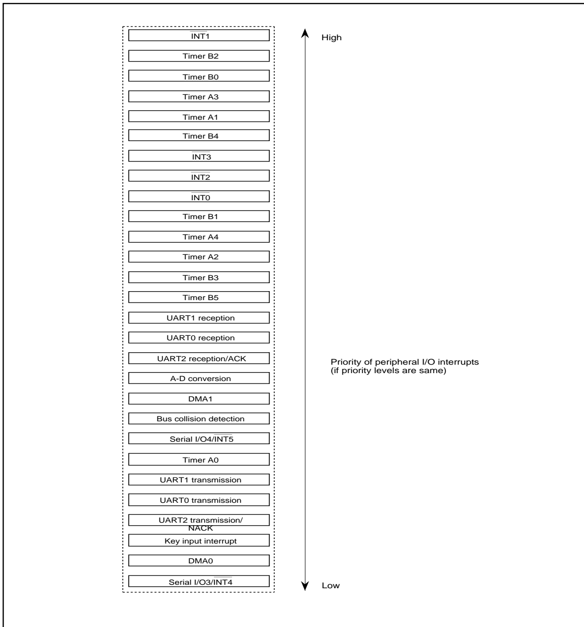
Figure 4.5.1. Maskable interrupts priorities (peripheral I/O interrupts)
