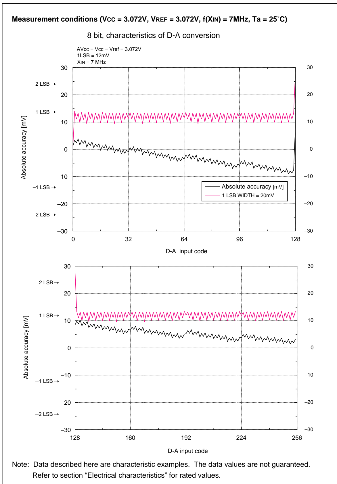
Figure 7.3.2. Characteristics of the D-A converter
