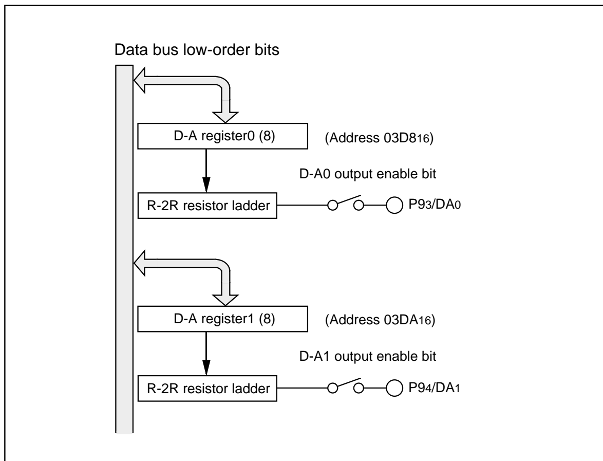
Figure 1.21.1. Block diagram of D-A converter
