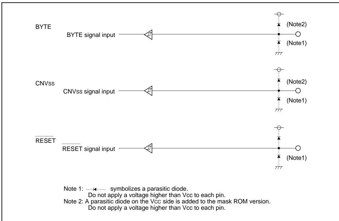
Figure 1.23.5. I/O pins
