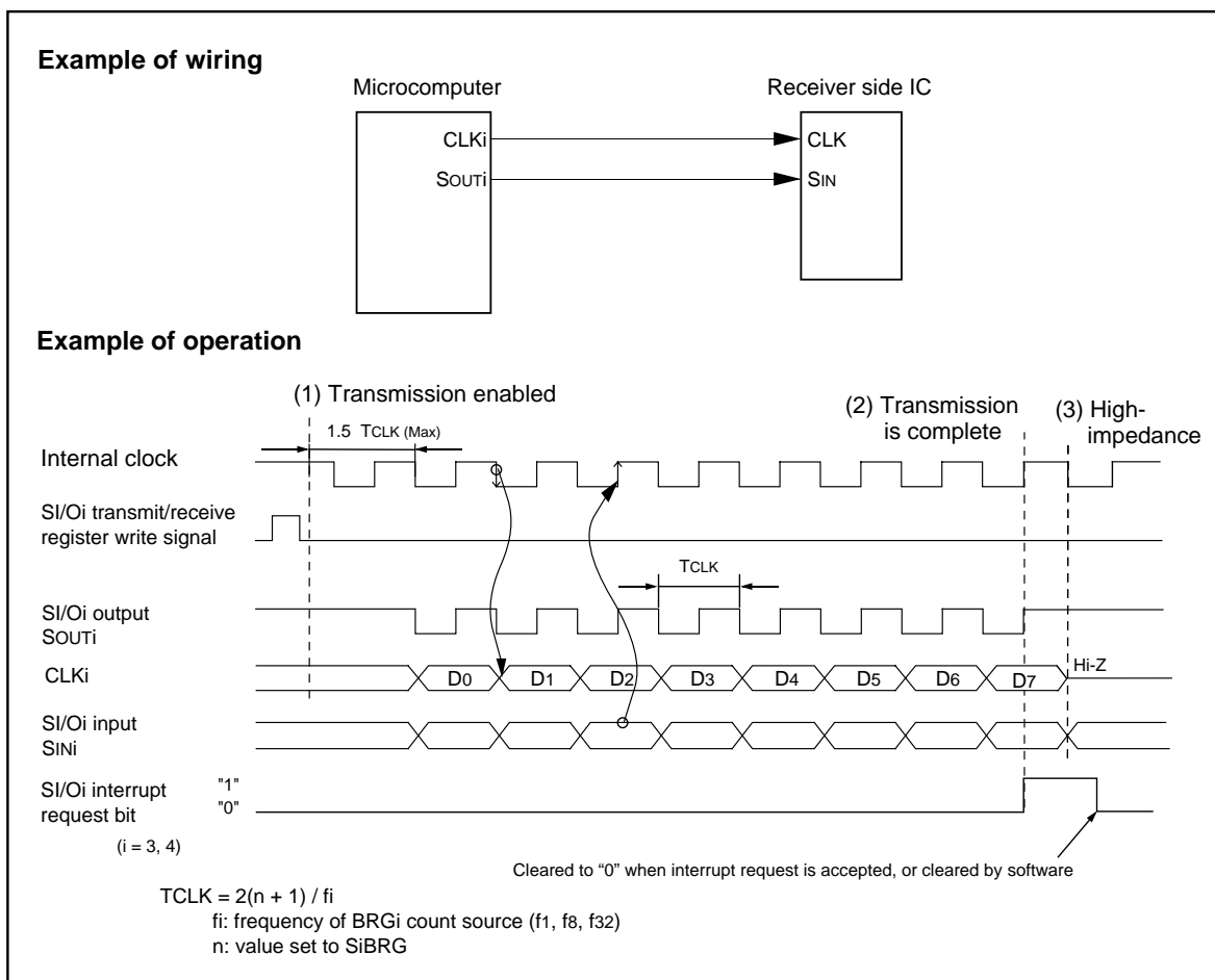
Figure 2.6.3. Operation timing of transmission in SI/O3, 4 mode
