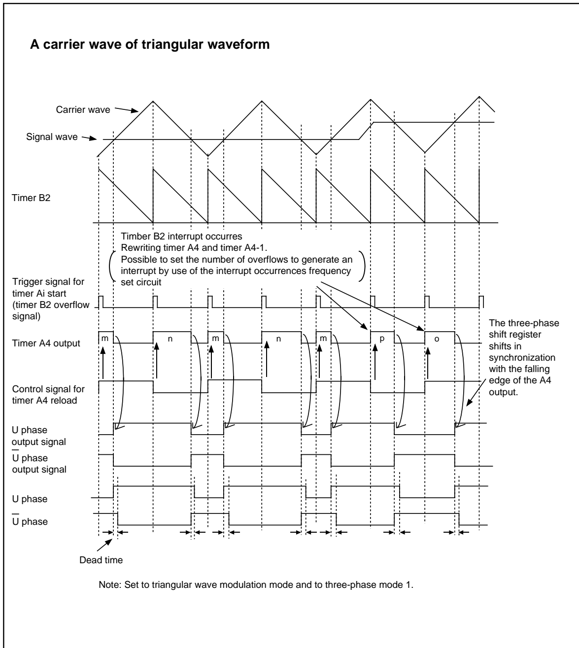
Figure 1.18.6. Timing chart of operation (1)
