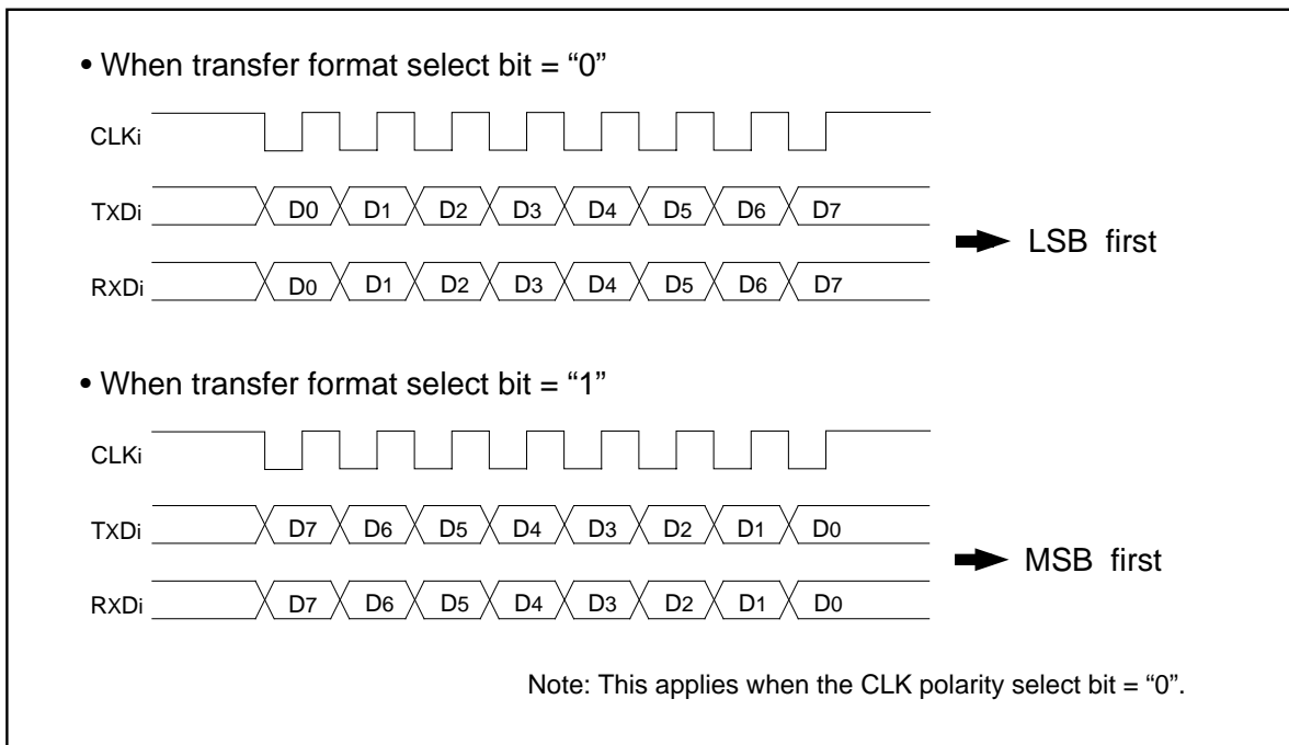
Figure 1.19.12. Transfer format
