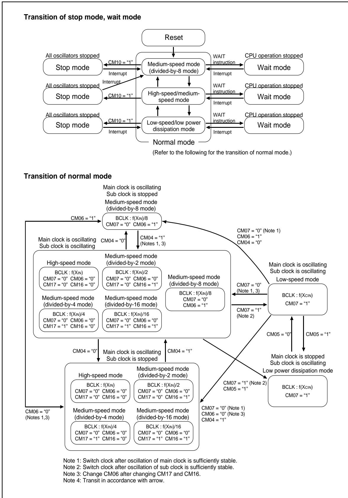
Figure 1.13.5. State transition diagram of Power control mode
