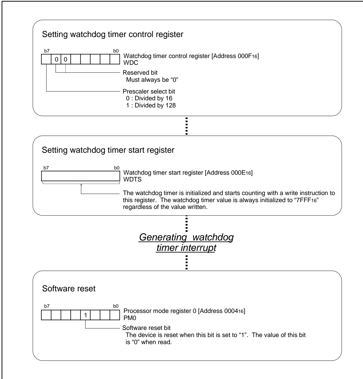
Figure 2.11.4. Set-up procedure of watchdog timer
