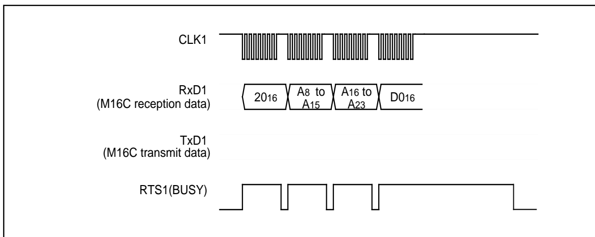
Figure 1.31.7. Timing for block erasing
