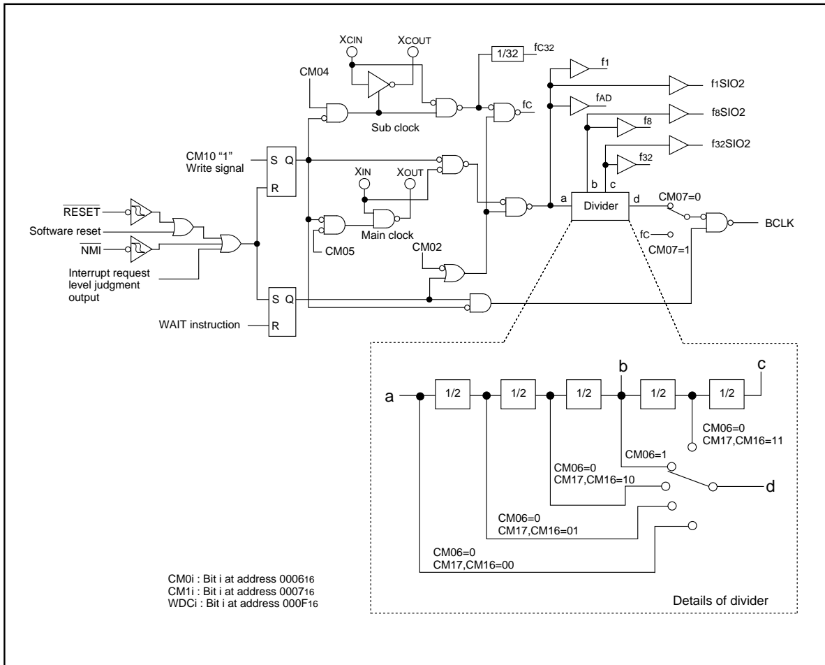
Figure 1.13.3. Clock generating circuit
