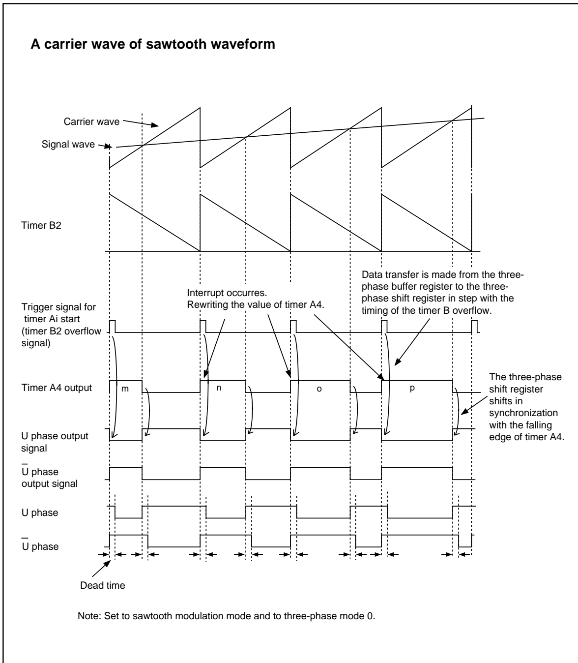
Figure 1.18.8. Timing chart of operation (3)
