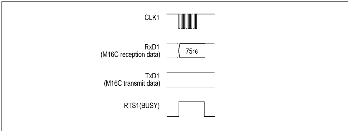
Figure 1.31.12. Timing for disabling the lock bit
