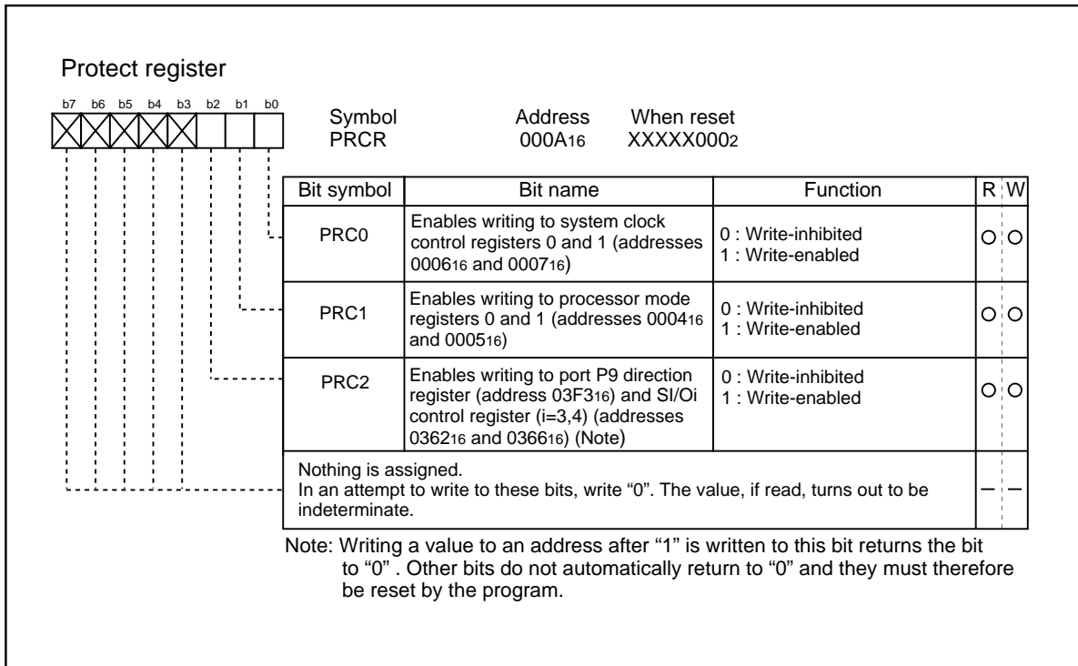
Figure 2.1.1. Protect register
