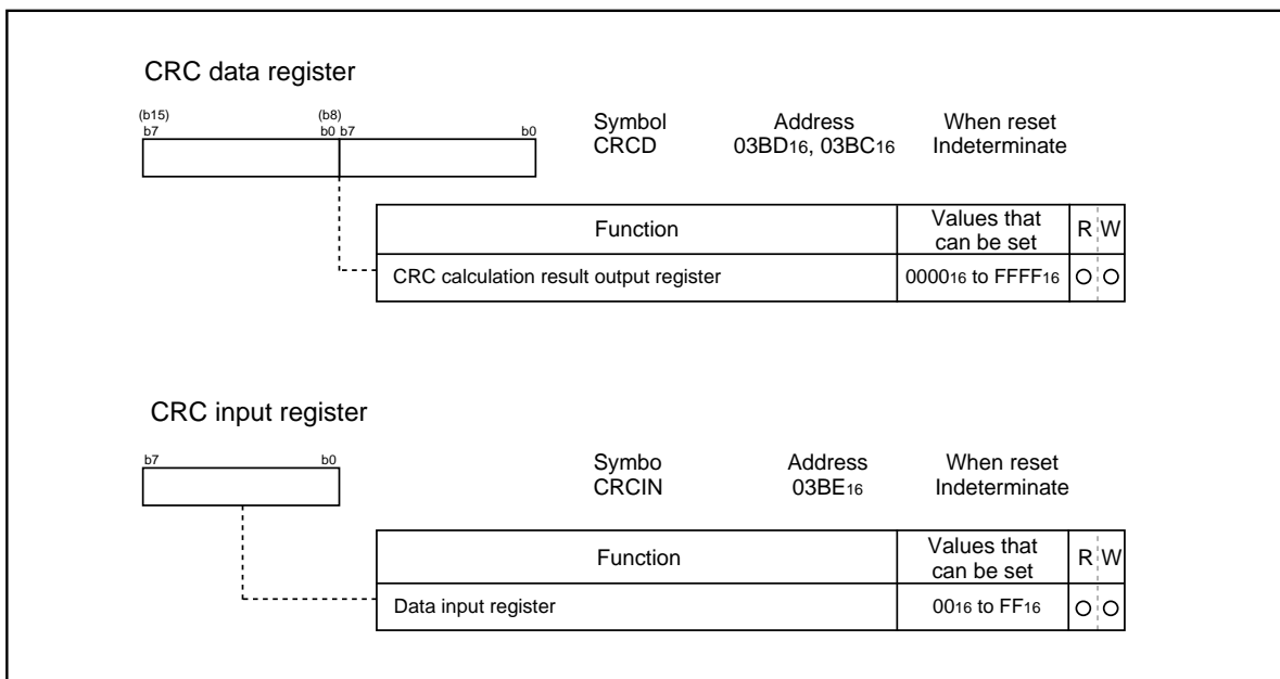
Figure 1.22.2. CRC-related registers
