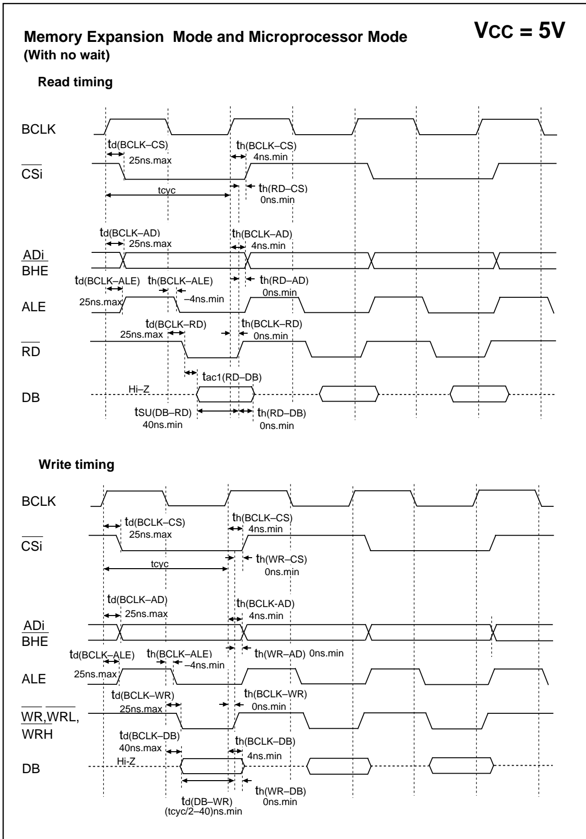
Figure 1.26.4. Vcc=5V timing diagram (3)
