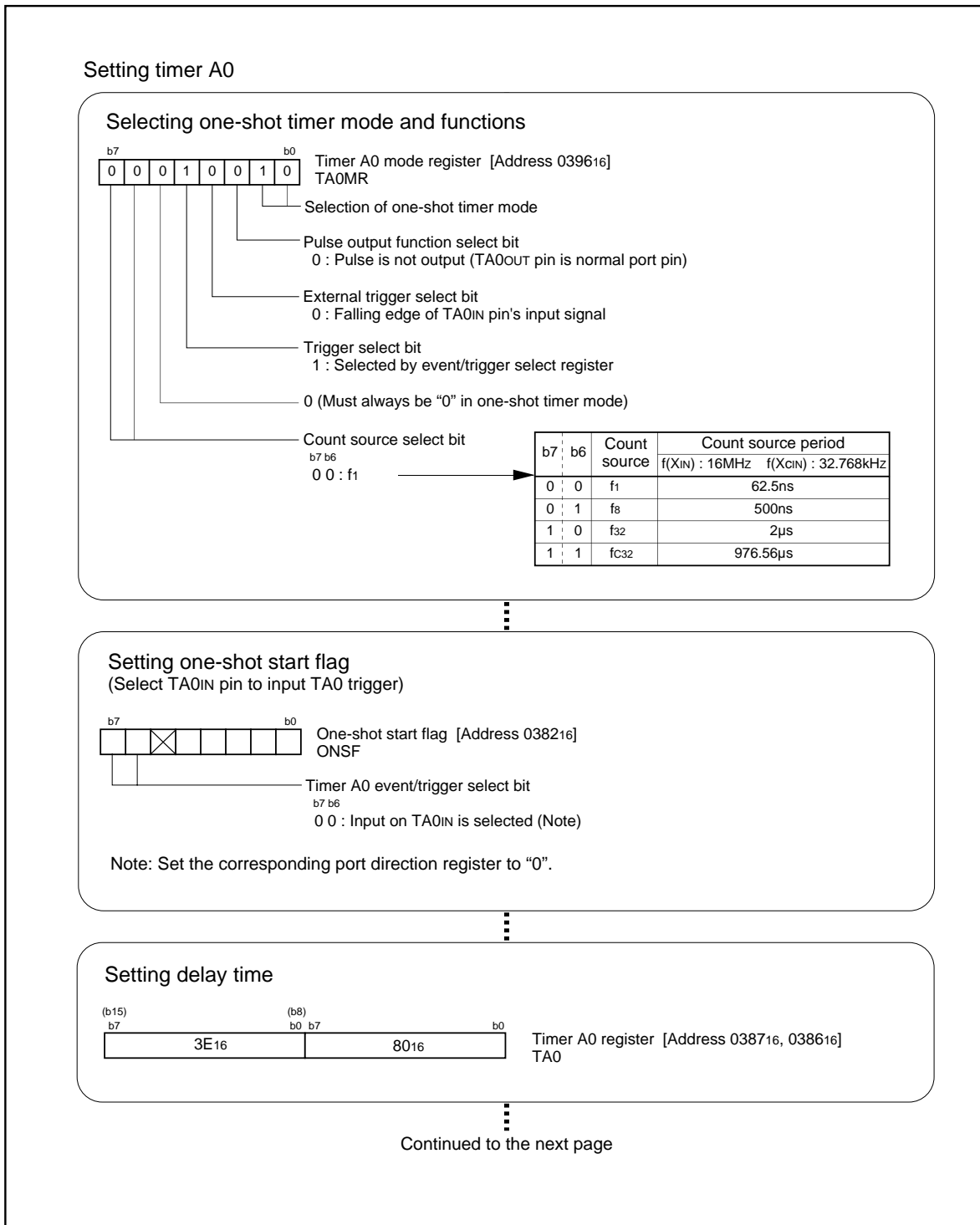
Figure 3.3.3. Set-up procedure of delayed one-shot output (1)
