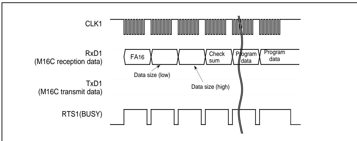
Figure 1.31.13. Timing for download
