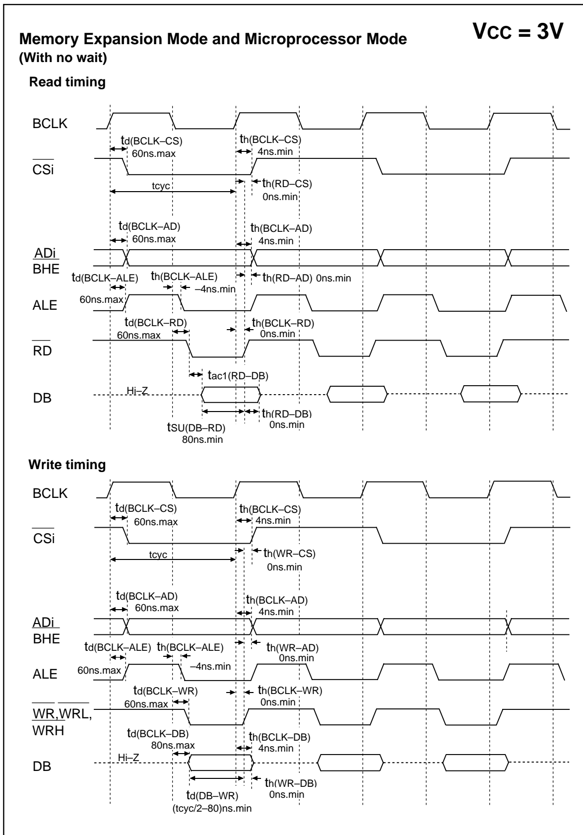
Figure 1.26.9. V_{CC}=3V timing diagram (3)
