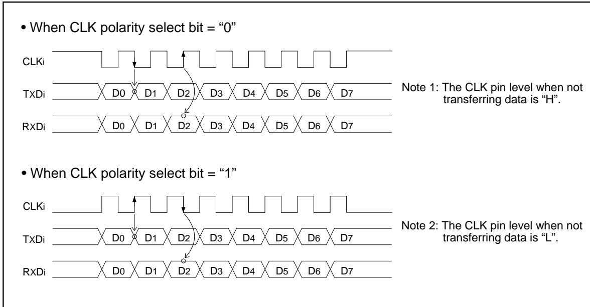
Figure 1.19.11. Polarity of transfer clock
