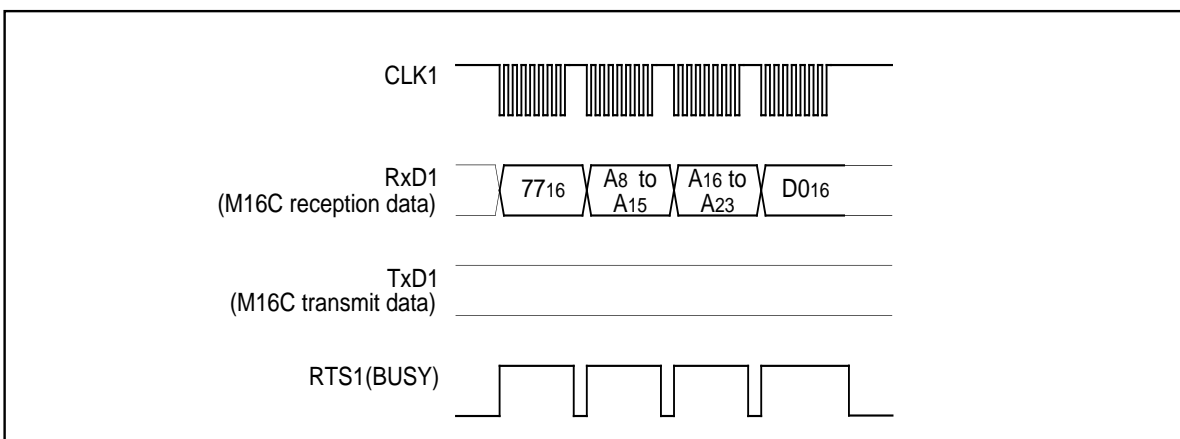
Figure 1.31.9. Timing for the lock bit program
