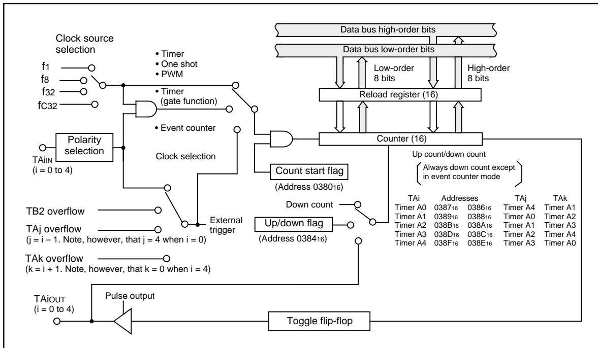
Figure 1.17.3. Block diagram of timer A
