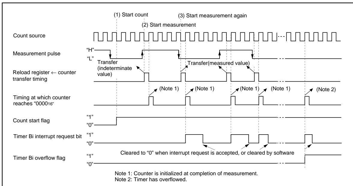
Figure 2.3.10. Operation timing of pulse width measurement mode
