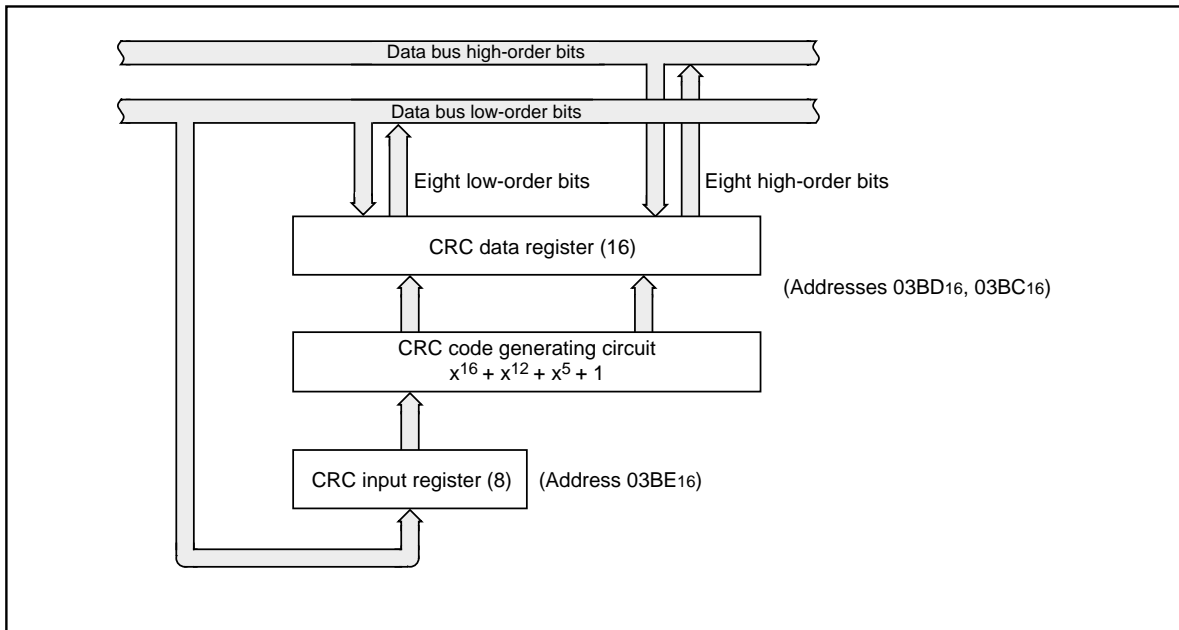
Figure 1.22.1. Block diagram of CRC circuit
