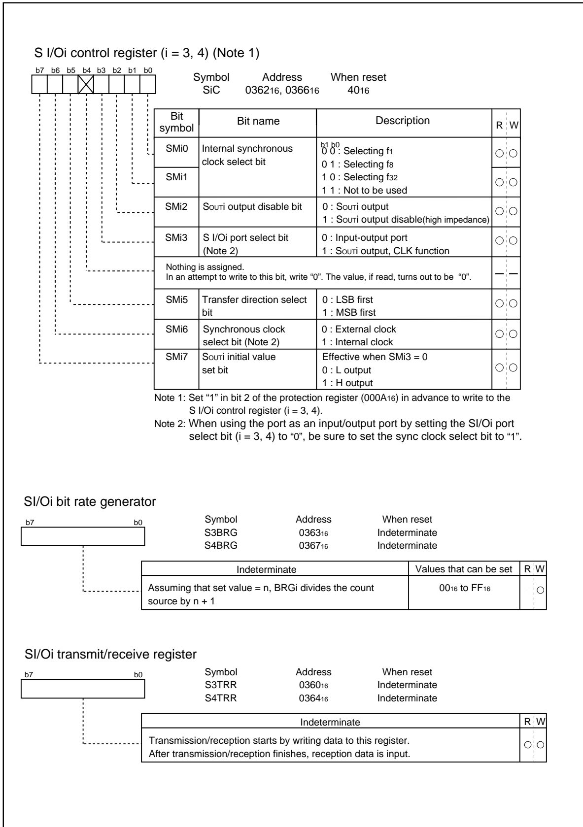
Figure 1.19.32. S I/O3, 4 related register
