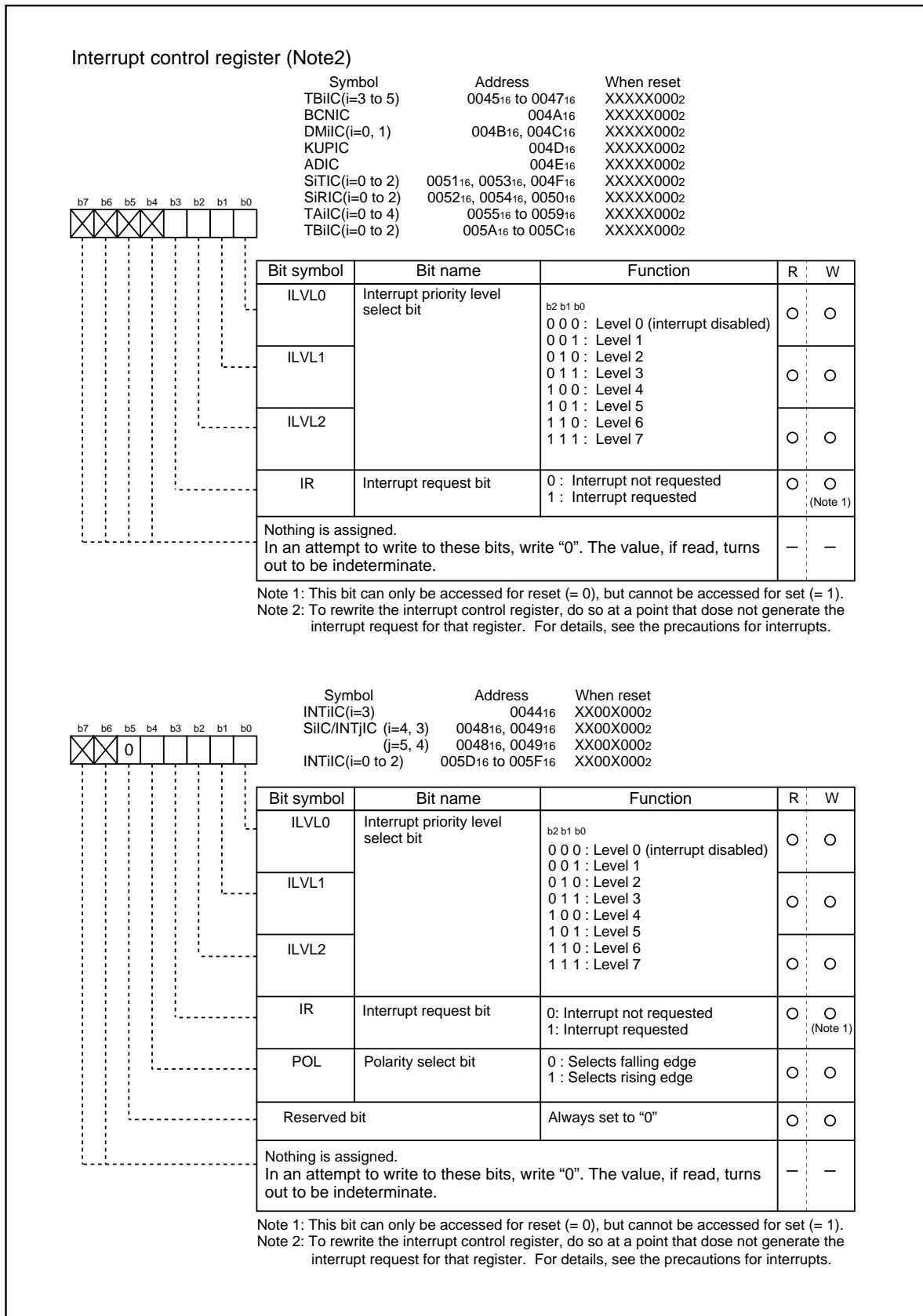
Figure 1.14.3. Interrupt control registers
