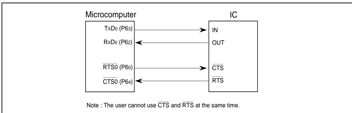
Figure 1.19.19. The separate CTS/RTS pins function usage
