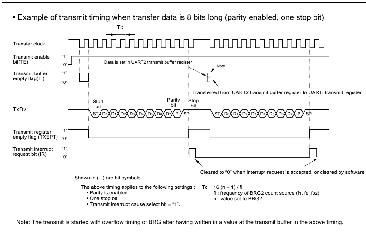
Figure 1.19.17. Typical transmit timings in UART mode(UART2)
