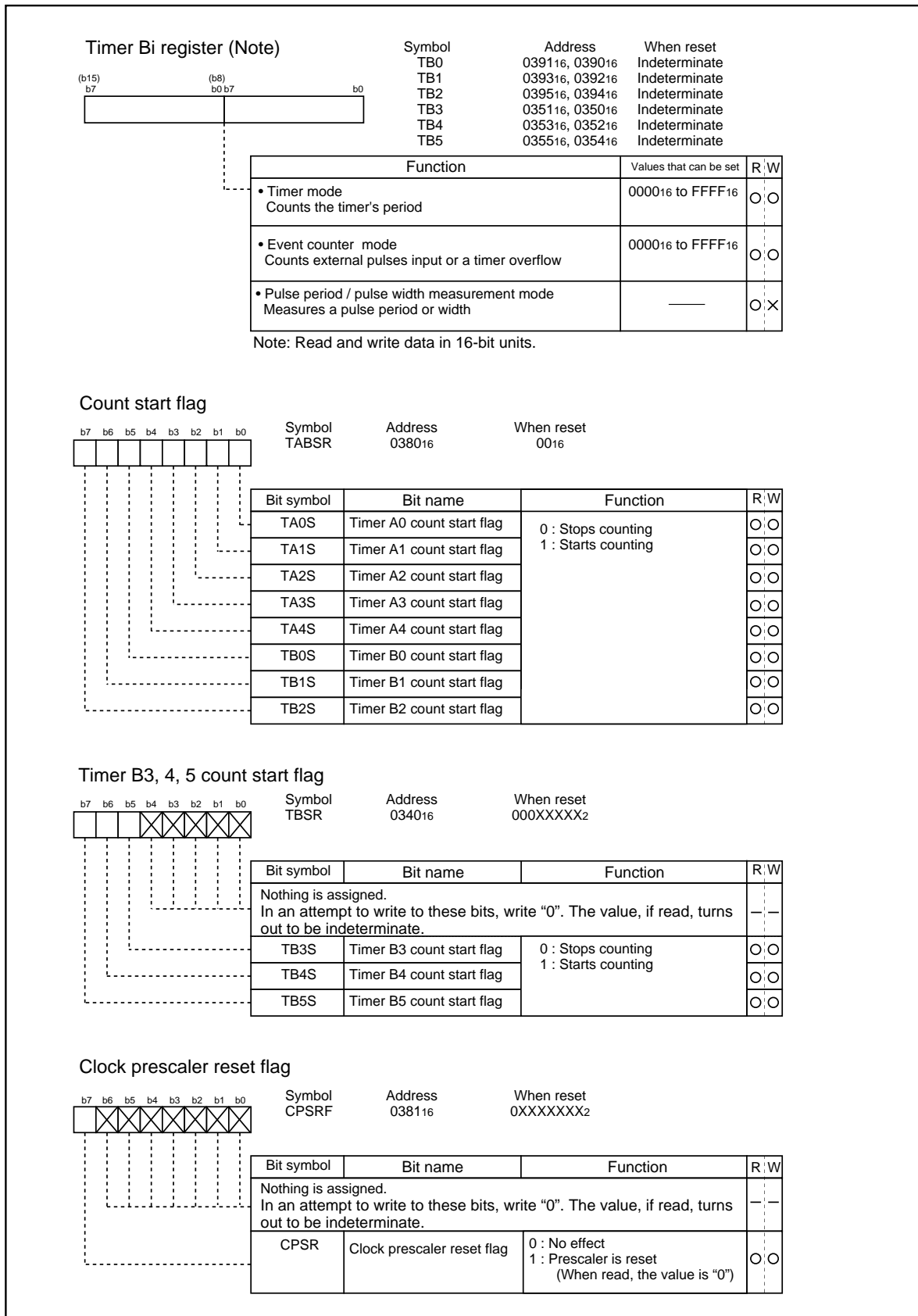
Figure 1.17.16. Timer B-related registers (2)
