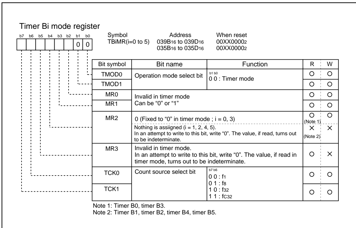
Figure 1.17.17. Timer Bi mode register in timer mode
