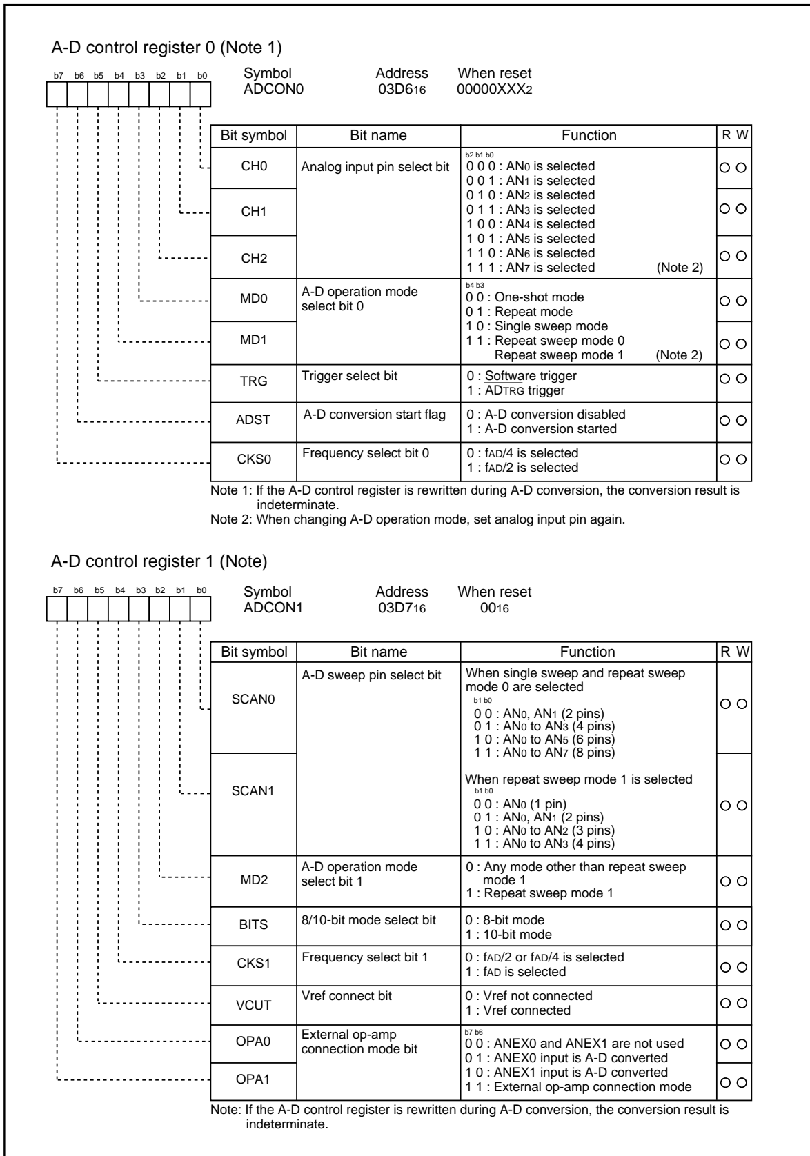
Figure 1.20.2. A-D converter-related registers (1)
