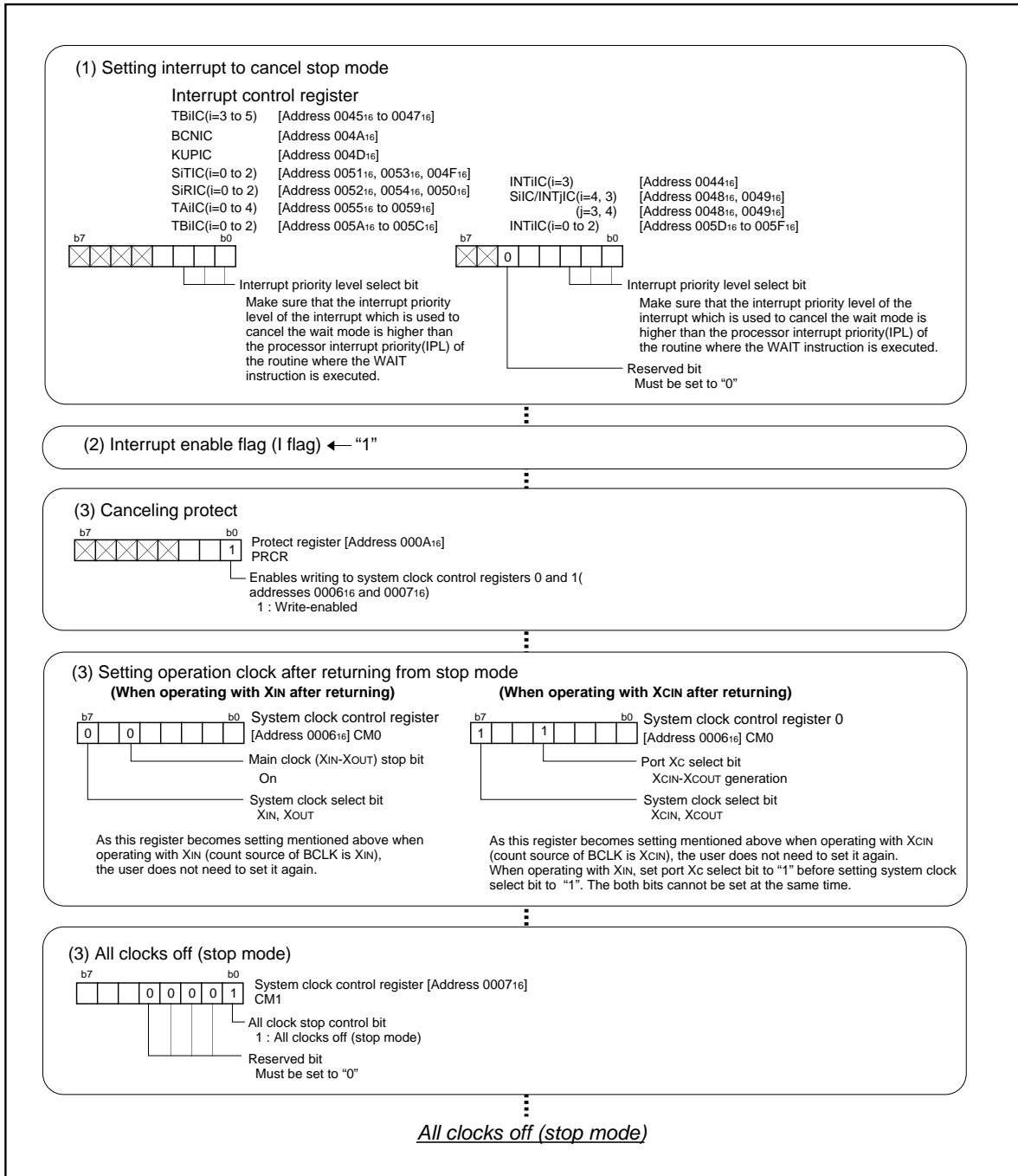
Figure 2.14.5. Example of stop mode set-up
