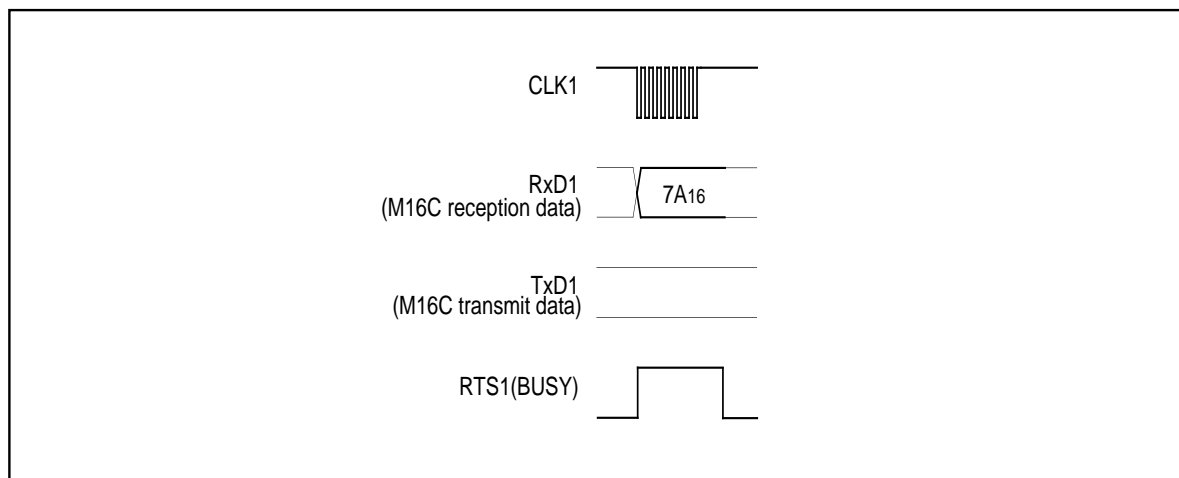
Figure 1.31.11. Timing for enabling the lock bit
