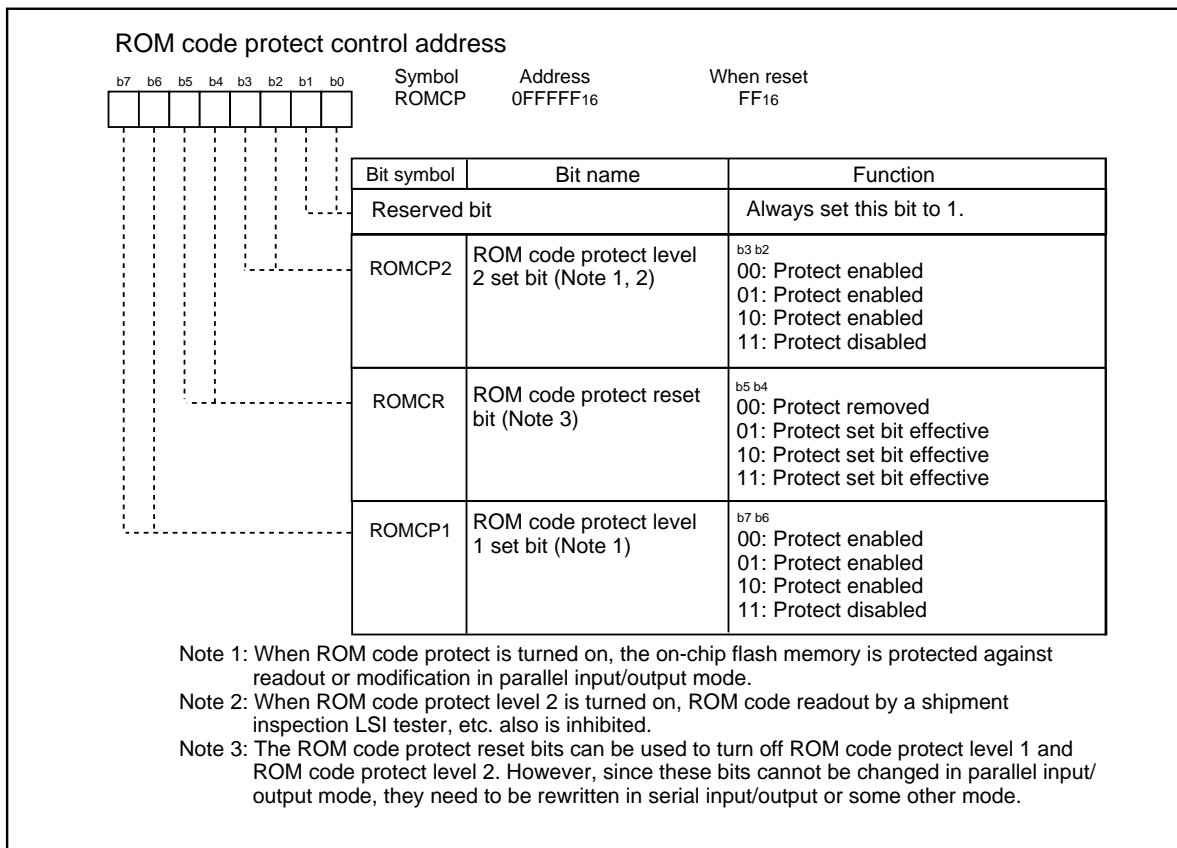
Figure 1.29.9. ROM code protect control address
