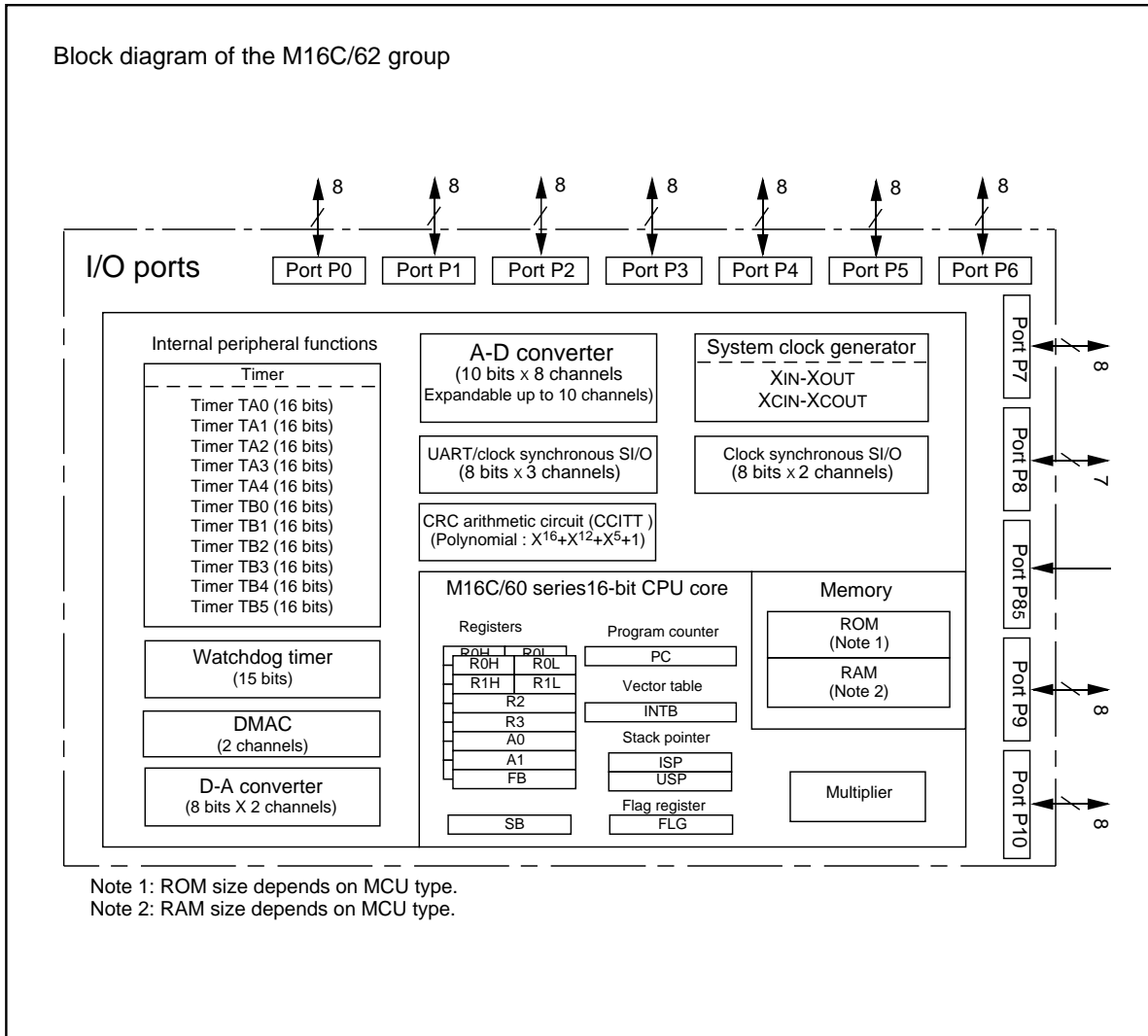
Figure 1.1.3. Block diagram of M16C/62 group
