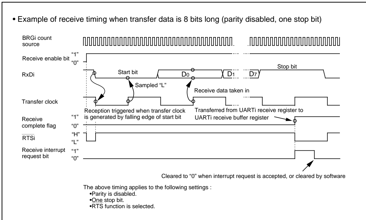
Figure 1.19.18. Typical receive timing in UART mode
