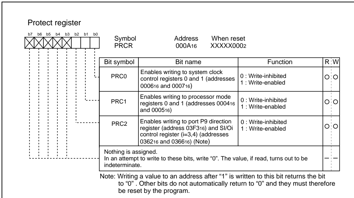
Figure 1.13.6. Protect register
