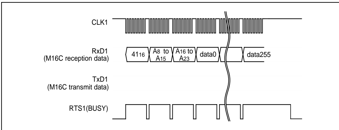
Figure 1.31.6. Timing for the page program
