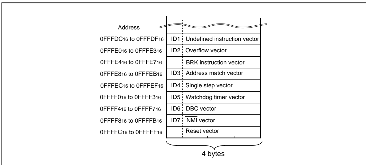
Figure 1.31.17. ID code storage addresses
