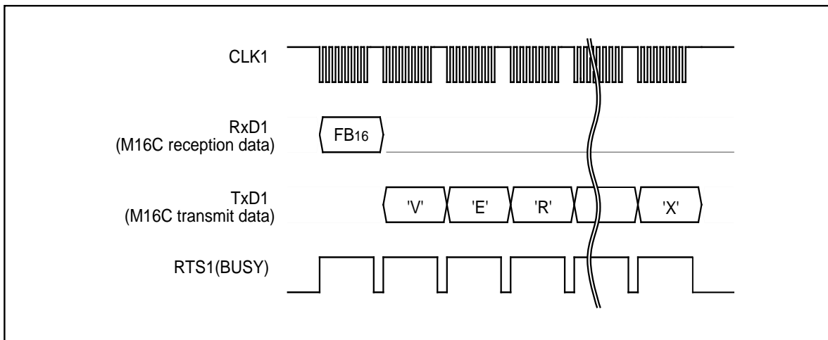
Figure 1.31.14. Timing for version information output
