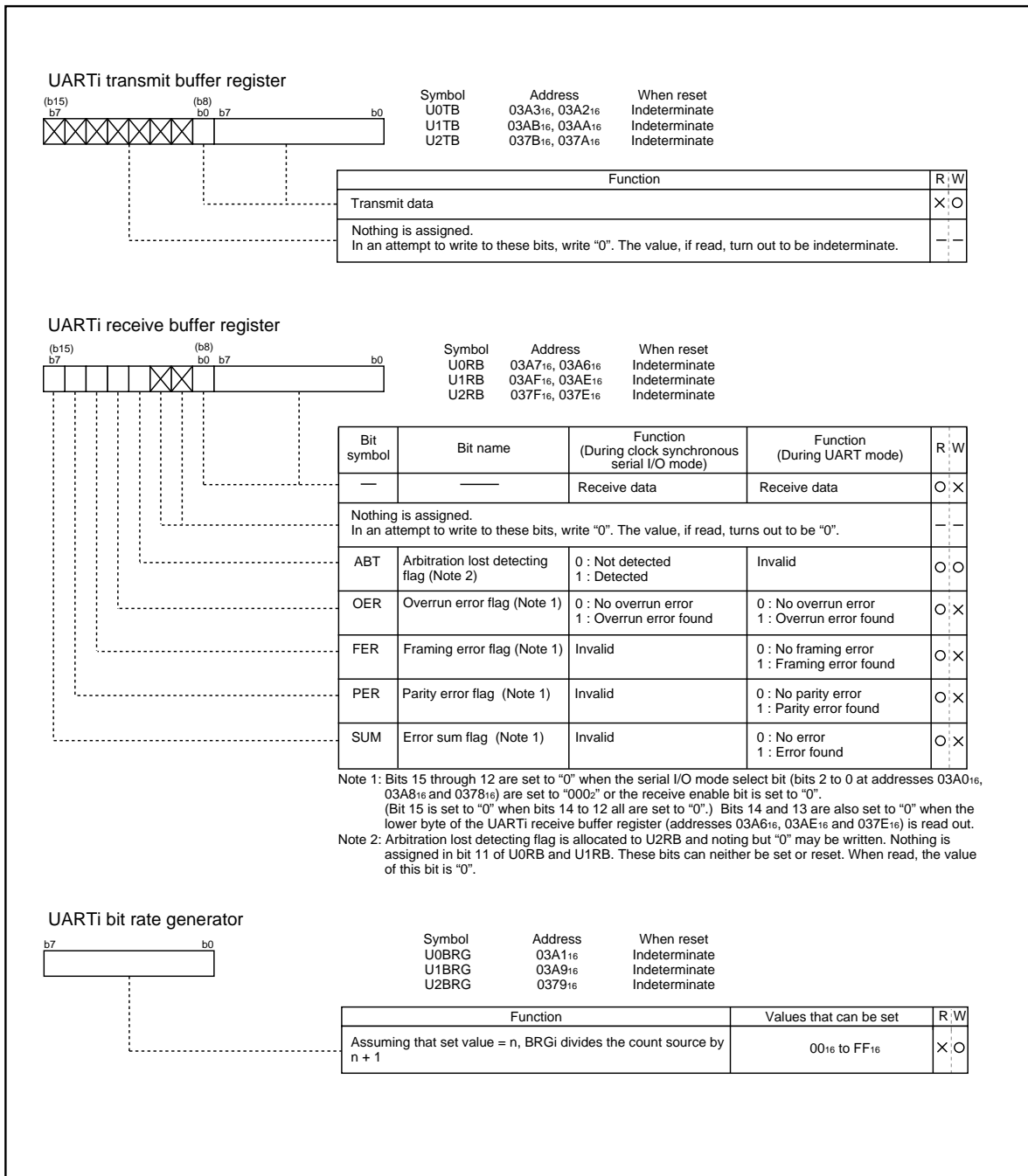
Figure 1.19.4. Serial I/O-related registers (1)
