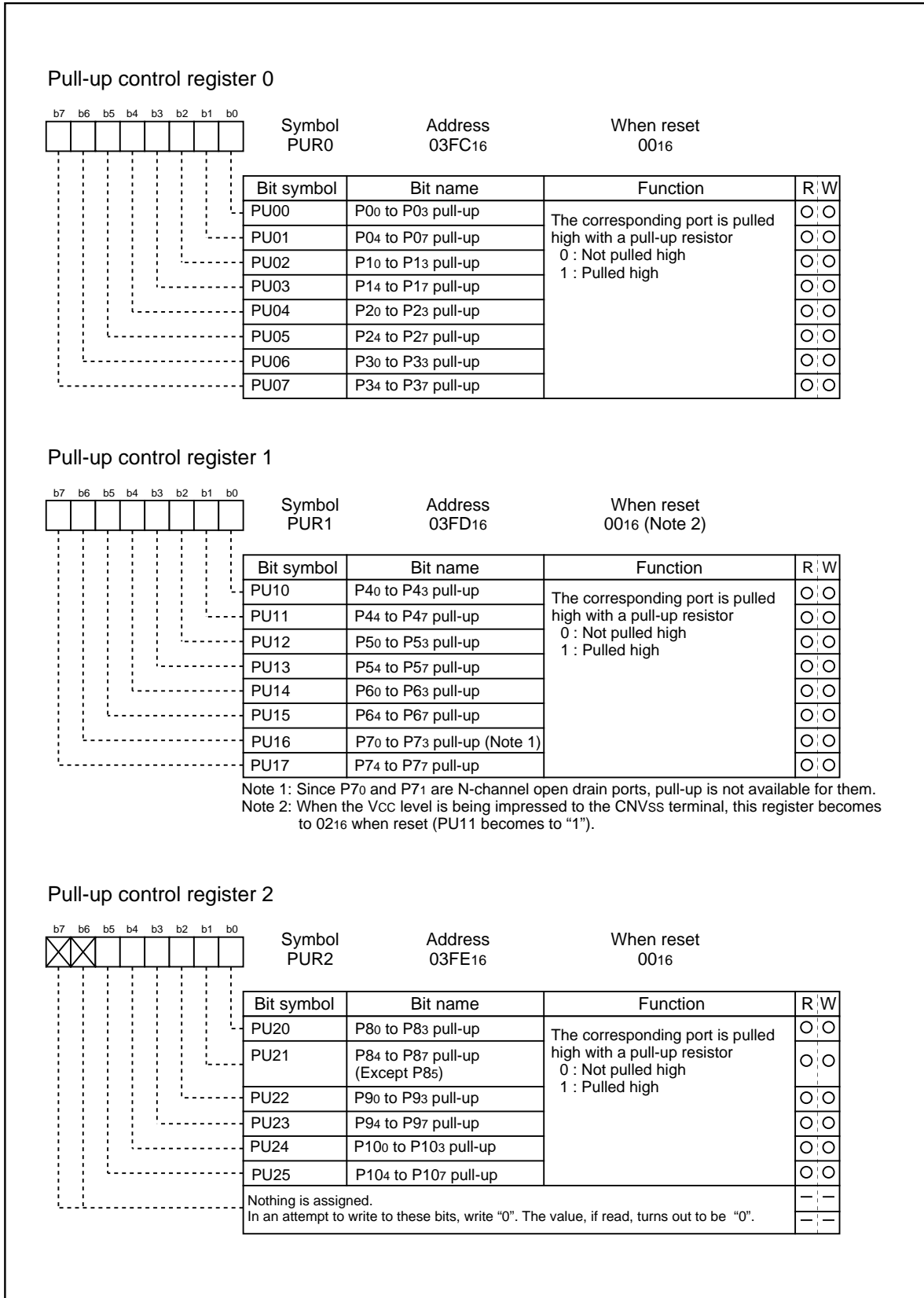
Figure 1.23.8. Pull-up control register
