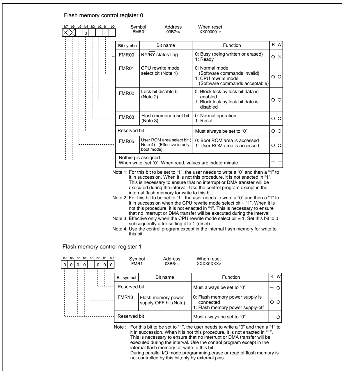
Figure 1.29.1. Flash memory control registers
