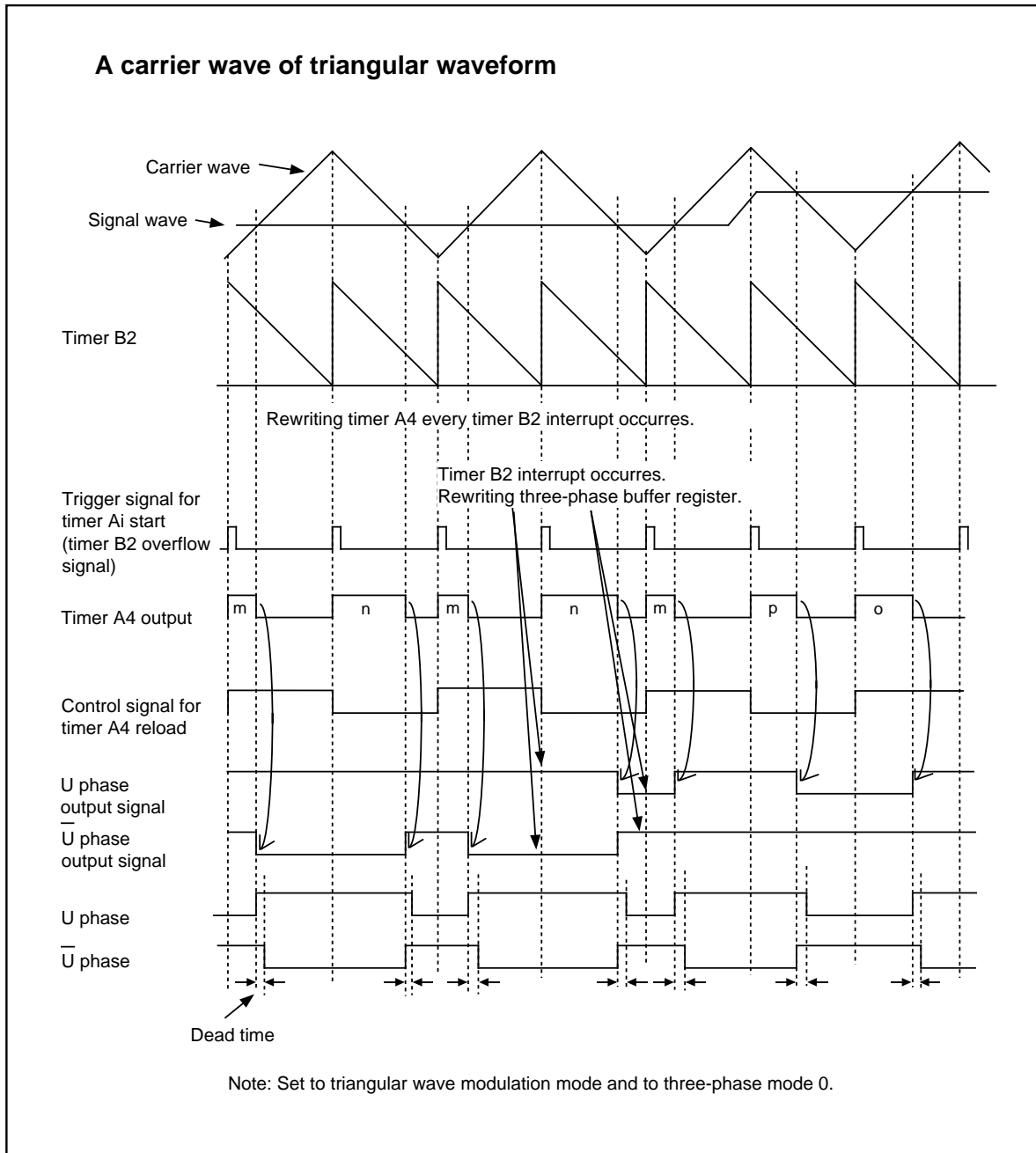
Figure 1.18.7. Timing chart of operation (2)
