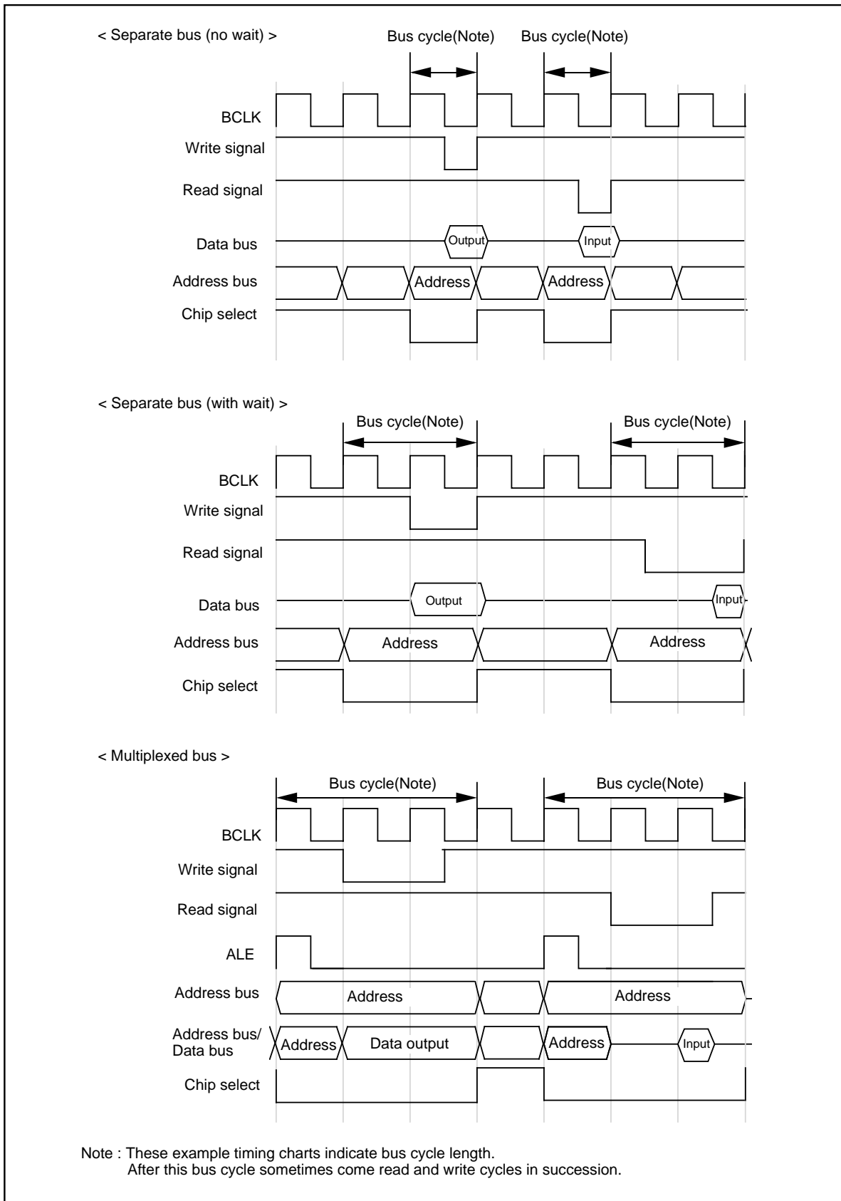
Figure 1.12.5. Typical bus timings using software wait
