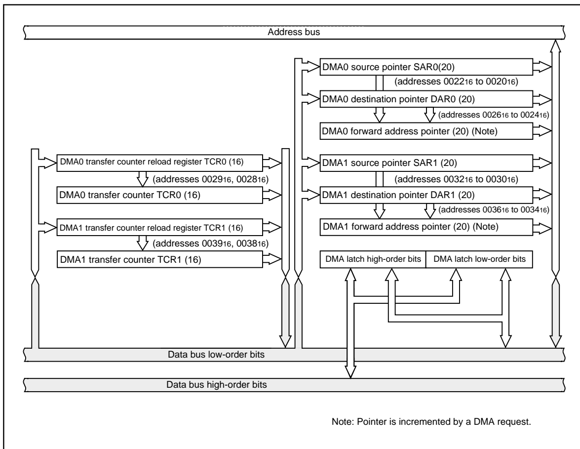
Figure 1.16.1. Block diagram of DMAC
