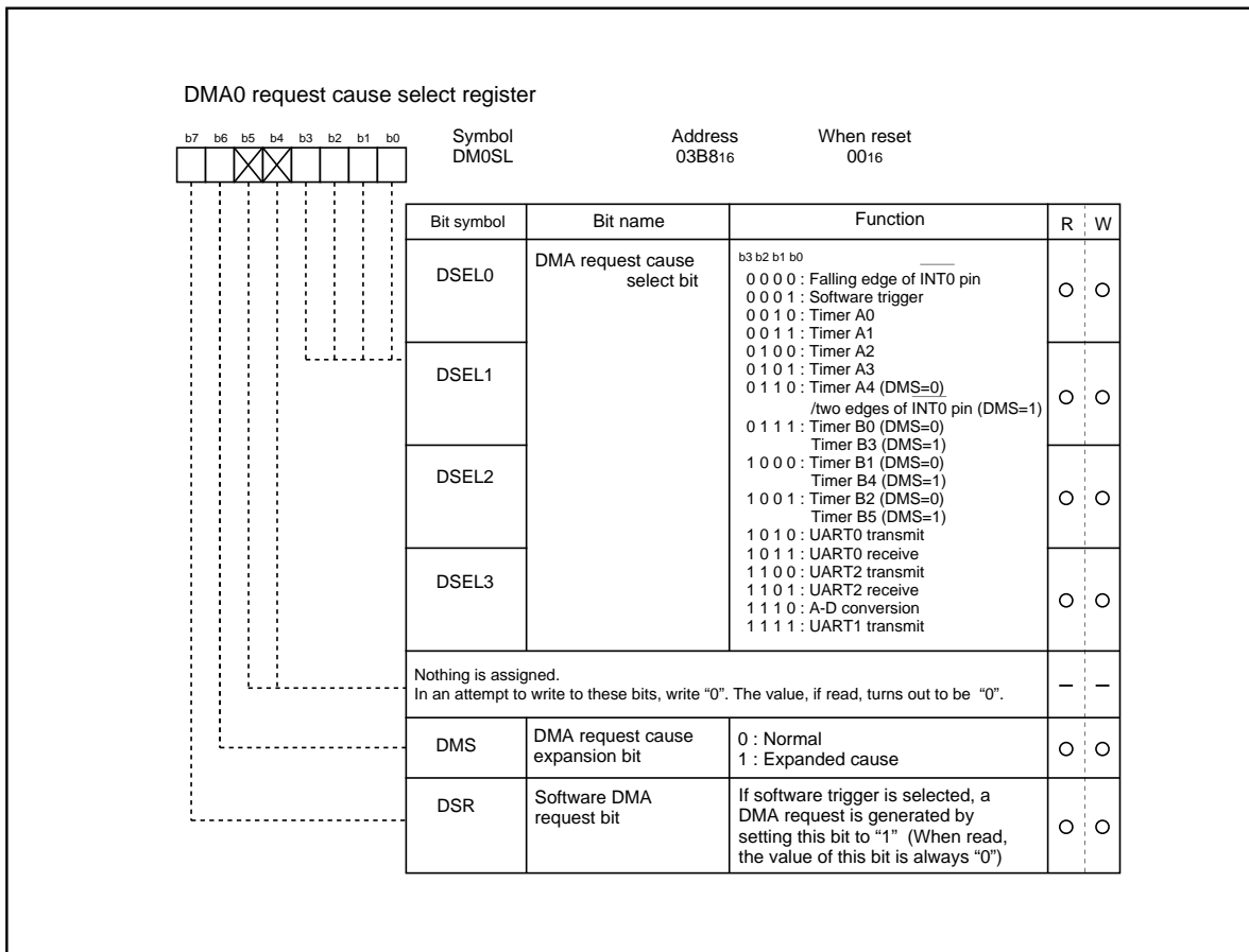
Figure 1.16.2. DMAC register (1)
