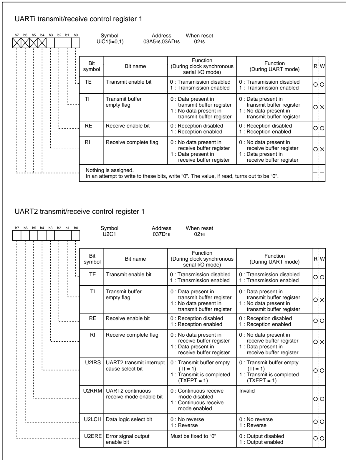
Figure 1.19.7. Serial I/O-related registers (4)
