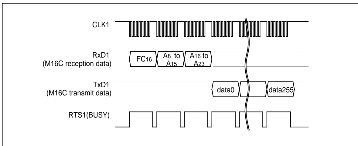
Figure 1.31.15. Timing for boot area output
