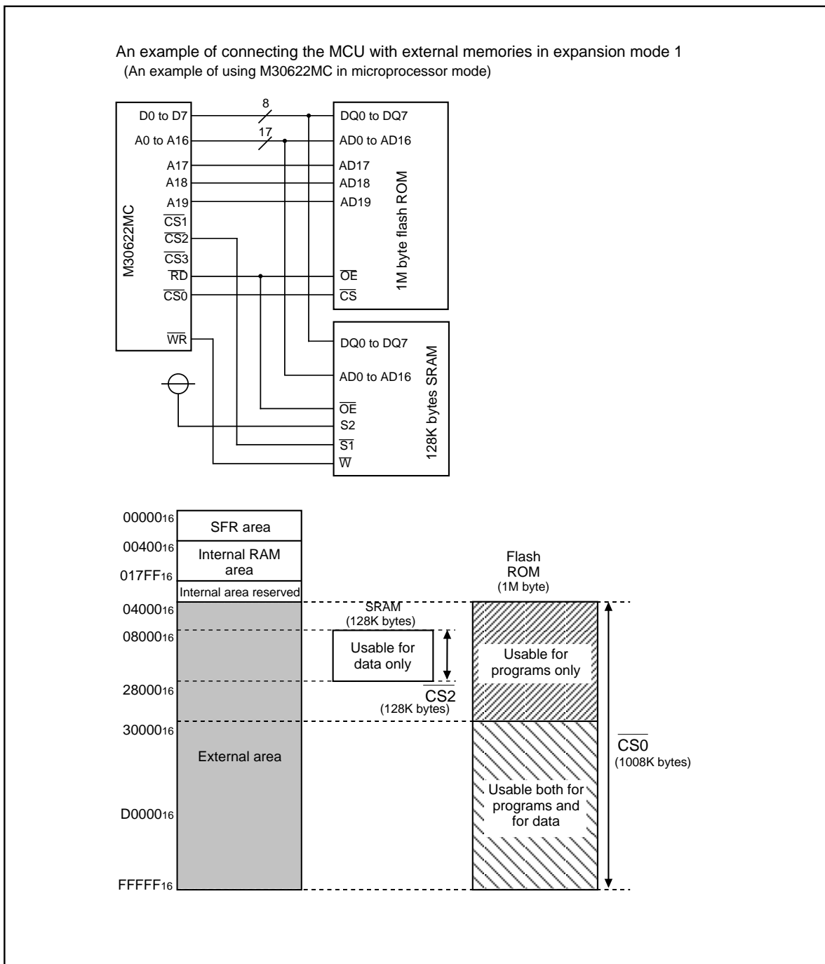
Figure 1.8.3. External memory connect example in expansion mode 1
