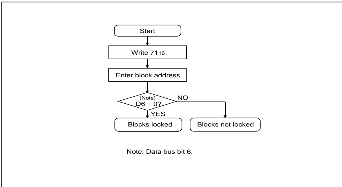
Figure 1.29.7. Read lock bit status flowchart
