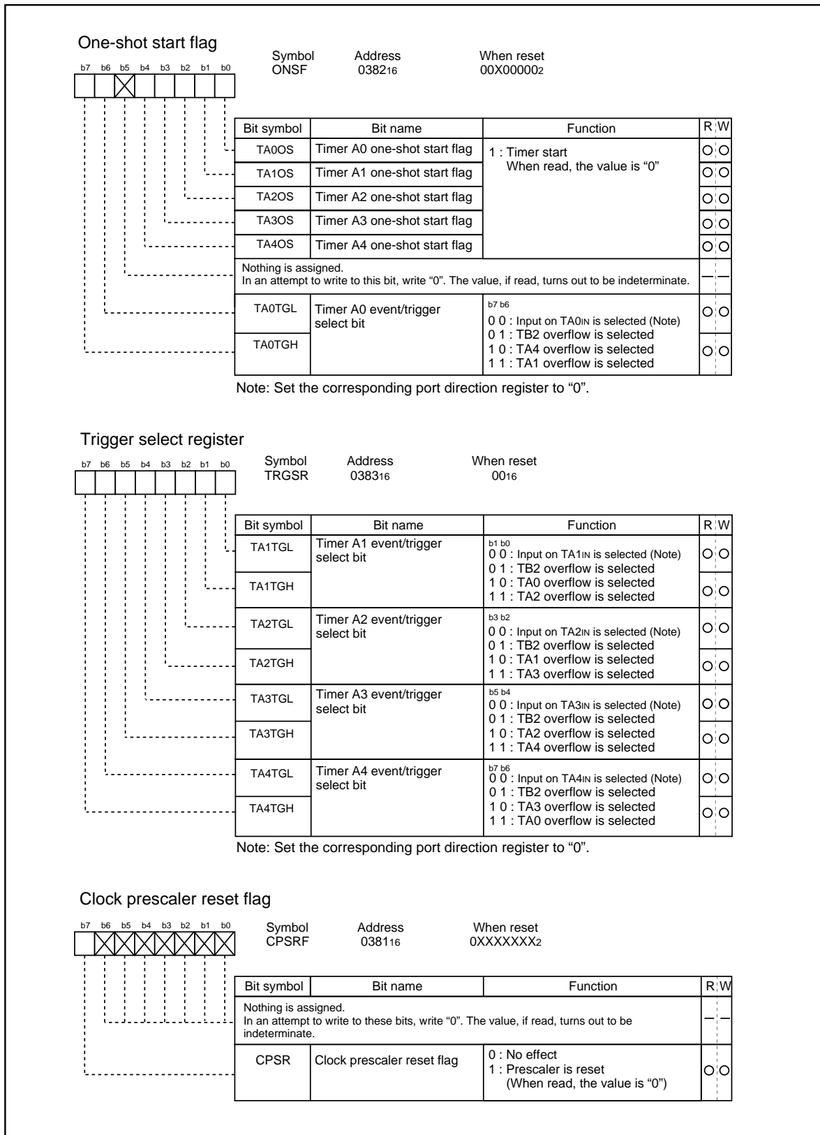
Figure 1.17.6. Timer A-related registers (3)
