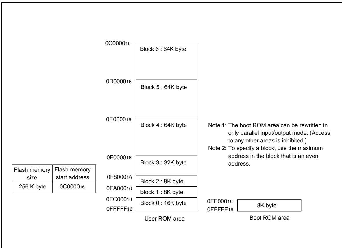
Figure 1.28.1. Block diagram of flash memory version
