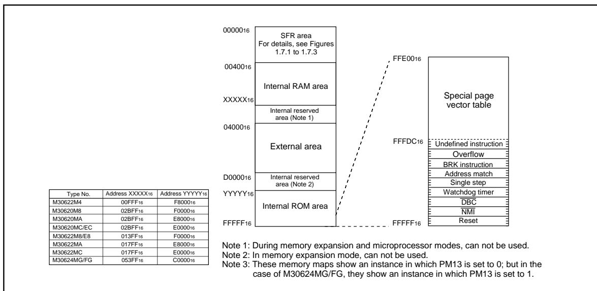
Figure 1.4.1. Memory map
