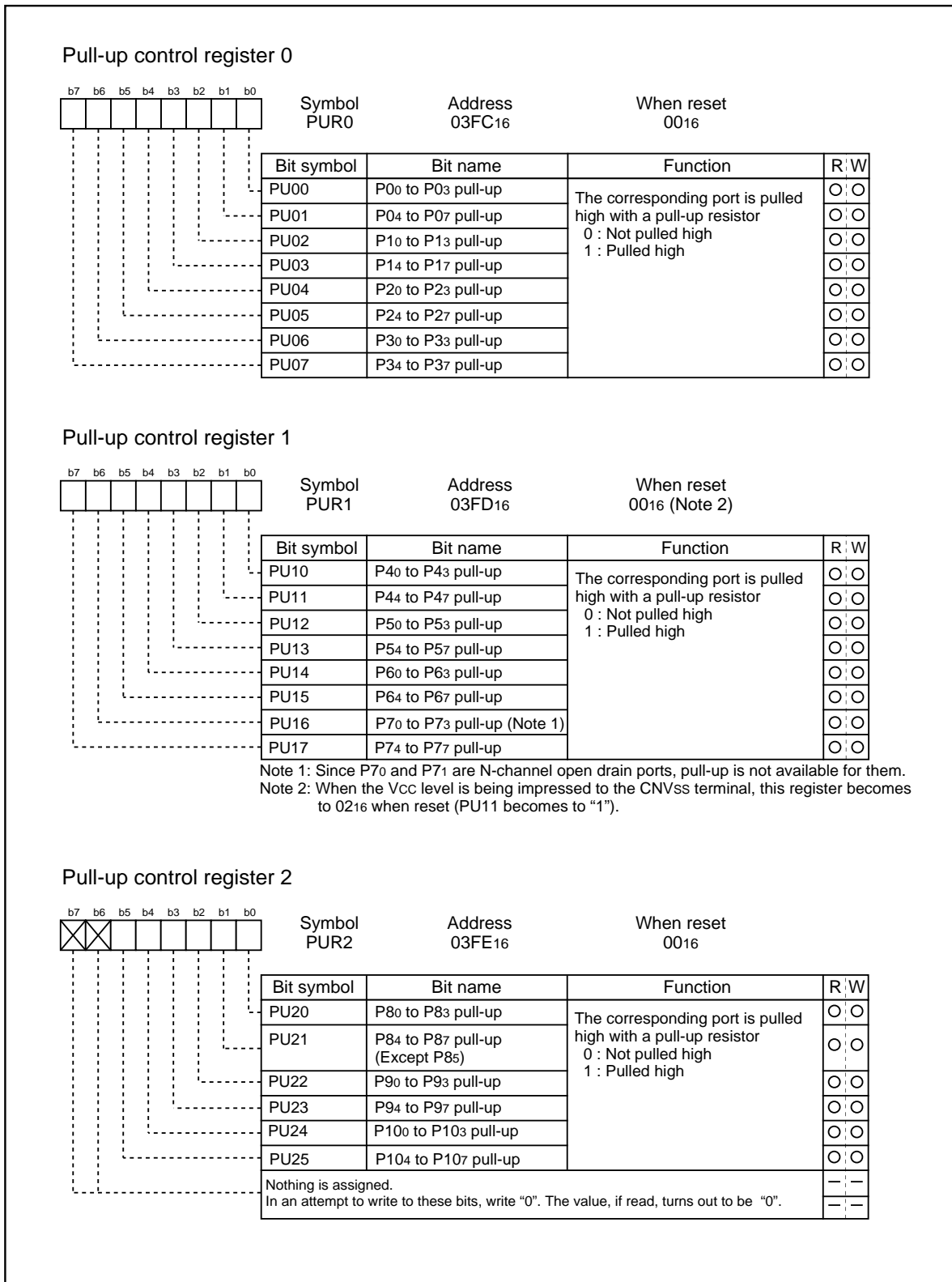
Figure 2.15.4. Programmable I/O ports-related registers (3)
