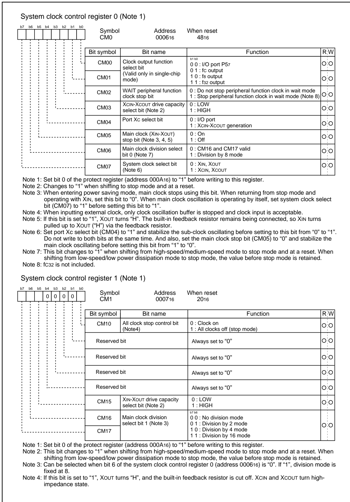
Figure 2.14.4. Power control-related registers
