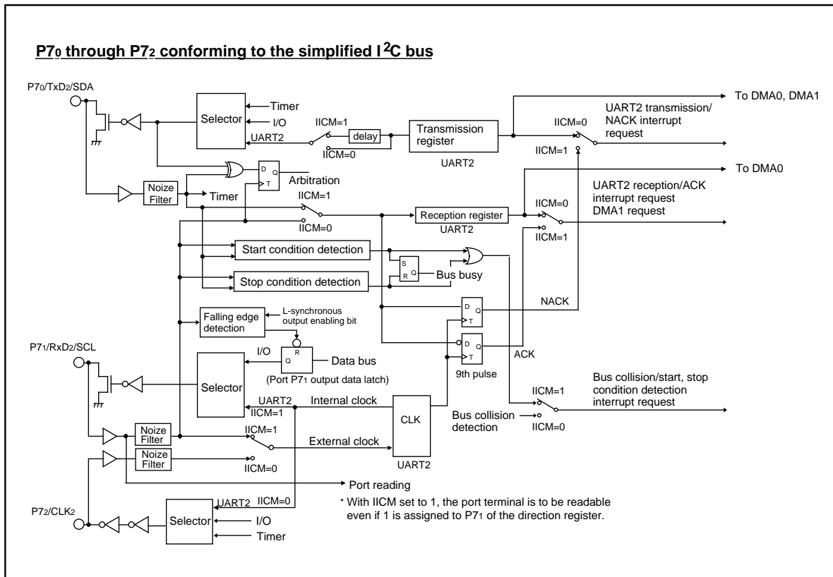
Figure 1.19.27. Functional block diagram for I 2 C mode
