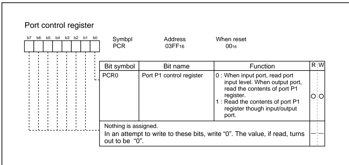
Figure 1.23.9. Port control register
