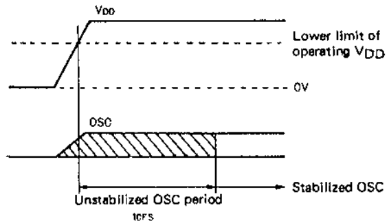
Fig. 5 Oscillation Stabilizing Period
