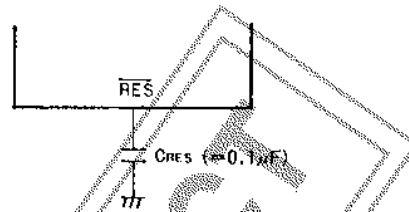
Fig. 6 Reset Circuit
