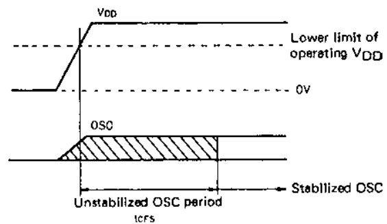
Fig. 3 Oscillation Stabilizing Period
