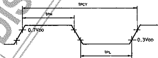
Fig. 6 Pulse Output Timing at Port PEQ
