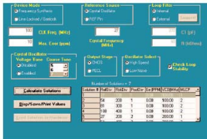
Figure 20: Frequency Synthesizer Screen
