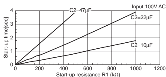
Fig. 5 Start-up time
