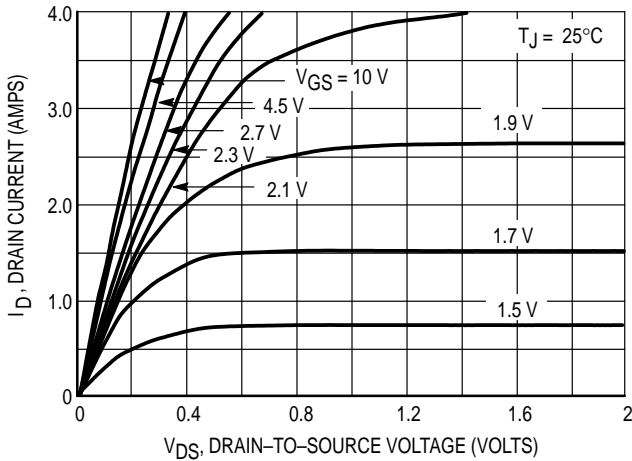
Figure 3. On-Region Characteristics
