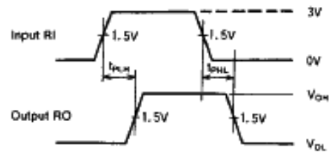
Receiver Section
