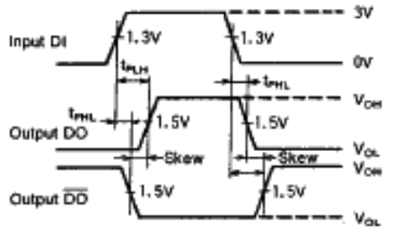
Driver Section
