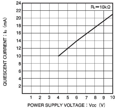
Fig. 3 Quiescent curve vs. power supply voltage
