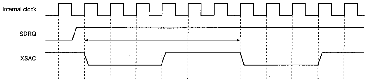
XFRATE [1:0] = 1
