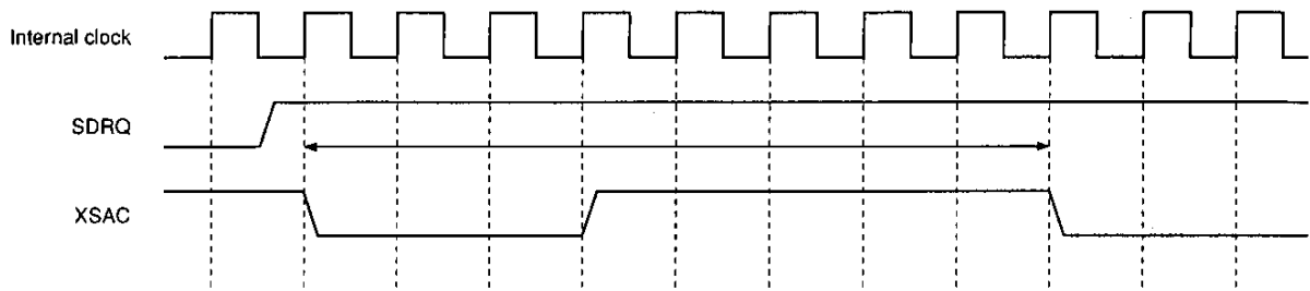
XFRATE [1:0] = 3
