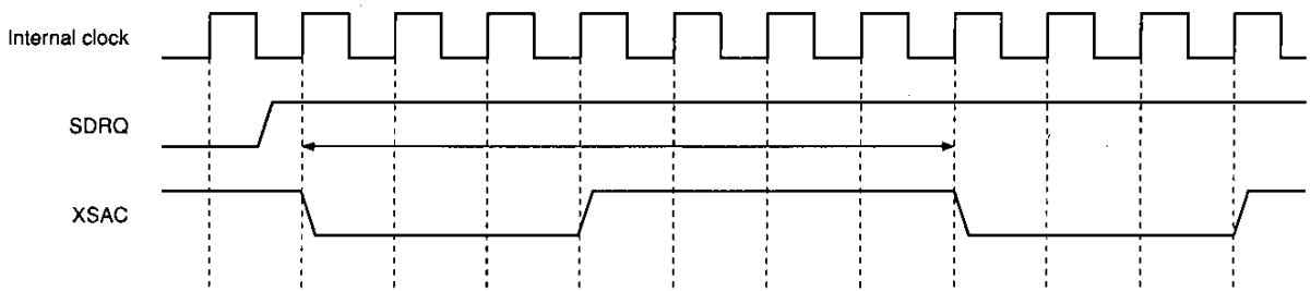
XFRATE [1:0] = 2
