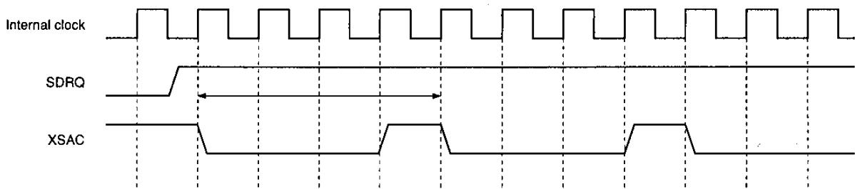
XFRATE [1:0] = 1
