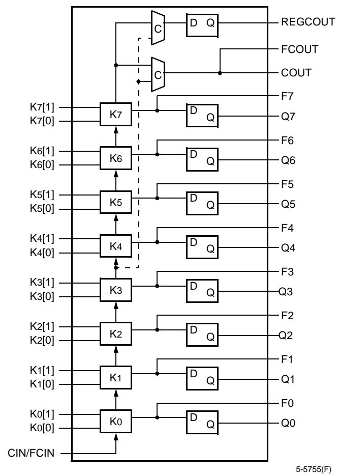
Figure 6. Ripple Mode
