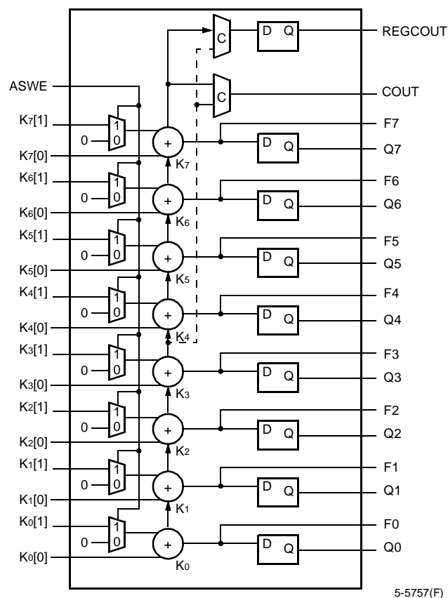
Figure 8. Multiplier Submode
