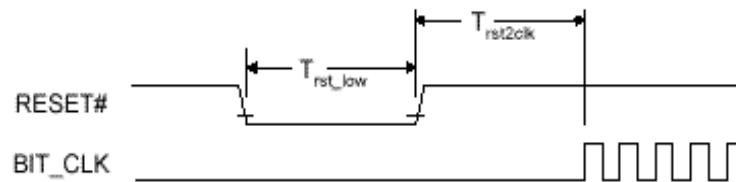
Fig 6.2.1-1 Cold reset timing diagram
