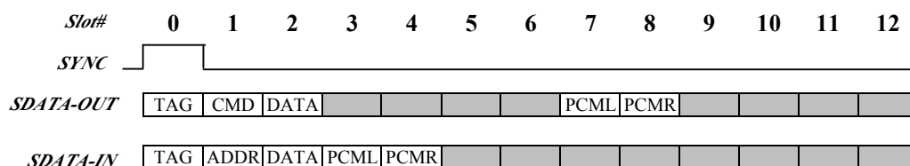
Fig5.2-2 ALC100 slot arrangement – CODEC ID = 10
