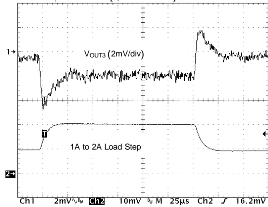
Fig.5 Transient Response of Linear Controller
