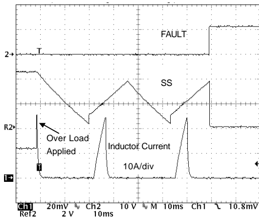
Fig.2 Over-Current Operation on Inductor
