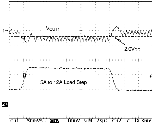
Fig.4 Transient Response of PWM Output
