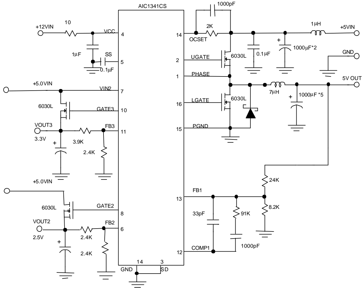
Circuit 1 Multiple Voltage Power application Circuit
