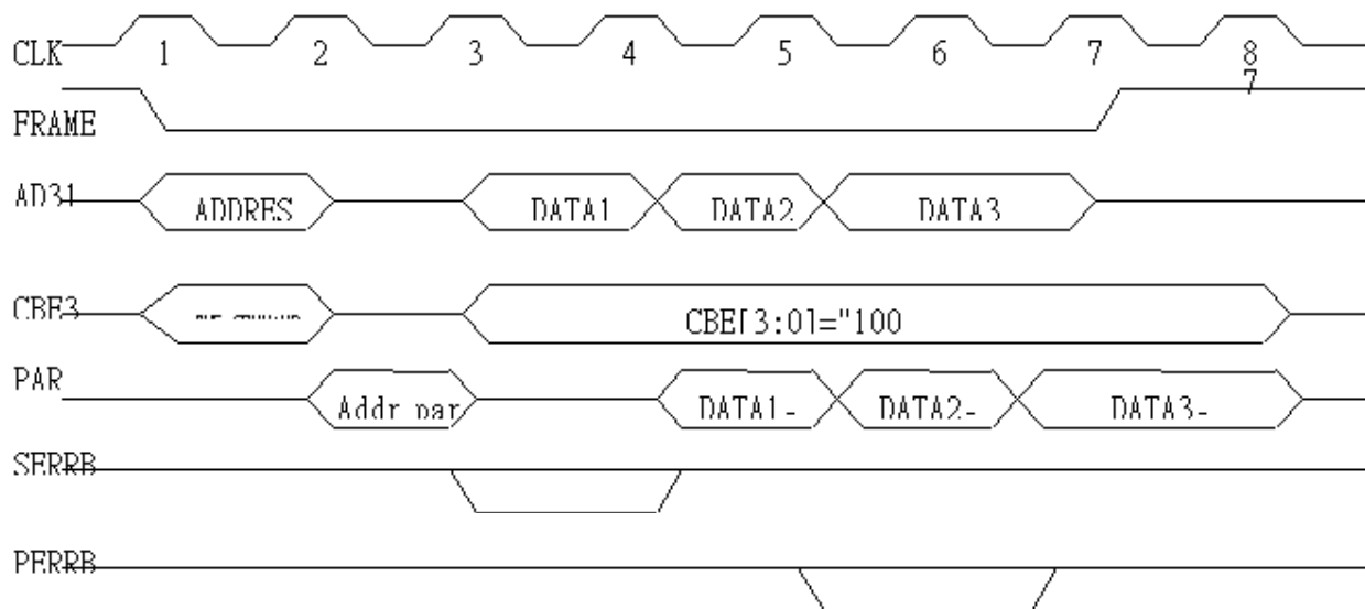
Figure 17. Parity Operation - One Example
