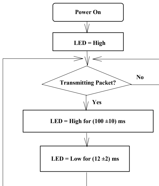
Figure 4. LED_TX
