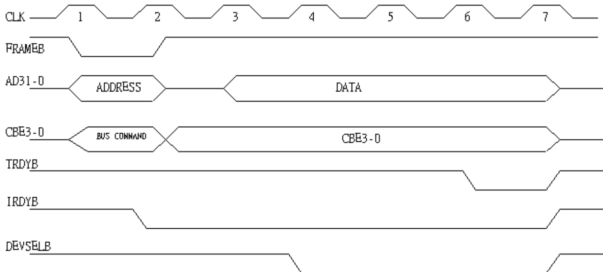
Figure 6. Target Read
