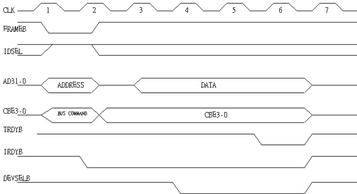
Figure 8. Configuration Read
