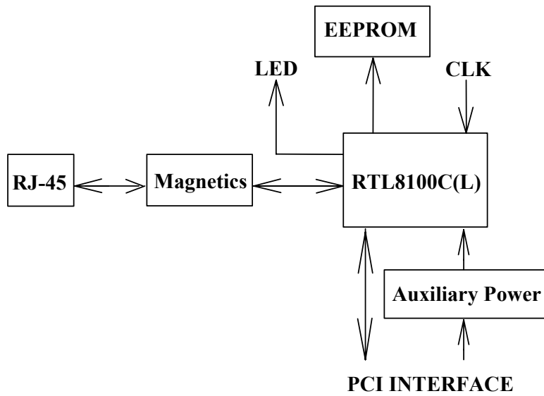
Figure 18. Application Information
