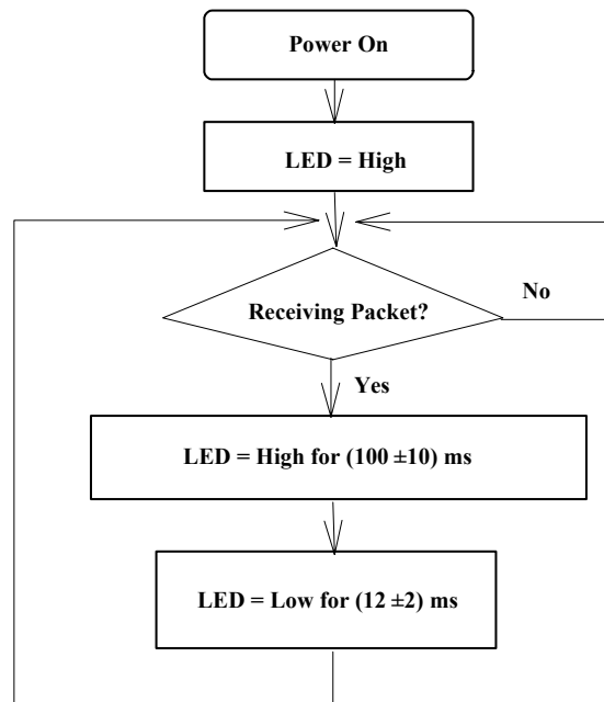
Figure 3. LED_RX
