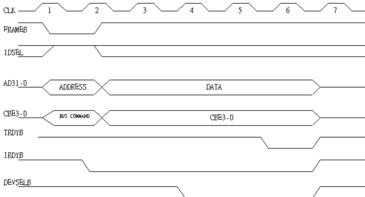
Figure 9. Configuration Write
