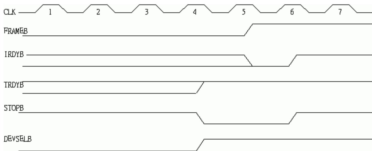
Figure 15. Target Initiated Termination - Abort
