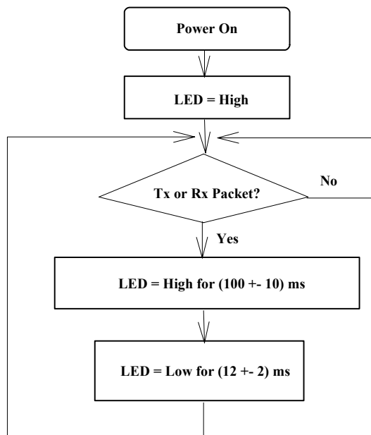
Figure 5. LED_TX+LED_RX
