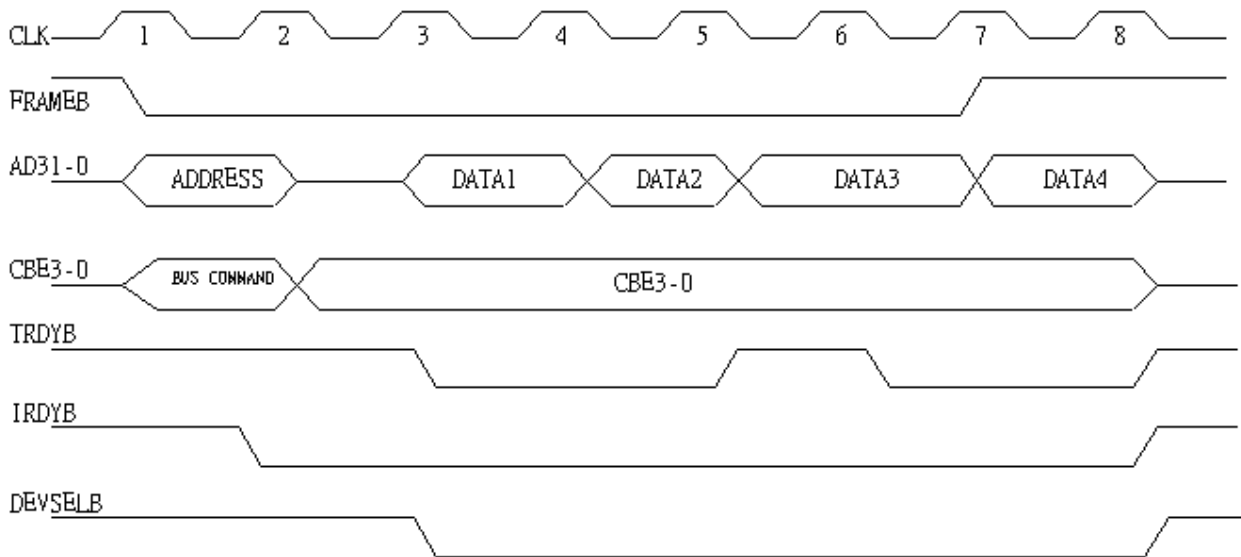
Figure 11. Memory Read
