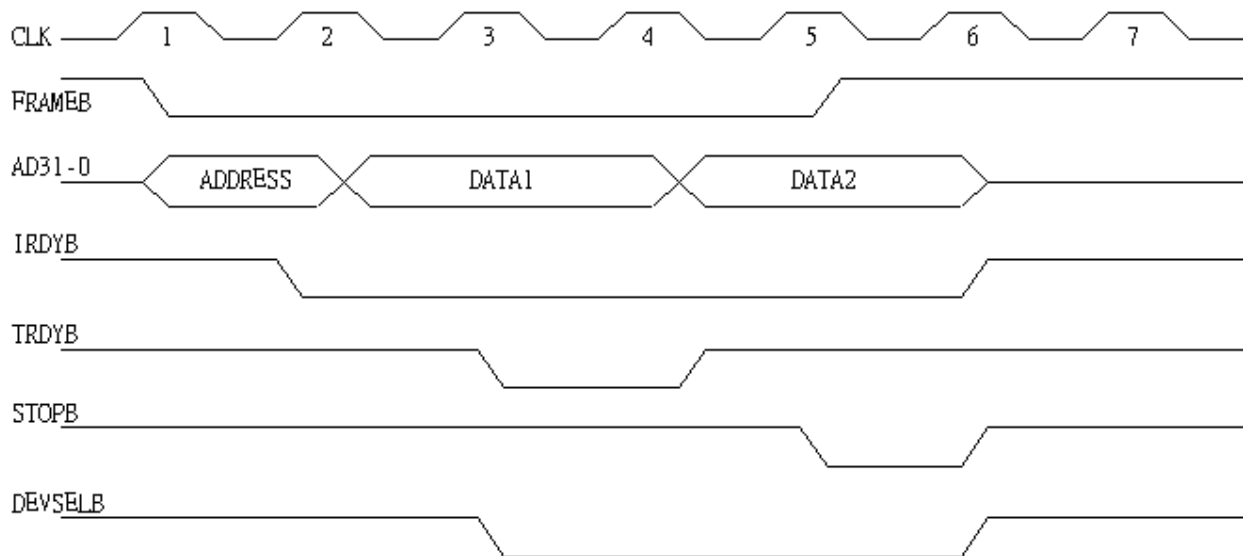
Figure 13. Target Initiated Termination - Retry
