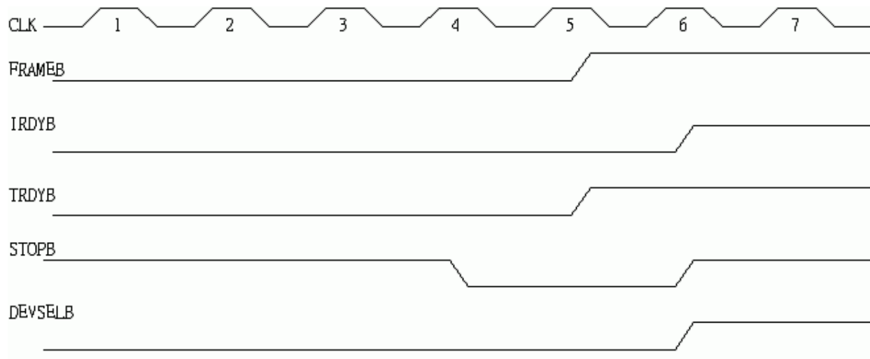
Figure 14. Target Initiated Termination - Disconnect
