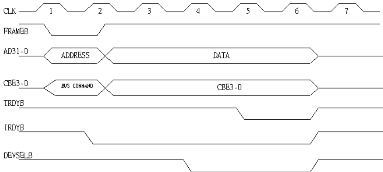
Figure 7. Target Write
