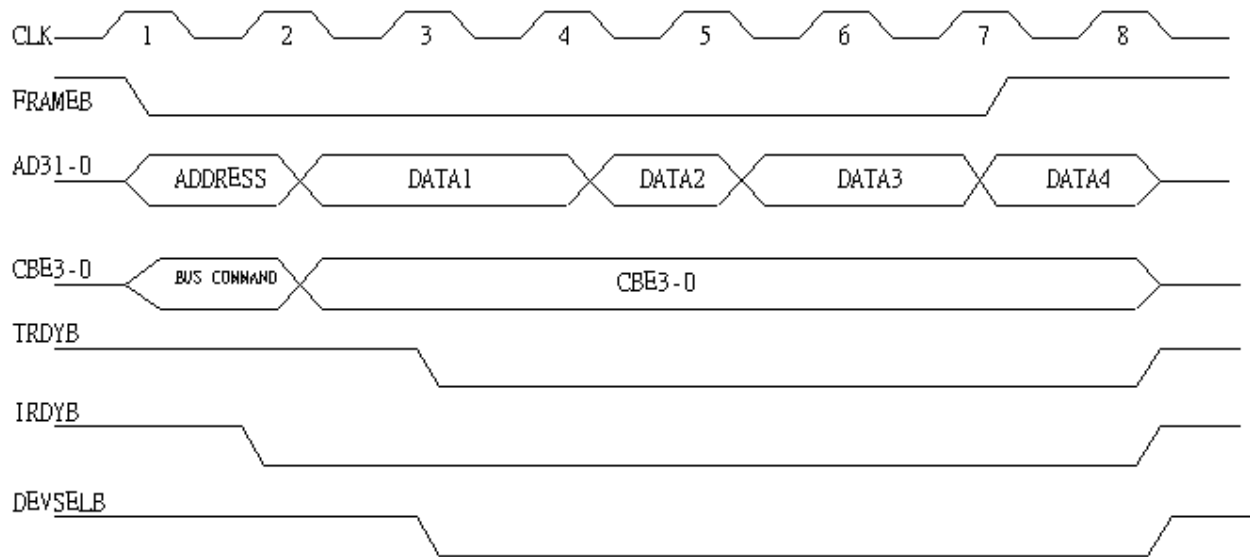
Figure 12. Memory Write
