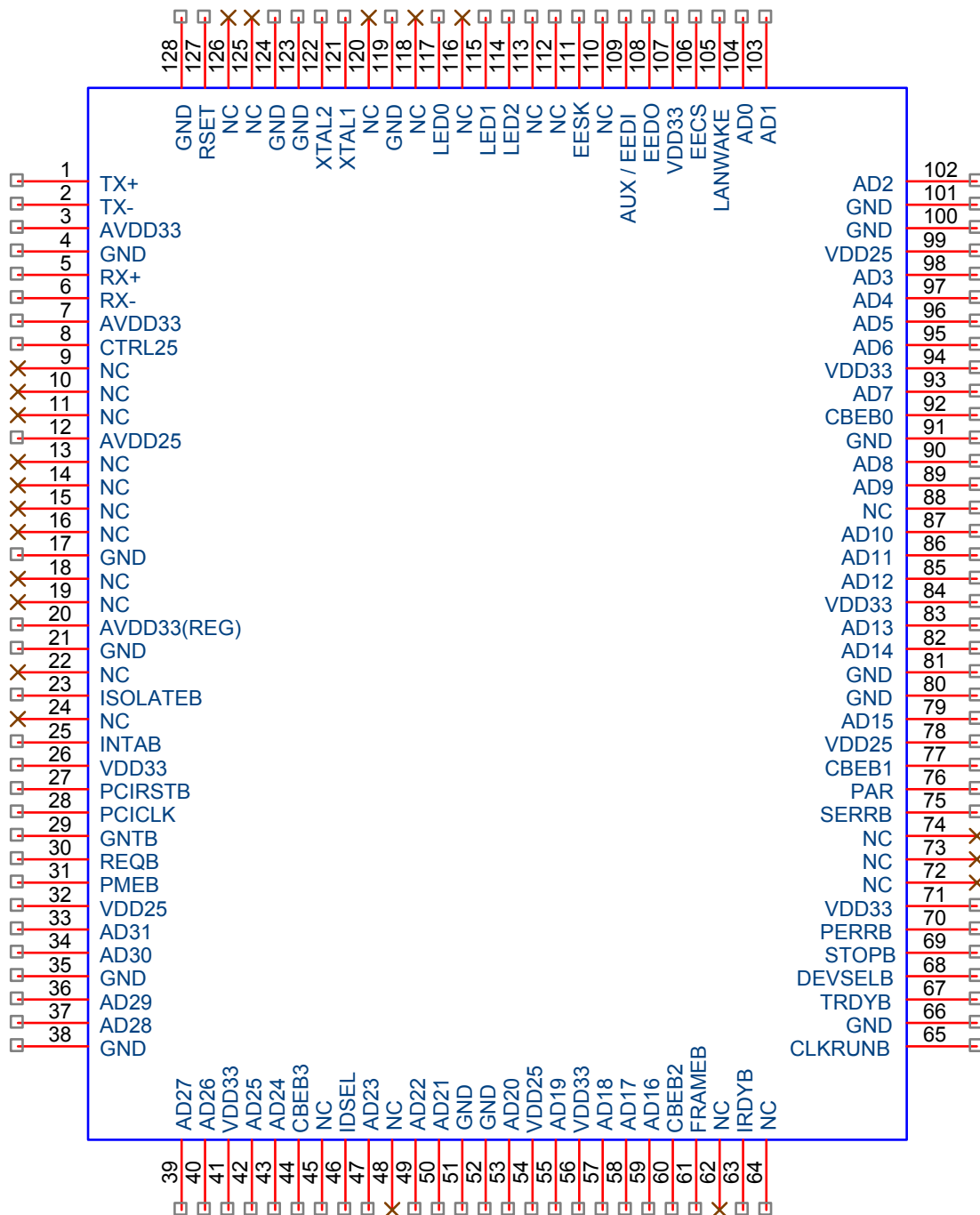
Figure 2. Pin Assignments
