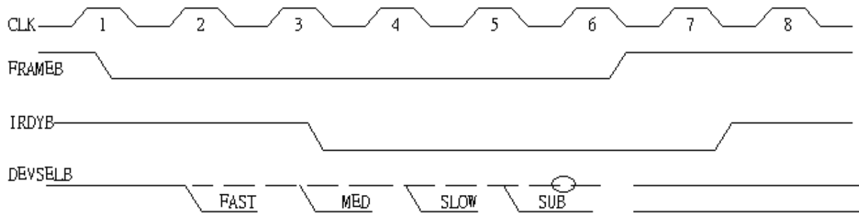
Figure 16. Master Initiated Termination – Abort
