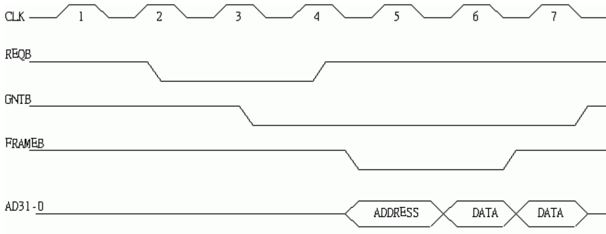
Figure 10. Bus Arbitration
