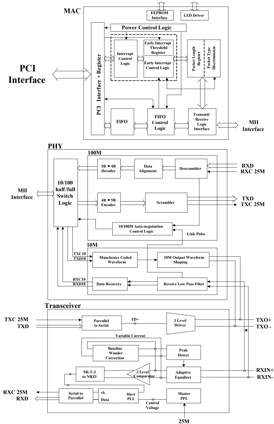
Figure 1. Block Diagram
