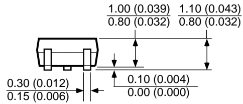
SC-70-5 (C5)
