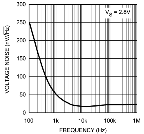
Voltage Noise
