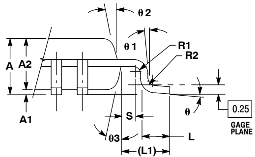
DETAIL F
