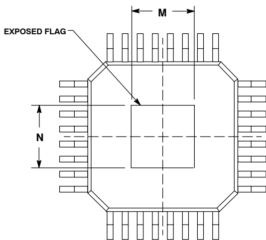
VIEW J-J
