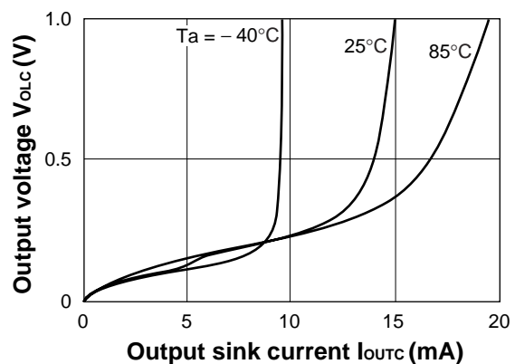
Output voltage ( V_{OLC} ) vs. output current
