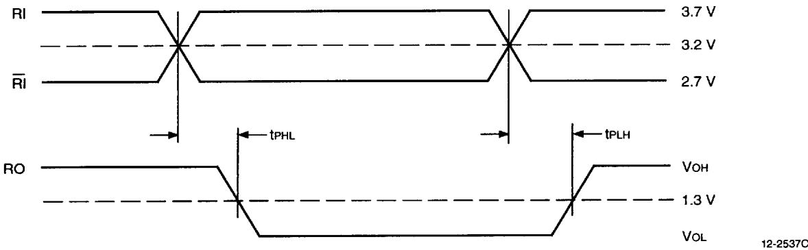
Figure 3. Receiver Propagation Delay Timing
