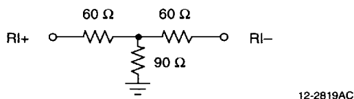
Figure 7. Built-In Y Termination Resistor
