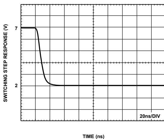
Figure 17. Data Switching Step Response (Falling Edge), 5 V Step, C_L = 200 pF, INV = LOW
