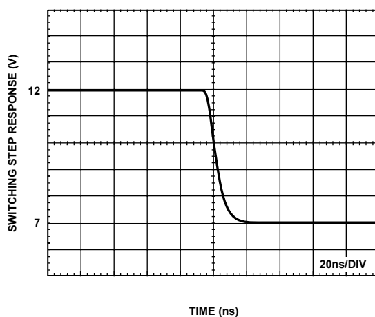
Figure 18. Data Switching Step Response (Falling Edge), 5 V Step, C_L = 200 pF, INV = HIGH
