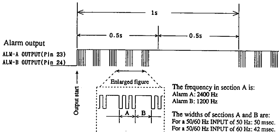
Figure 12 Alarm Output Waveforms
