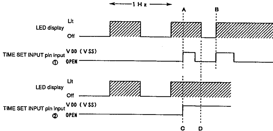
Figure 11 Clearing the Initial Input State Flashing
