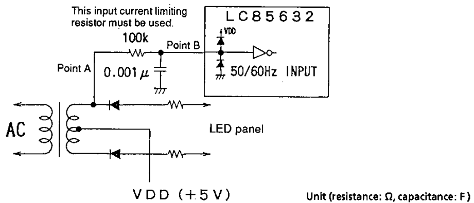
Figure 21 Recommended Circuit for AC Waveform Input
