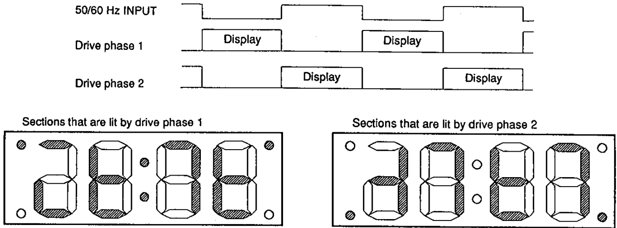
Figure 2 LED Sections Lit by the Drive Phases
