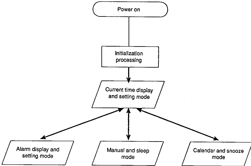
Figure 6 Operating State Transitions 1: Overall
