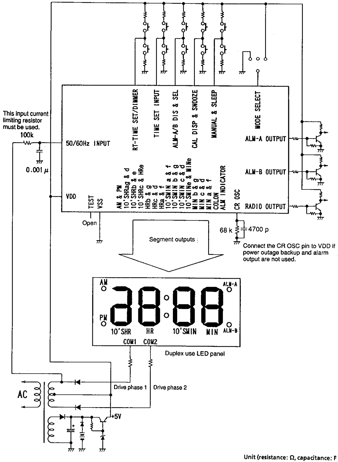
Figure 24 LC85632 Application Circuit
