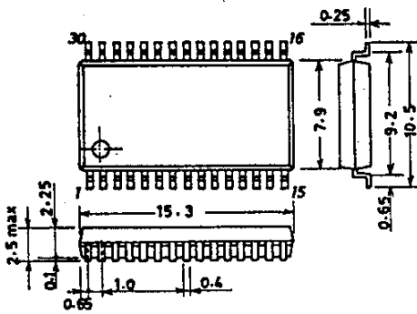
SANYO : MFP30S
