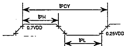
Fig. 7 Pulse Output Timing at Port PE0
