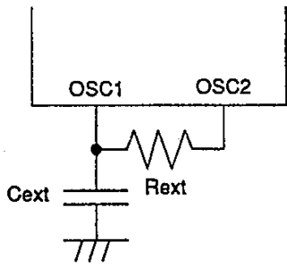
Fig. 2 2-pin RC Oscillation Circuit
