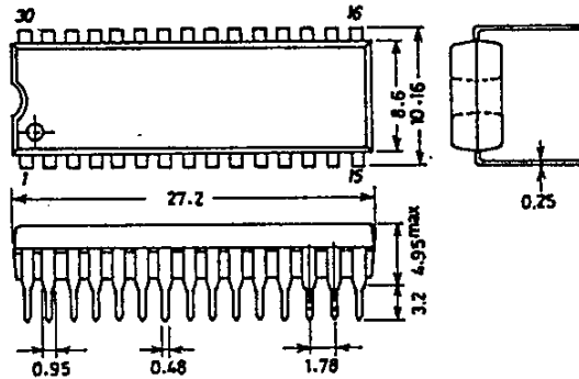
SANYO : DIP30S
