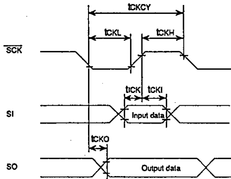
Fig. 6 Serial Input/Output Timing
