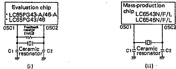
2-pin Ceramic Resonator Oscillation Circuit for Evaluation Chip and Mass-production Chip
