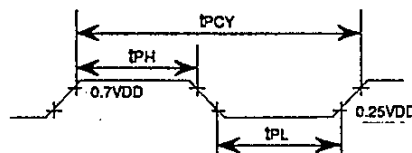
Fig.7 Pulse Output Timing at Port PE0
