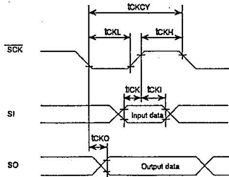
Fig. 5 Serial Input/Output Timing
