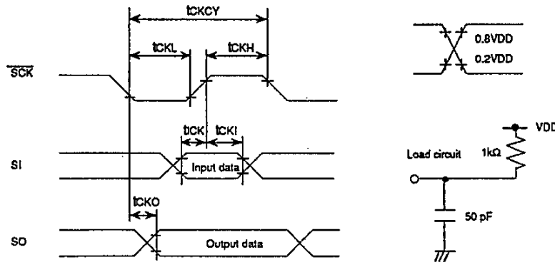
Fig. 6 Serial Input/Output Timing
