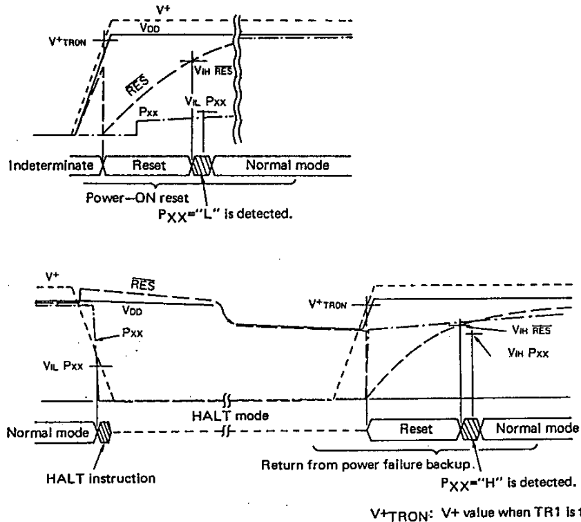
Fig. 2-4. Operating waveform in sample application circuit – (2)
