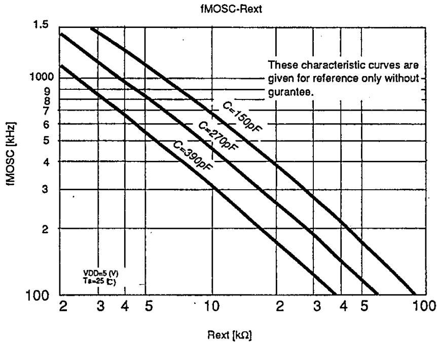
Fig. 8 RC Oscillation Frequency Data (Typ.)
