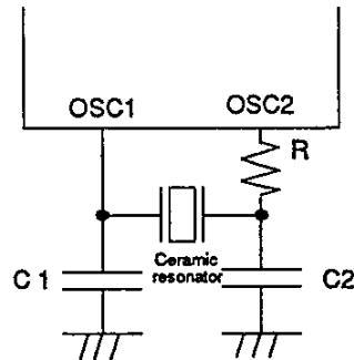
Fig. 3, Ceramic Resonator Oscillation Circuit
