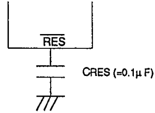
Fig. 5 Reset Circuit
