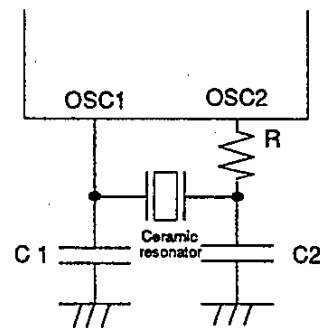
Fig. 3 Ceramic Resonator Oscillation Circuit
