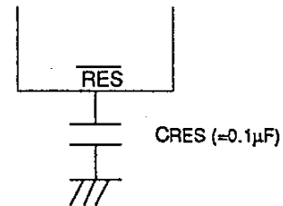
Fig. 4 Reset Circuit
