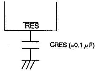
Fig. 5 Reset Circuit
