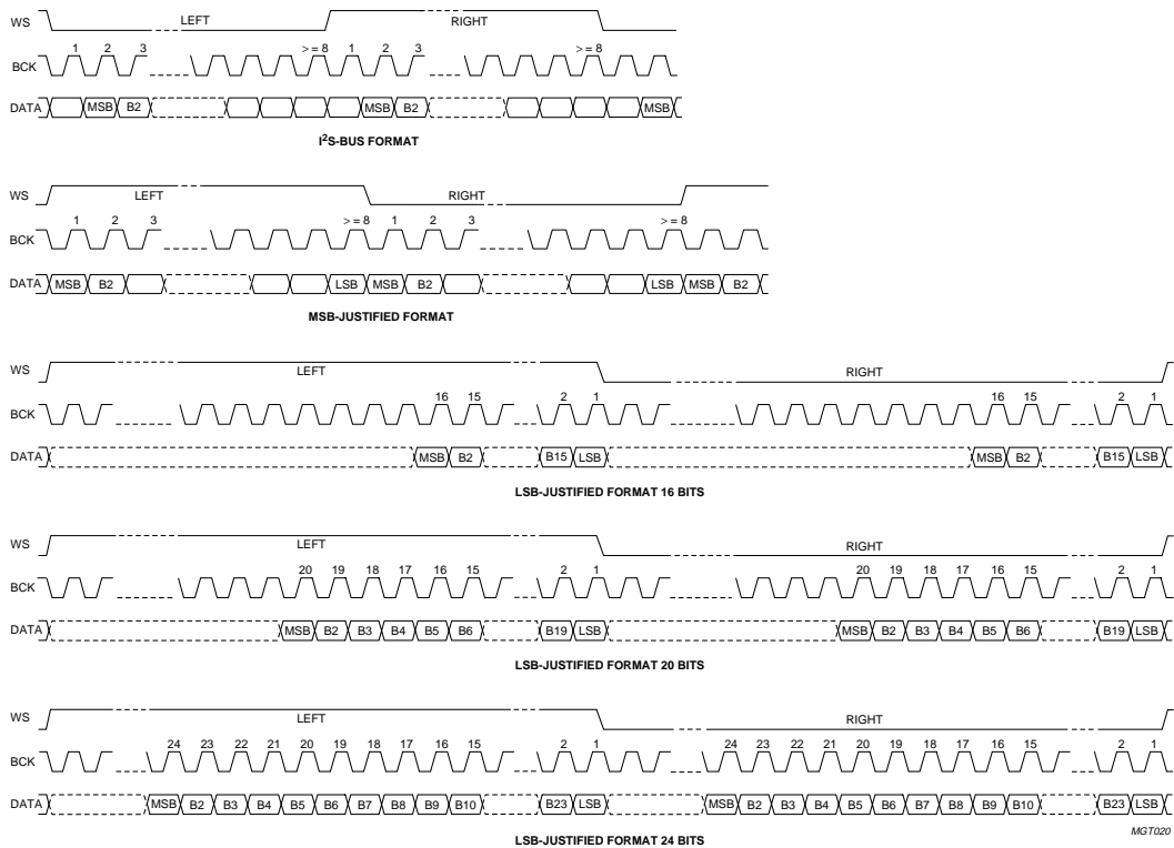
Fig.7 Formats of input and output data (single-channel).
