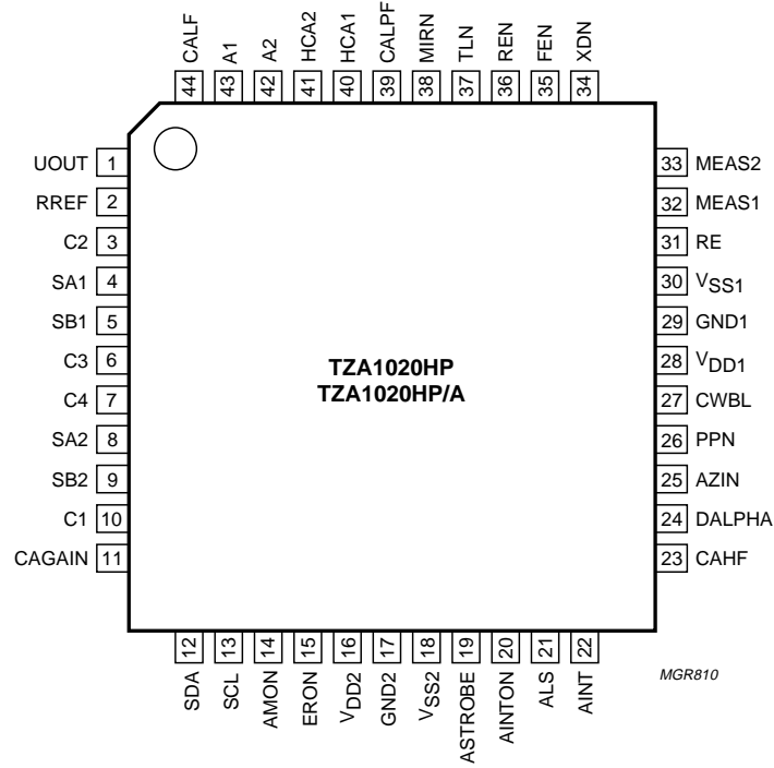
Fig.2 Pin configuration.
