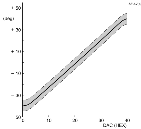
Fig.4 Hue control curve.
