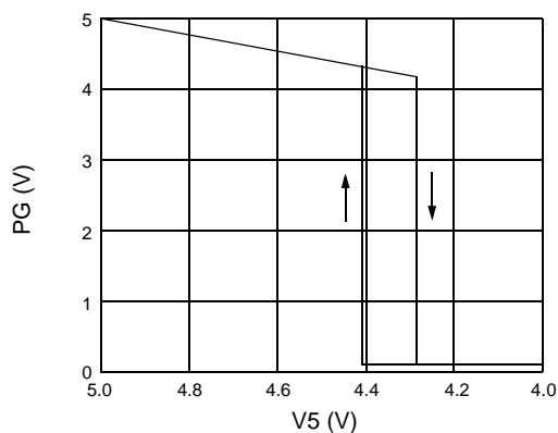
Figure 15. Detecting V5 Voltage for PG
