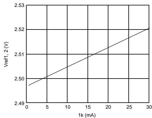
Figure 2. Vref1,2 Current Stability
