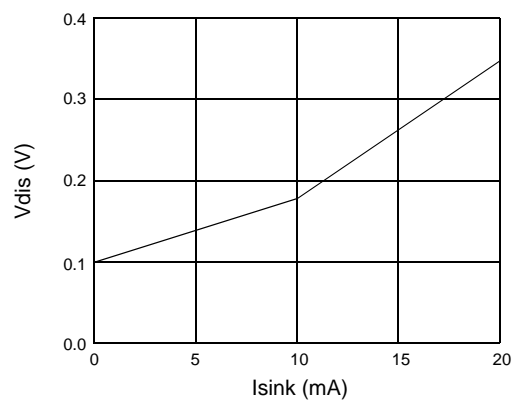
Figure 18. Disable Saturation Voltage
