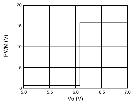
Figure 4. OCP Offset Voltage for 3.3V
