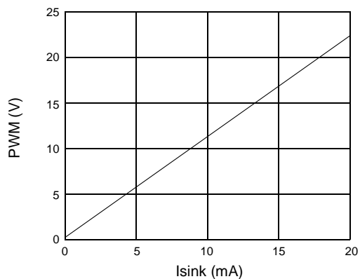
Figure 13. PWM Saturation Voltage
