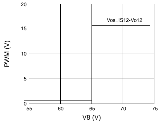
Figure 10. OCP Offset Voltage for 12V
