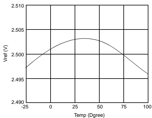
Figure 1. Temperature Stability for Vref1,2
