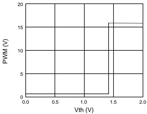
Figure 11. Remotr On/Off Input Threshold
