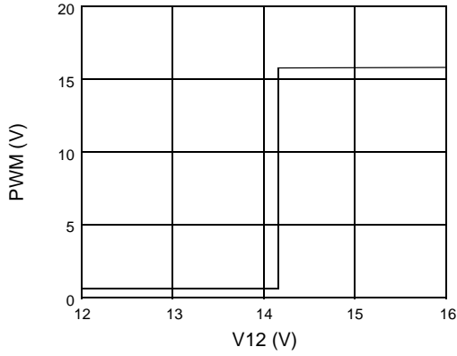
Figure 7. Over Voltage Protection for +12V
