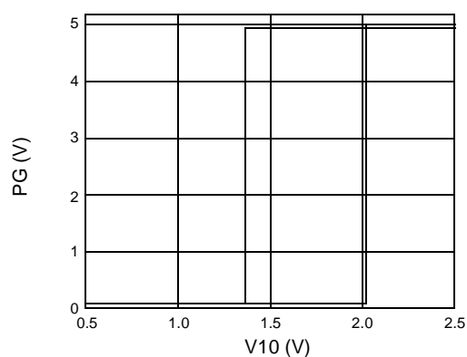
Figure 16. High/low Threshold Voltage of Comp9
