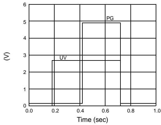
Figure 21. PG Delay
