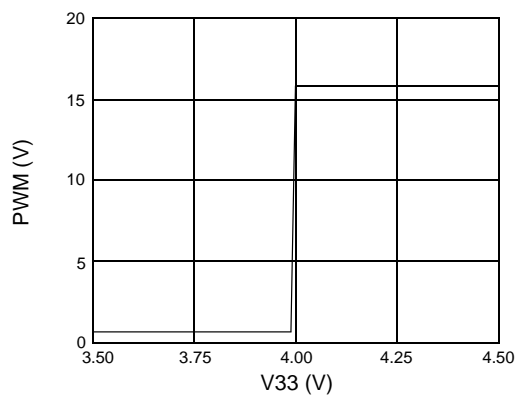
Figure 3. Over Voltage Protection for +3.3V
