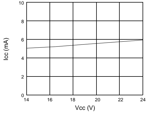
Figure 19. Supply Current of Vcc
