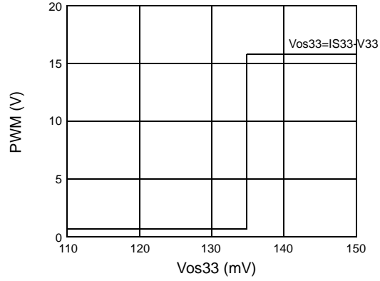
Figure 8. OCP Offset Voltage for 3.3V
