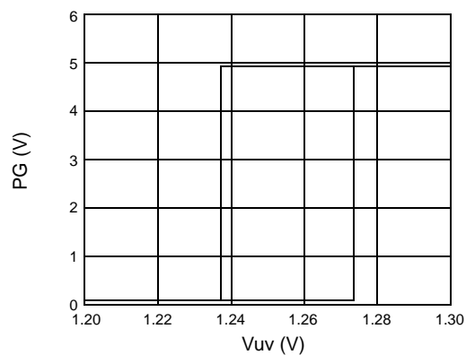
Figure 14. Detecting UV Voltage
