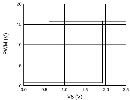
Figure 12. ON/OFF Delay Threshold Voltage
