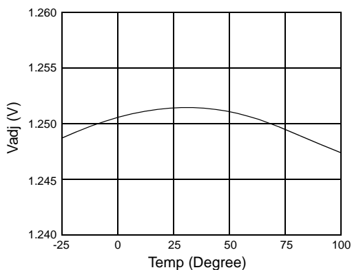
Figure 3. Bandgap Voltage (Vadj)
