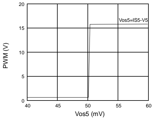
Figure 9. OCP Offset Voltage for 5V
