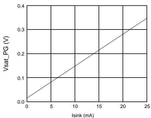
Figure 17. PG Saturating Voltage
