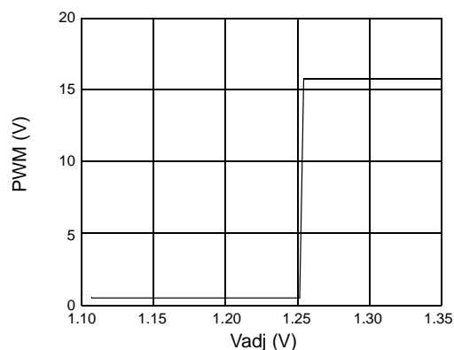
Figure 4. OVP Input Threshold Voltage for Adj
