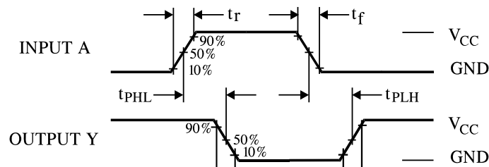
Figure 1. Switching Waveforms
