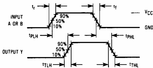
Figure 1. Switching Waveforms
