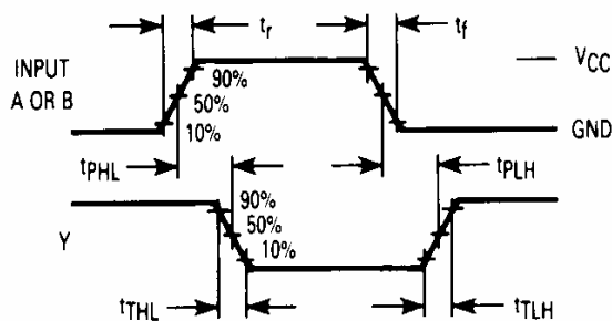
Figure 1. Switching Waveforms
