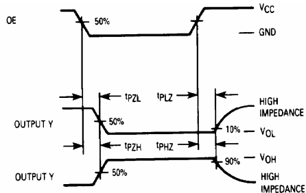
Figure 2. Switching Waveforms
