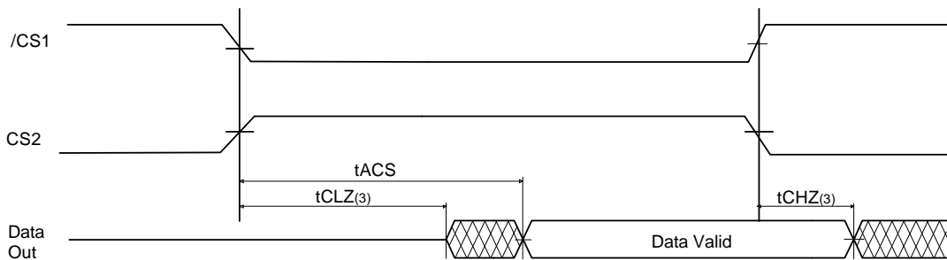
READ CYCLE 3(Note 1,2,4)
