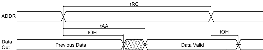
READ CYCLE 2(Note 1,2,4)
