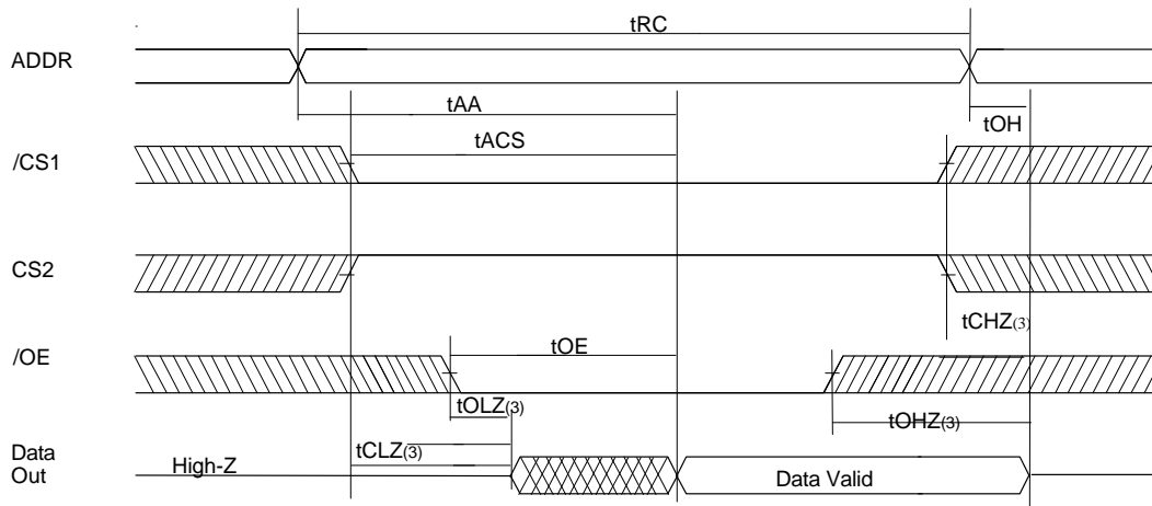
READ CYCLE 1(Note 1,4)
