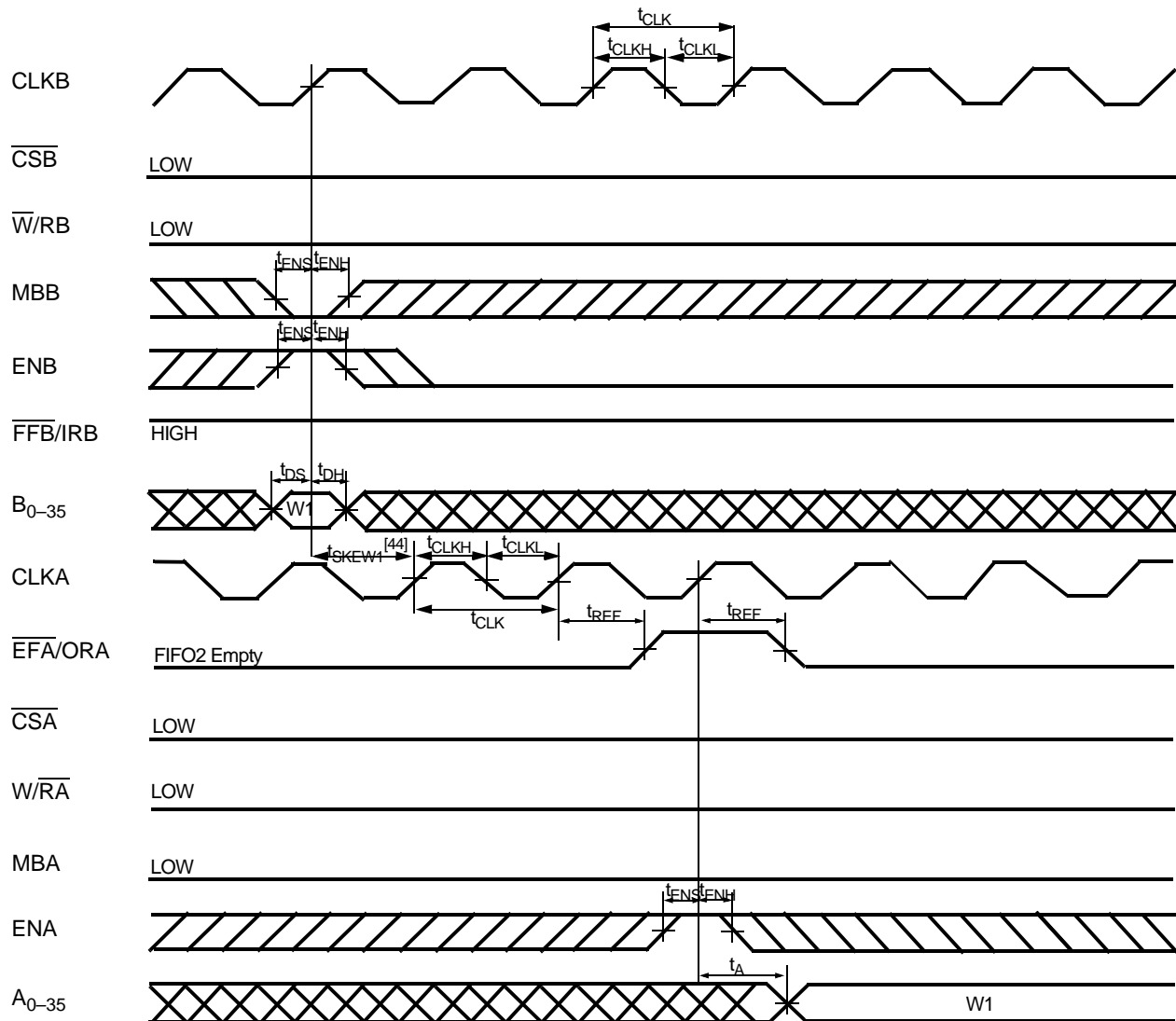
EFA Flag Timing and First Data Read when FIFO2 is Empty (CY Standard Mode) [42]
