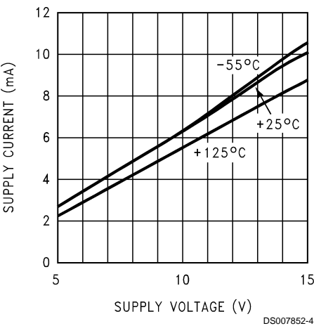
Supply Current vs. Supply Voltage (Each Section)
