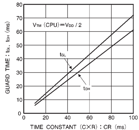
Fig. 11 Guard time vs. constant ( C \times R )
