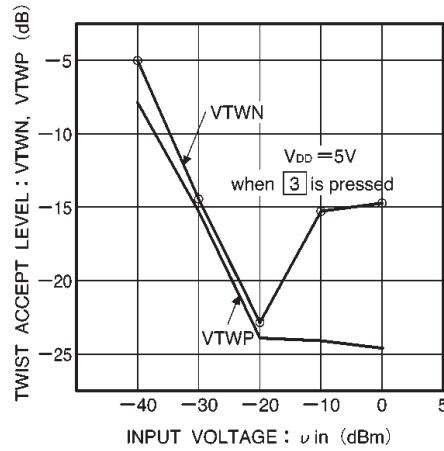
Fig. 17 2-frequency level vs. input voltage
