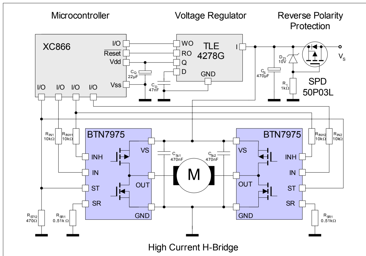
Figure 14 Application Example: H-Bridge with two BTN7975B
