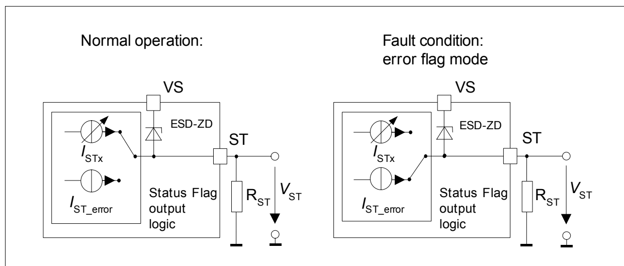
Figure 12 Status Flag Current
