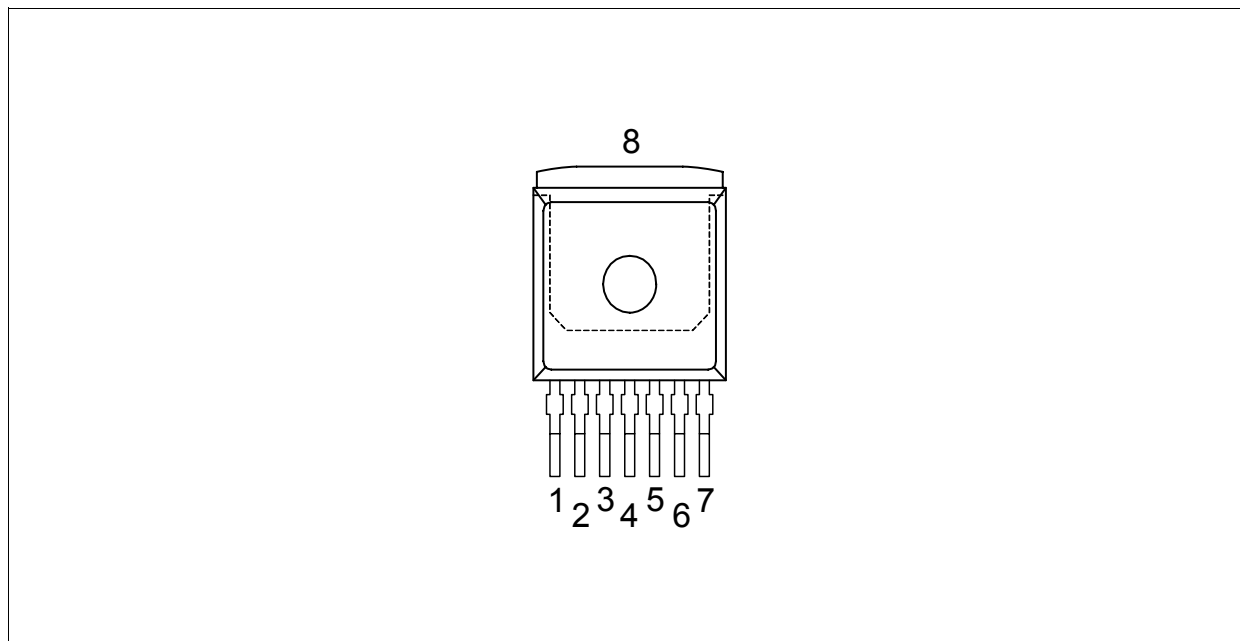
Figure 3 Pin Assignment BTN7975B (top view)
