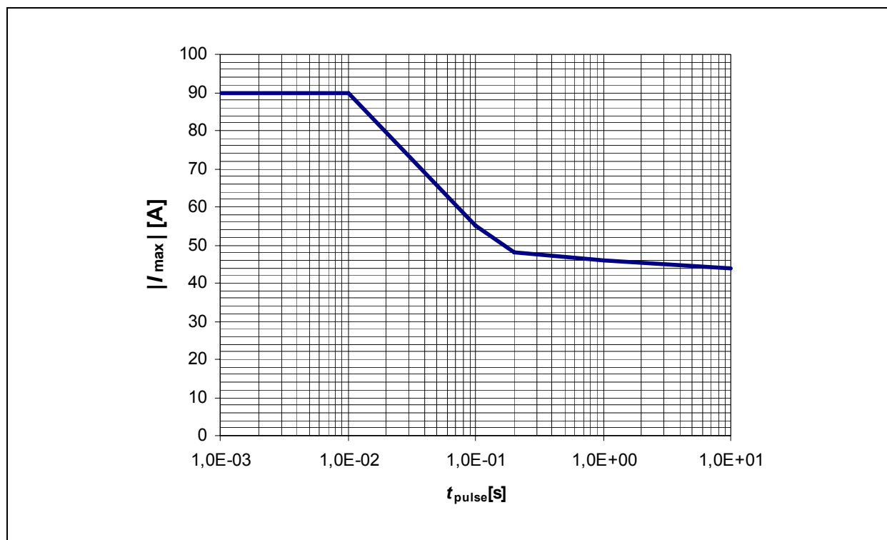
Figure 4 BTN7975B Maximum Single Pulse Current ( T_c < 85^\circ\text{C} )
