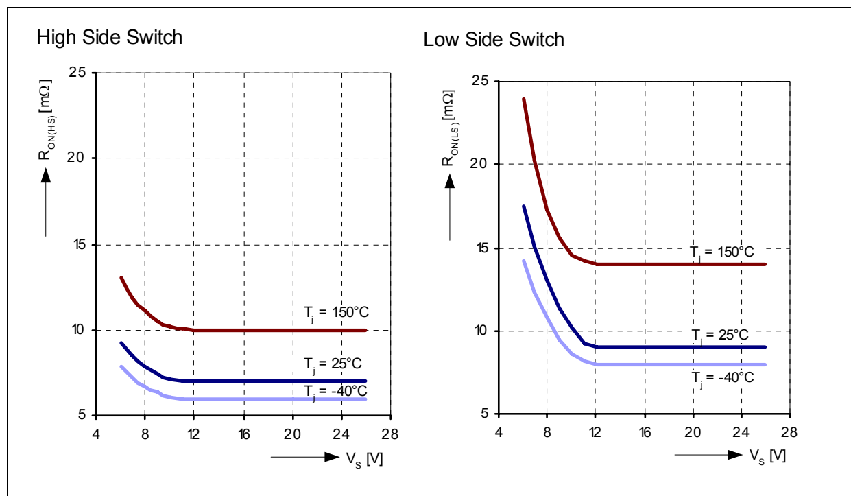
Figure 6 Typical ON State Resistance vs. Supply Voltage
