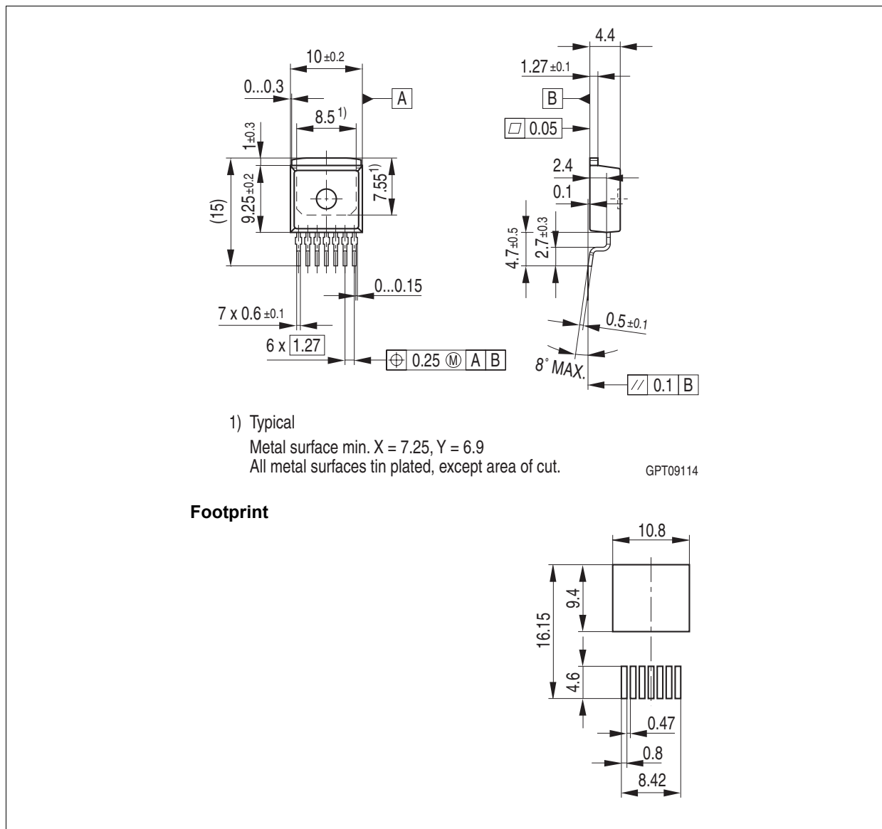
Figure 16 PG-T0263-7-1 (Plastic Green Transistor Single Outline Package)
