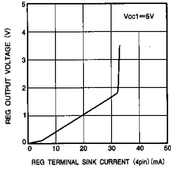
Fig.22 REG-pin output voltage vs. REG-pin sink current
