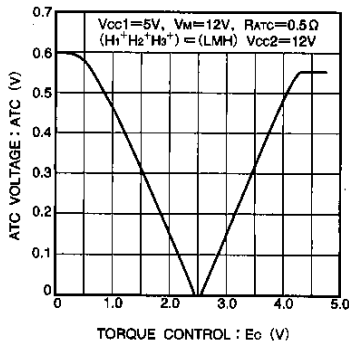
Fig.15 Output voltage vs. Torque control voltage ( I )
