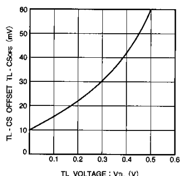
Fig.20 TL-CS offset vs. VTL voltage
