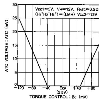
Fig.17 Output voltage vs. Torque control voltage ( III )
