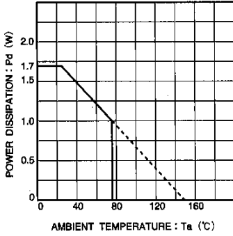
Fig.24 Power dissipation curve
