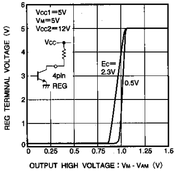
Fig.21 REG-pin voltage vs. High level output voltage
