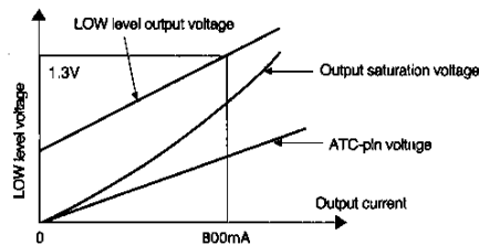
Fig.12 Low level output voltage vs. output current (reference curves)
