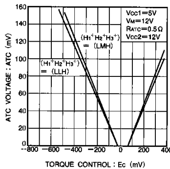
Fig.16 Output voltage vs. Torque control voltage ( II )
