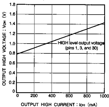
Fig.18 High level output voltage vs. High level output current
