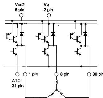
Fig.10 Output circuit
