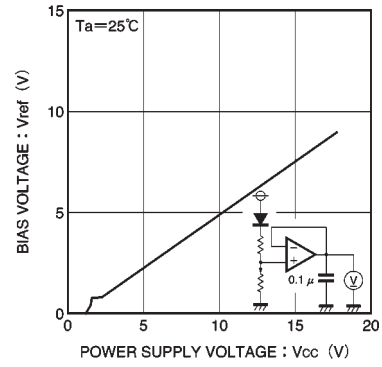
Fig. 3 Power supply voltage vs. bias pin voltage
