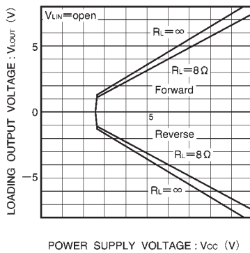
Fig. 15 Loading output vs. power supply voltage
