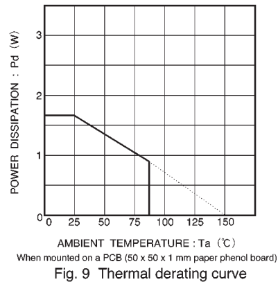
Fig. 9 Thermal derating curve
