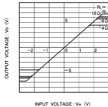
Fig. 11 Channel 1, 3 and 4 I/O characteristics (variable load)
