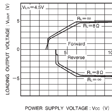
Fig. 14 Loading output vs. power supply voltage
