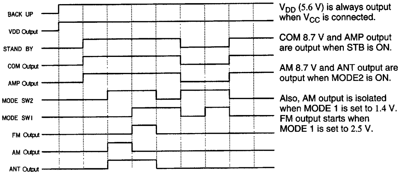
Figure 5 Timing chart
