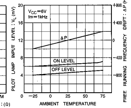
Fig. 10 Free running frequency drift and lamp on and off levels vs. ambient temperature
