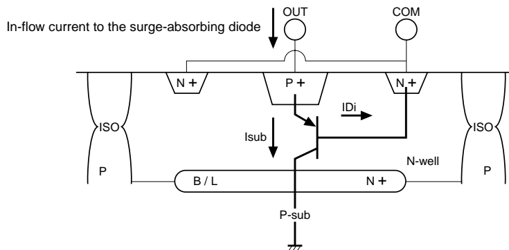
Fig.6 Vertical construction of the surge-absorbing diode
