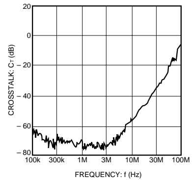
Fig. 4 Interchannel crosstalk
