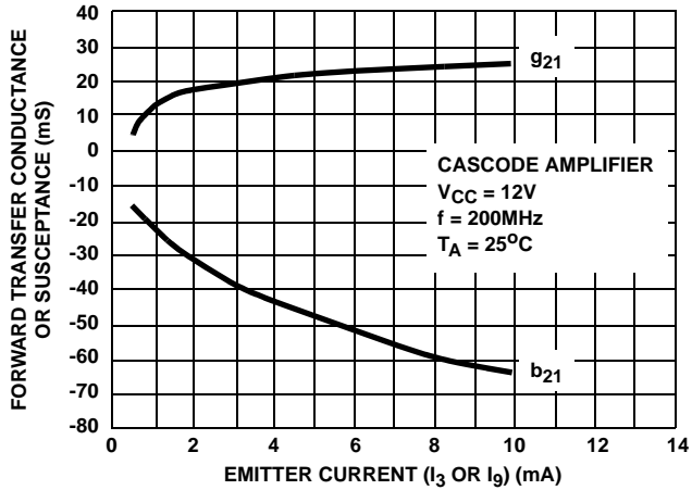
FIGURE 30. FORWARD TRANSFER ADMITTANCE ( Y_{21} ) vs EMITTER CURRENT
