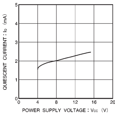
Fig.1 Quiescent current vs. power supply current
