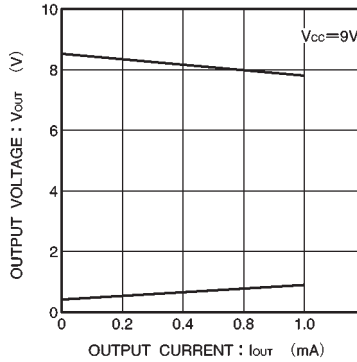
Fig.5 Hysteresis amplifier output voltage vs. output current
